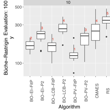
Fig. 2: Single-core BO vs. CMA-ES on the Büche-Rastrigin function. The notation refers to the different combination of acquisition function and kernel configuration. An experiment denoted as BO-PV-P2 then refers to BO using predicted value kernel with parameter p = 2 . The red number refers to the algorithm rank as determined by the pairwise multiple comparisons test.
