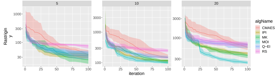
(a) Example of a separable multi-modal function
