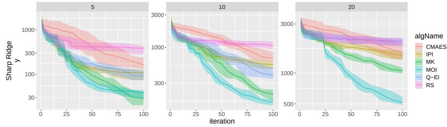
(b) Example of a unimodal function with high conditioning
