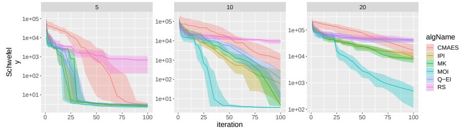
(c) Example of a multi-modal function with weak global structure
