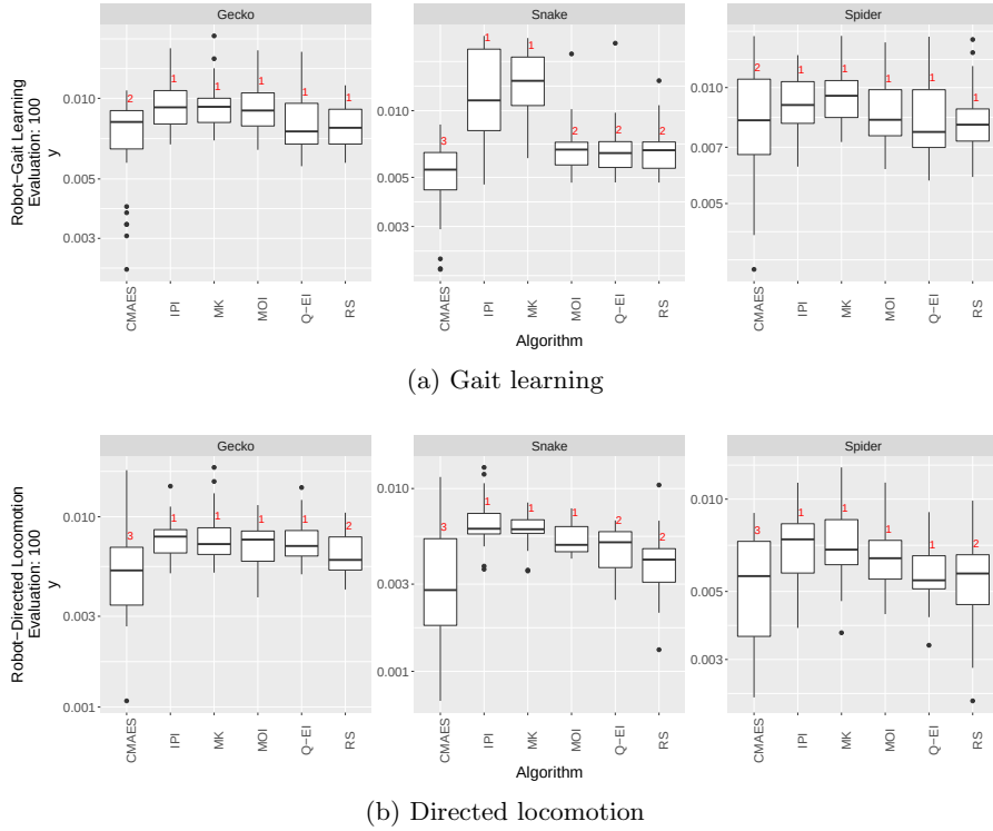
Fig. 4: Last iteration ranked multi-comparison test results for the robot application. The red number indicates the algorithm's achieved rank. BO methods maintain a better performance. However similar results by random search suggest BO is not able to efficiently exploit the optimization landscape.
