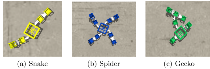
Fig. 1: Tested robot morphologies, each simulating an animal structure. The three different body components can be easily distinguished by shape and color. The biggest brick corresponds to the core component, each robot can only have one. Fixed bricks look similar but are smaller in size. Active hinges are illustrated in white.
