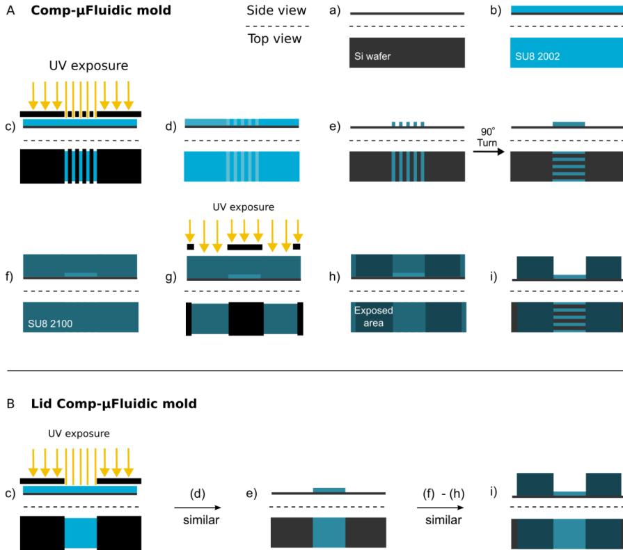
Figure 3.6 – SU-8 mold fabrication: (A) On the dehydrated silicon wafer (a), a first layer of SU8 2002 is spin-coated and UV-exposed using a photolithography technique (b-d). The unexposed area is removed in a development process (e), leaving the microchannel structures on the silicon wafer. A second layer of SU8-2100 or 2050 is spin-coated onto the sample (f), followed by UV exposure of the corresponding macrochannel areas (g-h). The final two-layer structure for microfluidic molding is obtained after development and curing (i). (B) The Lid Comp- \mu Fluidic molds are created in the same process with the use of different mask pattern: (c) depict the difference in UV-exposed area. (f-h) are the same steps with the different pattern, resulting in the (i) final Lid Comp- \mu Fluidic mold.
