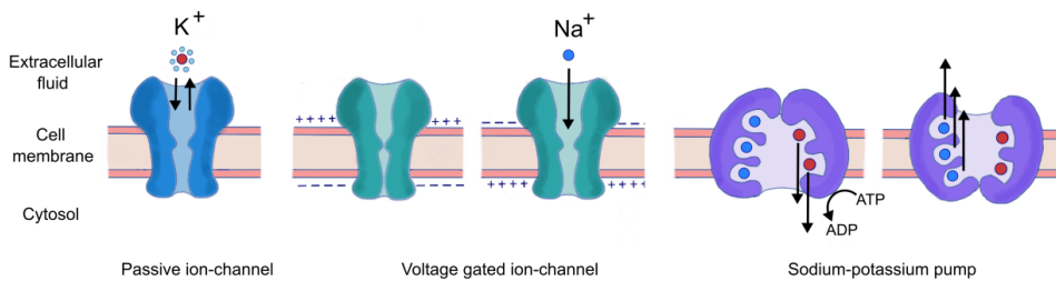
Figure 1.4 – Transmembrane proteins in charge of transferring ions across the cell membrane. The figure shows the most common ion channels and a pump responsible for the rest state of the membrane and action potential. Passive ion channels are highly selective and permeable to the specific hydrated ion. Voltage-gated ion channels are activated upon the change in membrane potential and present one of the crucial actors in the depolarization phase of an action potential. Sodium-potassium pump is an example of the active transport of these ions against the concentration gradient, intending to maintain the ionic concentration gradients that drive Na^+ and K^+ through their channels during the action potential. Figure adapted from Kandel et al. (2013b) and Bear et al. (2015c).
