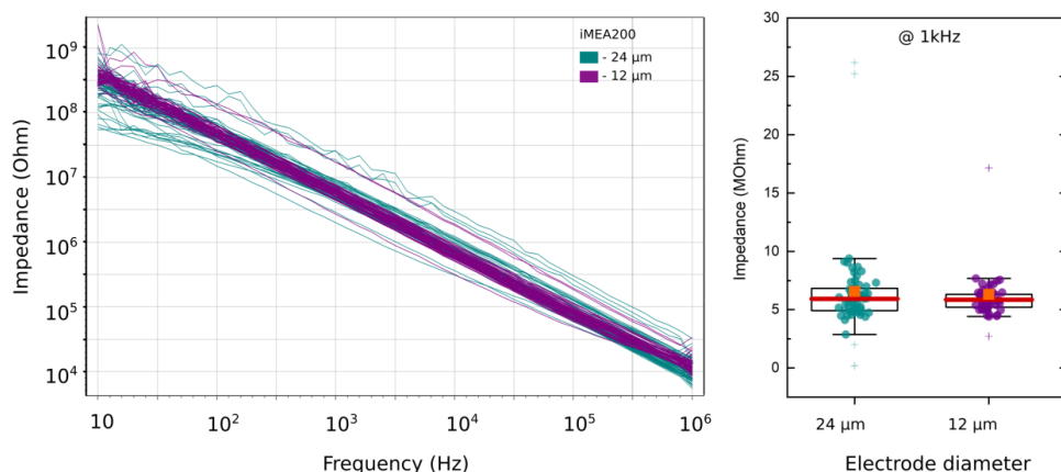
Figure 3.11 – EIS data of the iMEA200s of 24 (teal) and 12 (purple) \mu\text{m} electrode diameter. The bode impedance plot (left) presents scan frequencies from 10 Hz to 10^6 Hz. Presented are data sets from two MEAs with structured microchannels on top. Box plots present impedance values scanned at 1 kHz. Data points are plotted in teal (24 \mu\text{m} ) and purple (for 12 \mu\text{m} ) circles.
