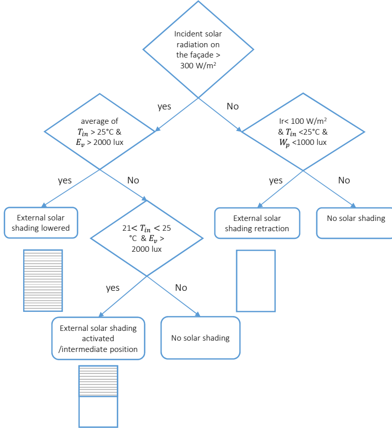
Figure 4.13: Flow chart of multi-objective control strategy.
