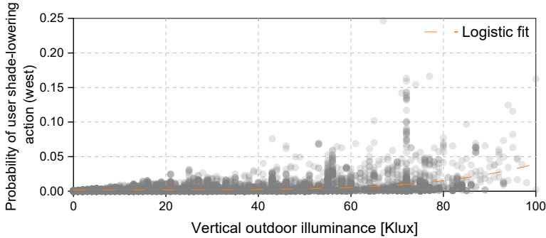
Figure 5.20: Probability of user-shade lowering action as a function of outdoor vertical illuminance on the west elevation.
