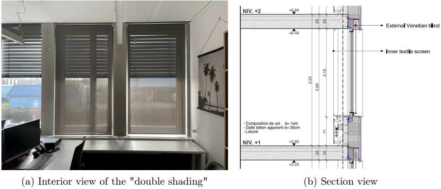
Figure 5.6: The double shading system approach 4
