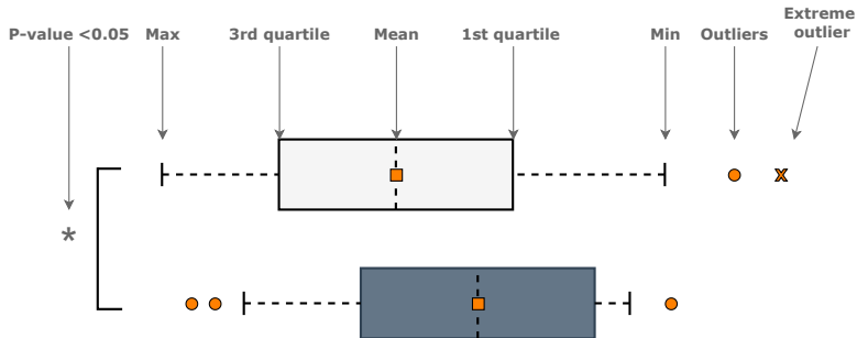
Figure 4.16: A statistical box-plot schematic diagram
