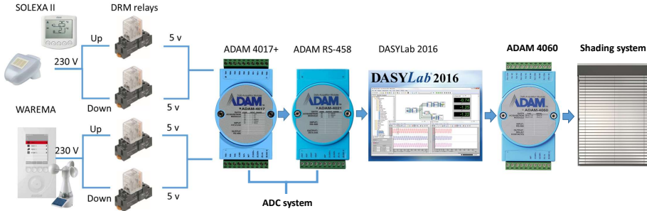
Figure 3.9: Electrical installation
