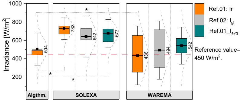
Figure 3.15: Setup 02 results:box-plot distribution of irradiance at the moment of shade lowering actions triggered by SOLEXA II and WAREMA, compared to simulation-based algorithm.
