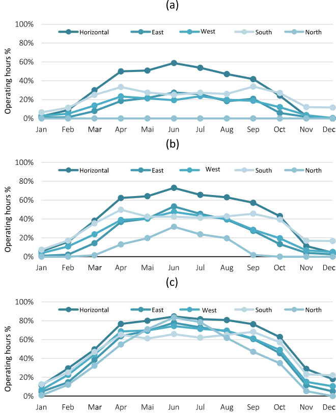
Figure 3.20: Monthly percentage of shade operating hours (closed) when irradiance threshold exceeded (a) 300 W/m 2 (b) 200 W/m 2 (c) 100 W/m 2
