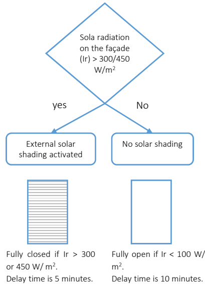
Figure 4.12: Flow chart of simple control strategy.
