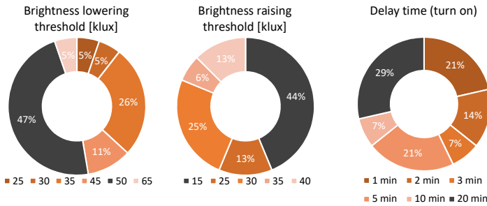
Figure 3.1: Brightness thresholds of shade operation (19 case studies).
