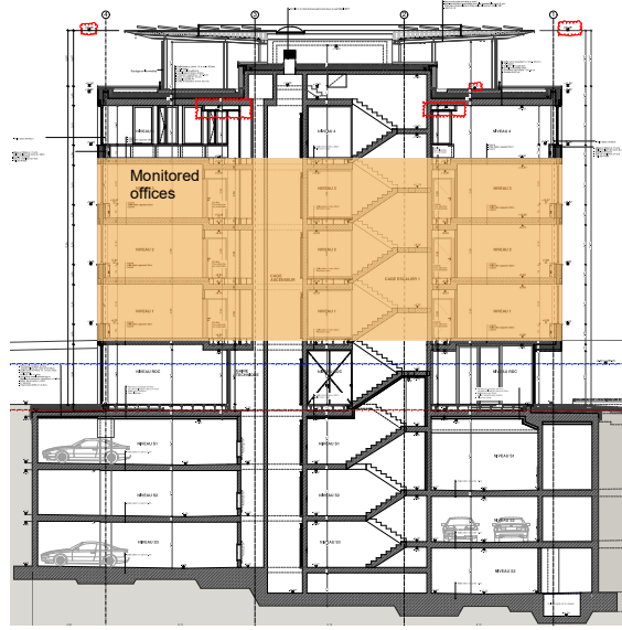
Figure 5.5: Section view of the building 3
