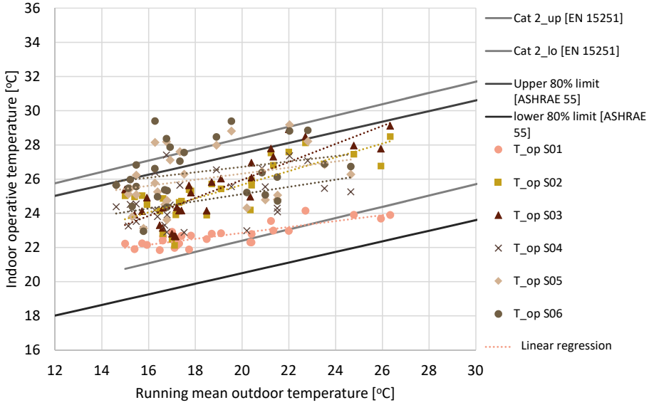
Figure 4.48: Acceptable operative temperature ranges from the adaptive comfort model included in ASHRAE 55 standards, 2017. The colored dots represent indoor operative temperatures registered for each scenario.
