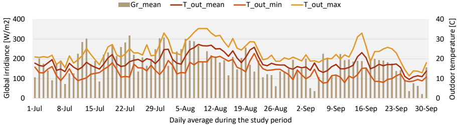
Figure 4.15: Daily average profile of max/ mean/ min outdoor temperatures and global horizontal radiation during the study period.
