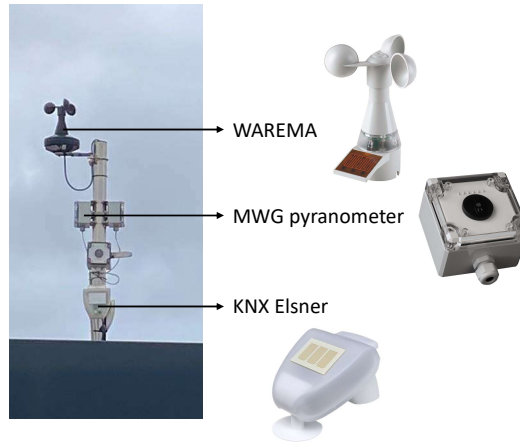
Figure 3.3: WAREMA, pyranometer, and KNX Elsner weather stations.
