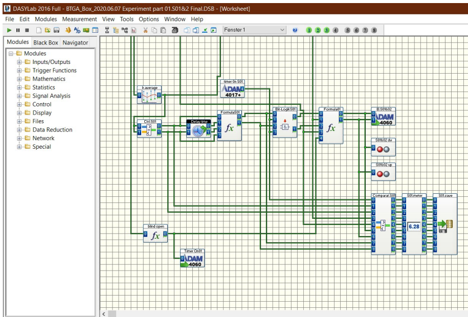
Figure 4.11: DASYLab worksheet of simple control strategy programming.
