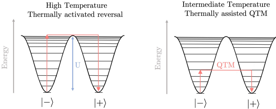
Figure 2.23: Visual representation depicting the mechanisms of magnetization reversal through thermal activation and thermally assisted quantum tunneling of magnetization.
