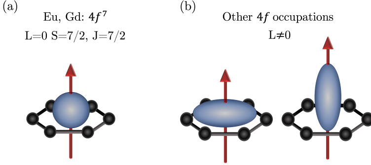
Figure 2.7: (a) In Eu and Gd the half-filled 4f -shell produces vanishing values of \mathbf{L} reflecting in a spherical shape of the 4f charge distribution. (b) For other 4f occupations, the total orbital angular momentum is non-zero leading to oblate or prolate-like geometries of the 4f cloud which interact differently with the surrounding CF based on their orientation.
