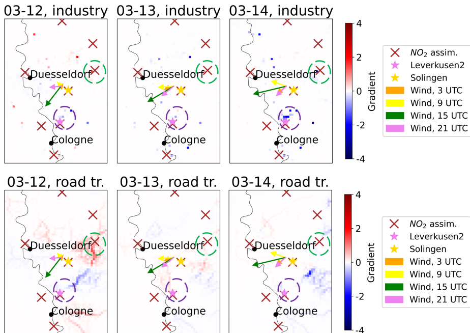
Figure B.15.: First iteration NO gradients of the industry and the road transport sectors from 12 March to 14 March. A part of the NRW domain with 51 \text{ km} \times 71 \text{ km} is shown. The wind directions at 3, 9, 15 and 21 UTC are displayed as arrows. The locations of the observation stations Leverkusen and Solingen are depicted as violet and gold stars, the locations of the other \text{NO}_2 assimilation stations as brown crosses, area 1 as a violet and area 2 as a green circle.
