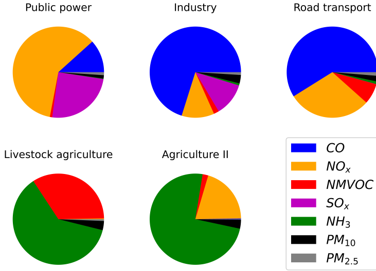
Figure 5.3.: Chemical composition of the emissions from the public power, industry, road transport and both agriculture sectors. The average chemical composition of the inventory emissions in the NRW domain for the year 2016 based on the inventory of the Copernicus Atmosphere Monitoring Service (CAMS) (Kuenen et al., 2018) and the GRETA tool (Schneider et al., 2016) of the Federal Environmental Agency (UBA) is depicted for each sector. Note that the chemical composition in the emission data is specific in each grid cell and thus may differ from the average values shown in this figure.
