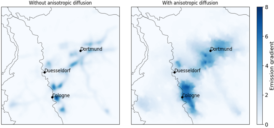
Figure 6.8.: Gradient with respect to the emission corrections for the road transport sector ( \nabla_{\mathbf{w}, \text{road}} J ) without (left) and with (right) anisotropic diffusion along roads (Section 4.3) in experiment I on 10 March 2016. The emission perturbation factors in the nature run of this experiment are 2 for the industry sector and 0.5 for the road transport sector.
