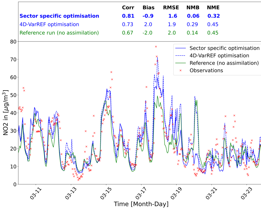
Figure 7.6.: Time series of \text{NO}_2 concentrations averaged over all validation stations. The observations are depicted as red crosses, the reference run without data assimilation as green solid line, the analysis of the sector specific optimisation as blue solid line and the analysis of the 4D-VarREF optimisation as blue dashed line. The correlation ("Corr"), the bias in \mu\text{g}/\text{m}^3 , the unbiased root mean squared error ("RMSE") in \mu\text{g}/\text{m}^3 , the normalised mean bias ("NMB") and the normalised mean error ("NME") - each with respect to the observations - are given for the time series of the three simulations.
