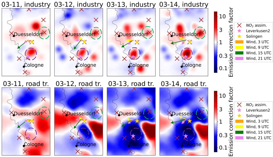
Figure B.13.: Emission correction factors of the industry and the road transport sector from 11 March to 14 March. A part of the NRW domain with 51 \text{ km} \times 71 \text{ km} is shown. The wind directions at 3, 9, 15 and 21 UTC are displayed as arrows. The locations of the observation stations in Leverkusen and Solingen are depicted as violet and gold stars, the locations of the other \text{NO}_2 assimilation stations as brown crosses, area 1 as a violet and area 2 as a green circle.
