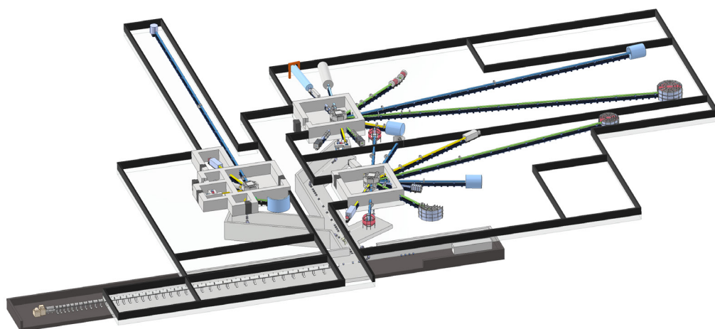
Figure III.1: General layout of the HBS facility
