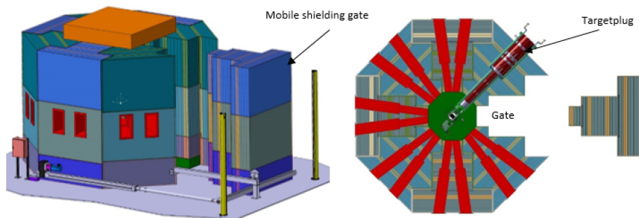
Figure III.2: Technical drawing of the shielding block in side view (left) and top view (right)
