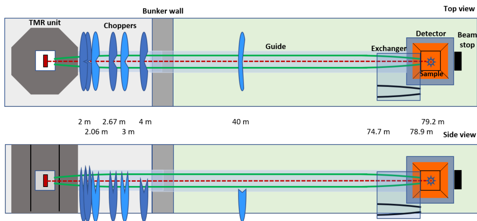
Figure V.2: Layout of the Thermal Powder Diffractometer (TPD).
