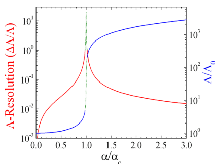
Figure V.30: Resolution scheme of the evanescent wave to study the structure in the normal direction. The scattering depth \Lambda (blue curve) switches between evanescent wave and damped wave. The derivative (red curve) determines the resolution of the depth-resolved GISANS measurement. The green dotted line indicate the forbidden range.
