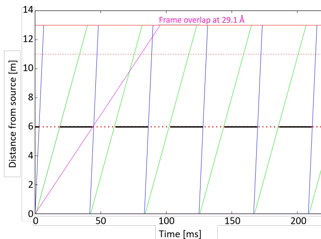
Figure V.40: Time-of-flight scheme of the reflectometer for off-specular scattering.
