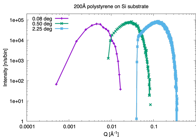
Figure V.42: Intensity impinging on a sample of 1 \text{ cm}^2 surface area at different angles of incidence. The binning size in Q is 10^{-3} \text{ Å}^{-1} .
