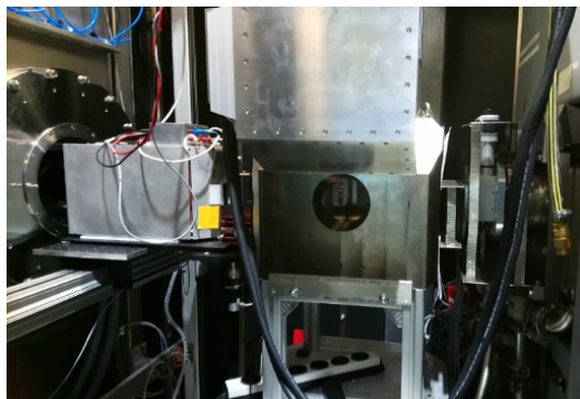
Figure V.28: The polarization analysis set-up (left) with a 3 T magnet (center) at the sample position of KWS-1, one SANS instrument at JCNS/MLZ in Garching.
