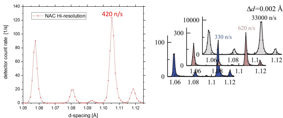
Figure V.8: Shapes and intensities of the intense lines between 1.05 and 1.12 Å of the NAC diffraction pattern obtained for the HBS diffractometer (left, red) in comparison with simulations on other sources: WISH at ISIS (blue), POWGEN at SNS (brown) and DREAM at ESS (grey). Figure on the right side taken from reference [SVL + 16]
