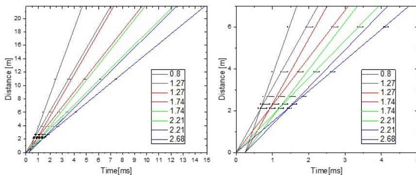
Figure V.19: Time Distance Diagram of the WFM set-up. On the left for the whole instrument length showing the 4 generated sub frames. On the right a closer look on the first 7 m of the instrument.
