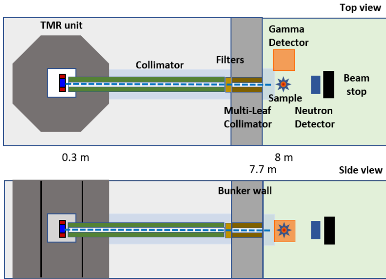
Figure VII.8: Schematic top and side view of the PGAINS instrument with fast neutrons.
