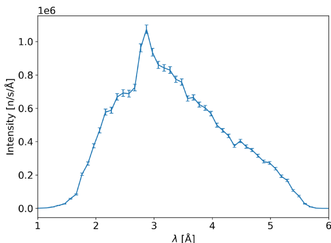
Figure V.37: Intensity on a 2x2 cm 2 sample with collimated mode under 1.9° incident angle with \frac{\Delta\theta}{\theta} = 10\% .
