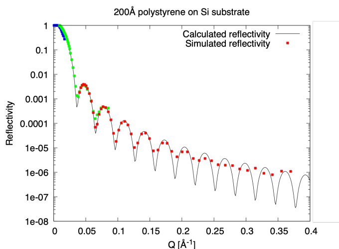
Figure V.43: Simulated reflectivity measurement of a 200 \text{ Å} thick polystyrene film on a Si wafer of 1 \text{ cm}^2 size. Three measurements at different angles of incidence have been simulated: 0.08^\circ (blue), 0.5^\circ (green), and 2.25^\circ (red). The 'calculated reflectivity' does not take the convolution with resolution into account.
