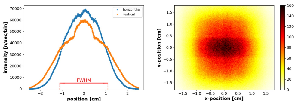
Figure V.24: Spatial distribution of the neutrons at the sample position for the high flux mode.
