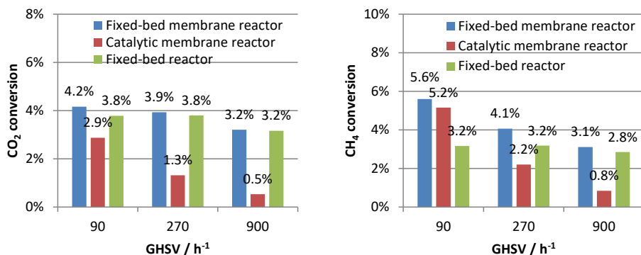
Fig. 6-16 CO 2 and CH 4 conversions at 450 °C and 20 bar with CH 4 :CO 2 = 1:2.
