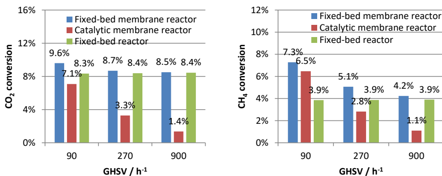
Fig. 6-17 CO 2 and CH 4 conversions at 500 °C and 20 bar with CO 2 :CH 4 = 1:1.
