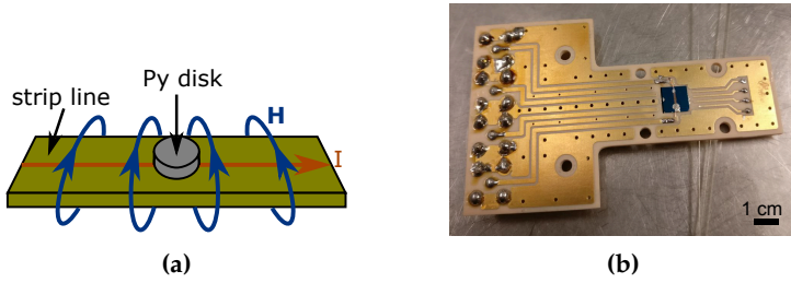
Figure 6.18.: Sample geometry used for STXM measurements. (a) Schematic diagram of the Py disk on a strip line, which generates an in-plane magnetic field H at the sample position when a current I is passed through. (b) Image of a sample on the chip stuck to a PCB board with silver paste. The strip line is also connected to the board with silver paste.
