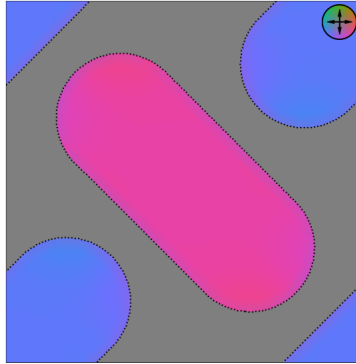
Figure 4.24.: Close up on a single particle from the micromagnetic simulation of the chiral ice pattern revealing parallel magnetisation along the long axis of the particle. Adapted from [117]
