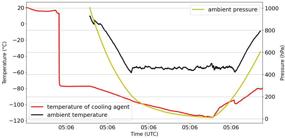
Figure B.2: Temperature of the new cooling agents during the flight on the 25 April 2020. The temperature of the ethanol-CO 2 mixture is given in red. The ambient temperature is given in black and the pressure in yellow.
