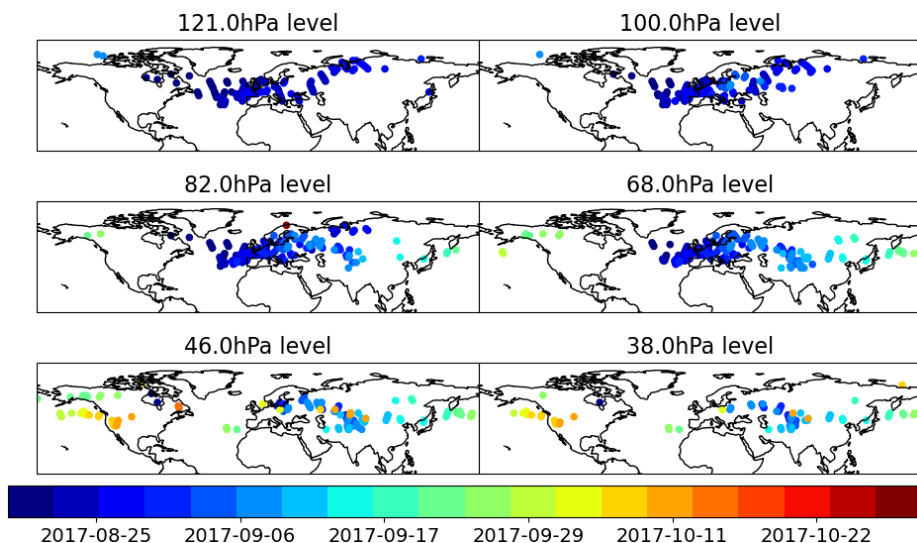
Figure 5.4: Horizontal distribution of the plume at 6 different pressure levels as measured by MLS for BC2017 from 8 August to 30 October 2017. The time of the measurement is color-coded.
