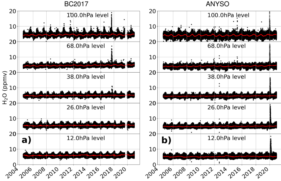
Figure 5.1: A timeline of water vapor mixing ratios measured by the MLS instrument over: a) The northern hemisphere at latitudes between 35^{\circ}\text{N} and 80^{\circ}\text{N} at 5 pressure heights b) The southern hemisphere at latitudes between 10^{\circ}\text{S} and 70^{\circ}\text{S} at the same pressure level. The red lines represent the smoothed data sets.
