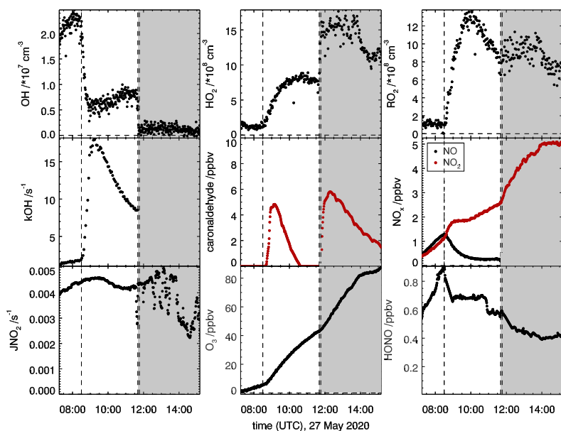
Figure S3 . Overview of measured concentrations for selected species in the SAPHIR chamber for the caronaldehyde photooxidation experiments E5. The shaded area indicates the time where CO was injected as an OH scavenger (experiment E6). Dashed lines indicate times when caronaldehyde was injected into the chamber.
