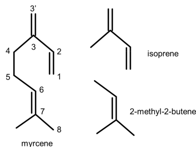
Figure 1. Chemical structures of myrcene, isoprene and 2-methyl-2-butene.
