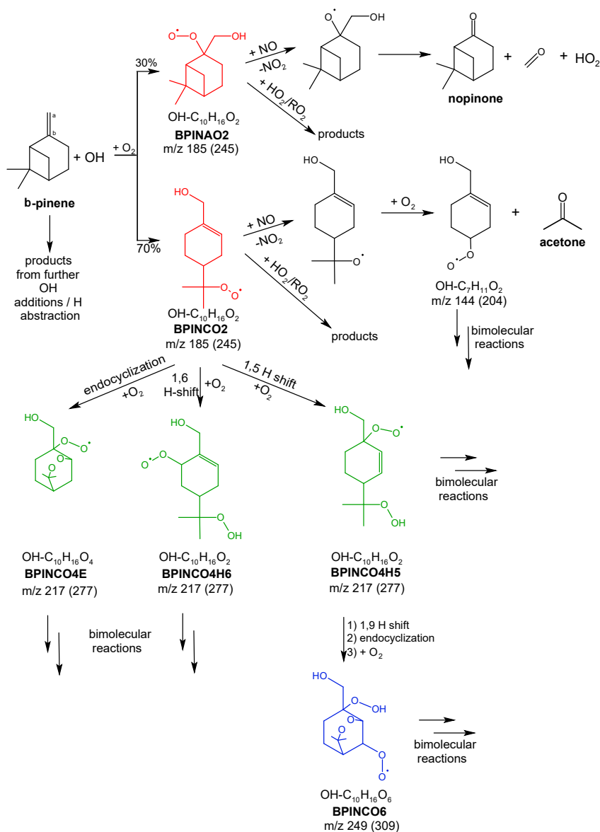
Figure 7.1: The first steps of the mechanism of the oxidation of \beta -pinene with \text{OH} , adapted from Kaminski et al. (2017) and Xu et al. (2019). For simplicity, the addition of \text{OH} is only shown at the \text{C}_a atom, as the branching ratio for an \text{OH} addition at \text{C}_a is 83%. The initially formed peroxy radicals with the sum formula \text{OH-C}_{10}\text{H}_{16}\text{O}_2 are shown in red. Peroxy radicals formed from one autooxidation step ( \text{OH-C}_{10}\text{H}_{16}\text{O}_4 ) are shown in green, peroxy radicals from a second autooxidation step ( \text{OH-C}_{10}\text{H}_{16}\text{O}_6 ) in blue. The mass to charge ratios are given for the respective molecule, and for the clusters of the respective peroxy radical with protonated propylamine ( +60\text{ Th} ) in brackets. Some bimolecular reaction pathways, like the formation of organic nitrates (yield: 25%) from the reactions of the peroxy radicals with \text{NO} are not shown in this scheme. The peroxy radicals can also undergo bi-
