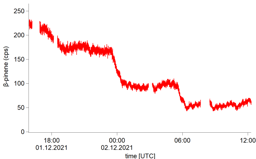
Figure 7.3: Timeseries of the \beta -pinene signal intensity measured by a PTR-MS instrument in an experiment in the SAPHIR-STAR chamber where ozone photolysis was used as an OH source. Only the time prior to the injection of NO is shown. Gaps in the timeseries indicate times when the sampling point of the PTR-MS was switched to the bypass line that provides the \beta -pinene to the chamber.
