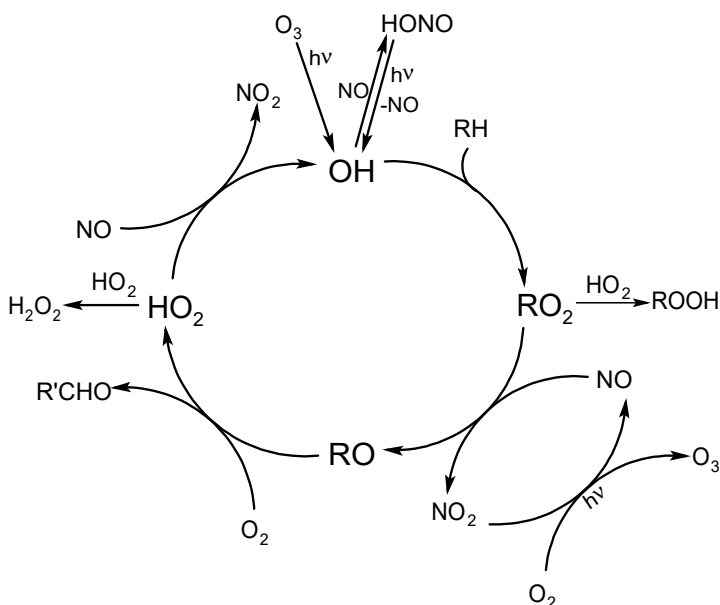
Figure 1.3: Simplified scheme of the daytime radical chemistry in the atmosphere.
