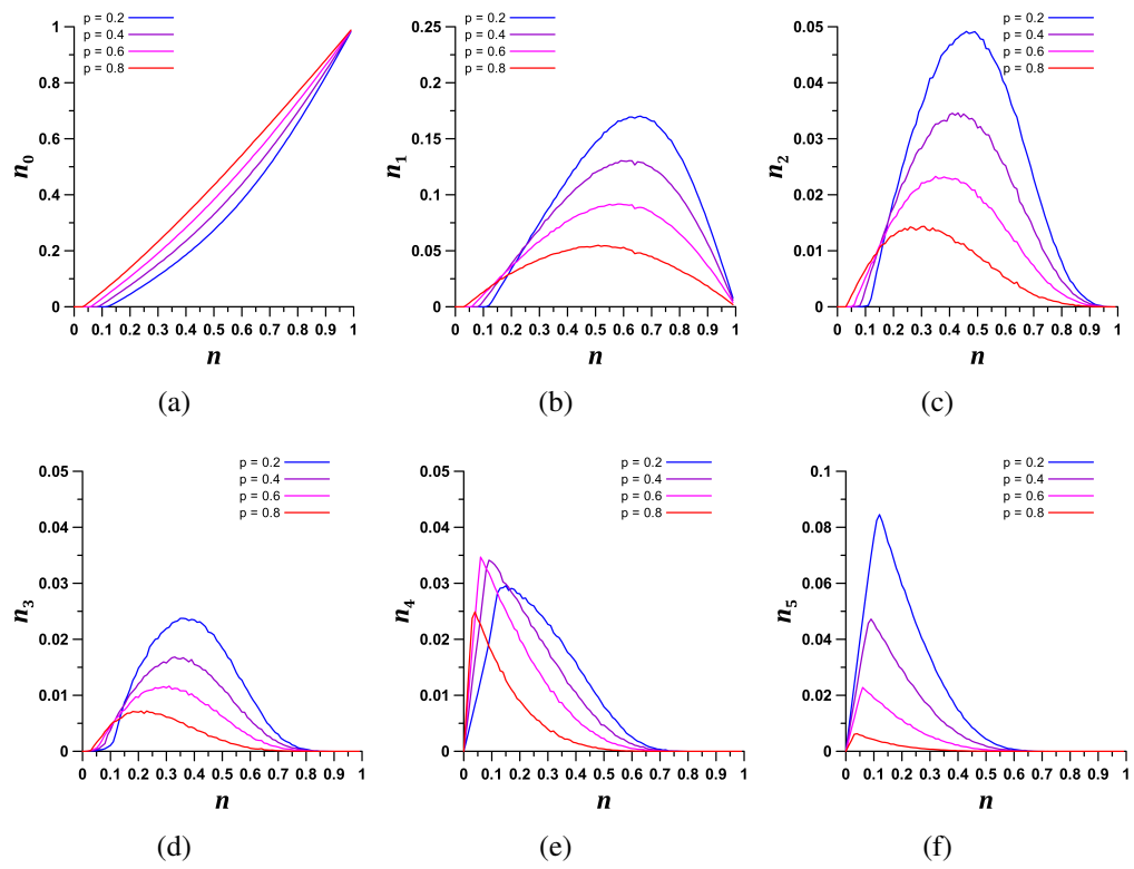
Figure 2 Steady-state velocity distributions of the NS traffic cellular automata as functions of the particle density and stochastic delay. (a) n_0 , (b) n_1 , (c) n_2 , (d) n_3 , (e) n_4 , and (f) n_5 .
