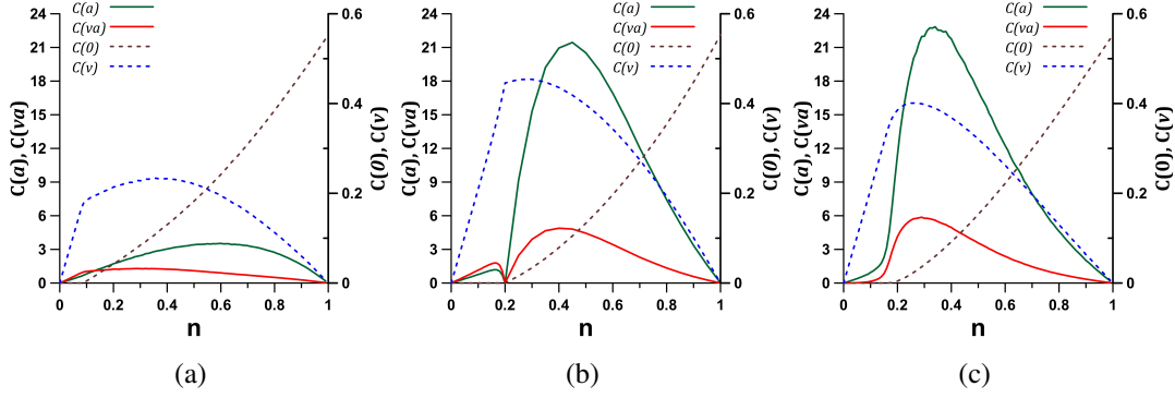
Figure 12 Contributions of the vehicles velocity and acceleration to the steady-state CO 2 emission rate per site (g/s) in traffic cellular automata. (a) NS model, (b) FI model, (c) NS+FI model.
