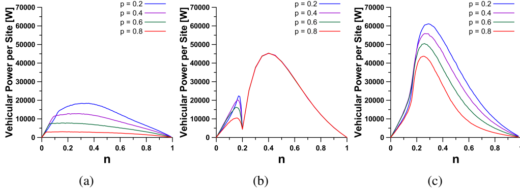
Figure 9 Steady-state vehicular power per site in traffic cellular automata. (a) NS model, (b) FI model, (c) NS+FI model.
