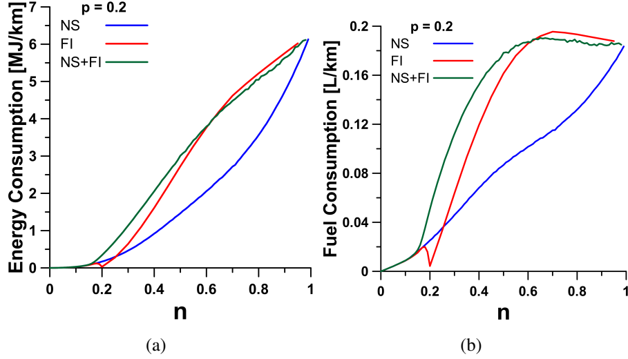
Figure 10 Energy (a) and fuel (b) consumption per kilometer with the NS, FI, and NS+FI driving styles for the stochastic delay p = 0.2 .
