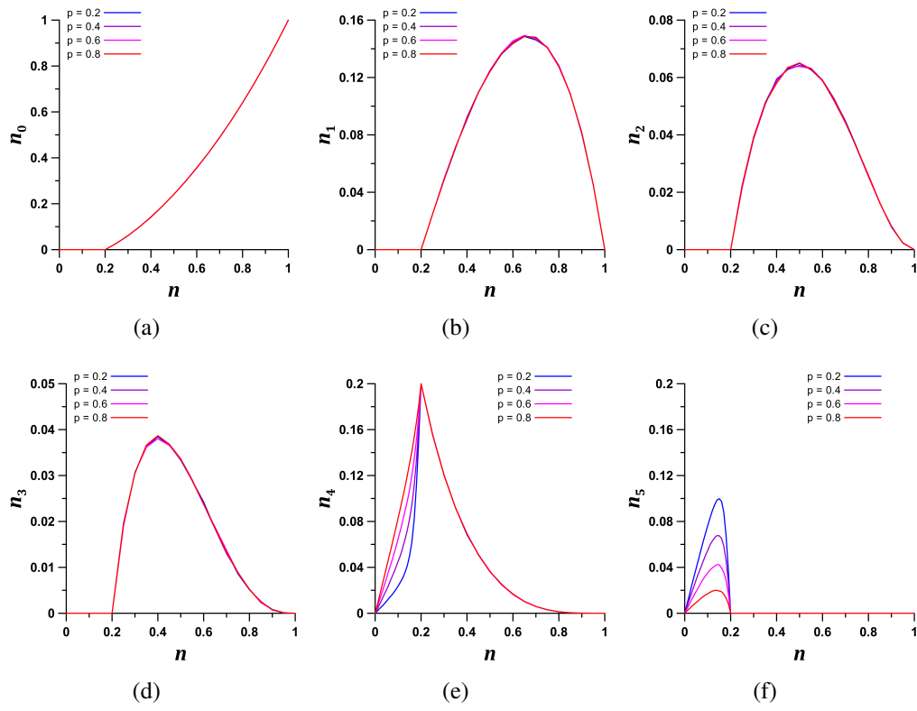
Figure 3 Steady-state velocity distributions of the FI traffic cellular automata as functions of the particle density and stochastic delay. (a) n_0 , (b) n_1 , (c) n_2 , (d) n_3 , (e) n_4 , and (f) n_5 .
