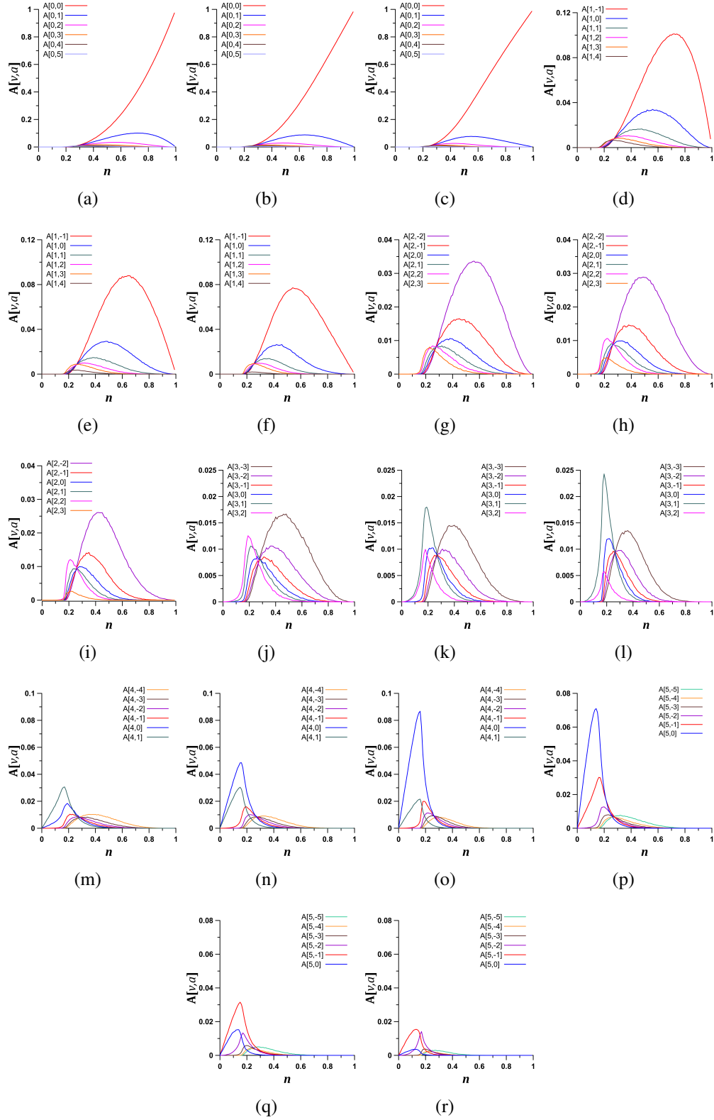
Figure 7 Steady-state acceleration distribution for the NS+FI model with v_{max} = 5 . (a) A_{0j} , p = 0.2 ; (b) A_{0j} , p = 0.6 ; (c) A_{0j} , p = 0.8 ; (d) A_{1j} , p = 0.2 ; (e) A_{1j} , p = 0.6 ; (f) A_{1j} , p = 0.8 ; (g) A_{2j} , p = 0.2 ; (h) A_{2j} , p = 0.6 ; (i) A_{2j} , p = 0.8 ; (j) A_{3j} , p = 0.2 ; (k) A_{3j} , p = 0.6 ; (l) A_{3j} , p = 0.8 ; (m) A_{4j} , p = 0.2 ; (n) A_{4j} , p = 0.6 ; (o) A_{4j} , p = 0.8 ; (p) A_{5j} , p = 0.2 ; (q) A_{5j} , p = 0.6 ; (r) A_{5j} , p = 0.8 .
