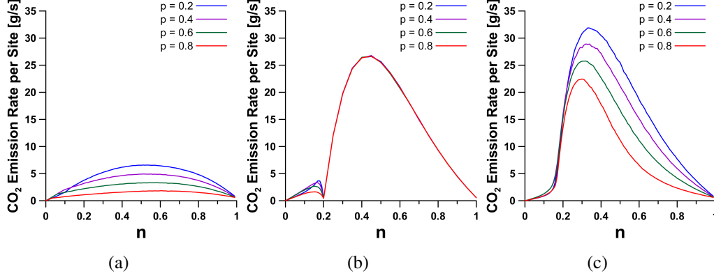
Figure 11 Steady-state CO 2 emission rate per site in traffic cellular automata. (a) NS model, (b) FI model, (c) NS+FI model.
