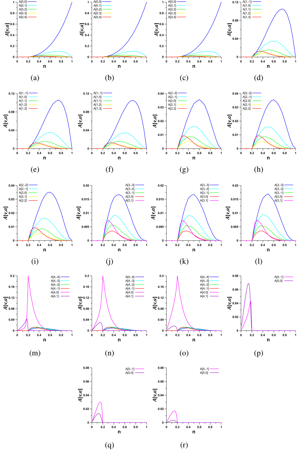
Figure 6 Steady-state acceleration distribution for the FI model with v_{max} = 5 . (a) A_{0j} , p = 0.2 ; (b) A_{0j} , p = 0.6 ; (c) A_{0j} , p = 0.8 ; (d) A_{1j} , p = 0.2 ; (e) A_{1j} , p = 0.6 ; (f) A_{1j} , p = 0.8 ; (g) A_{2j} , p = 0.2 ; (h) A_{2j} , p = 0.6 ; (i) A_{2j} , p = 0.8 ; (j) A_{3j} , p = 0.2 ; (k) A_{3j} , p = 0.6 ; (l) A_{3j} , p = 0.8 ; (m) A_{4j} , p = 0.2 ; (n) A_{4j} , p = 0.6 ; (o) A_{4j} , p = 0.8 ; (p) A_{5j} , p = 0.2 ; (q) A_{5j} , p = 0.6 ; (r) A_{5j} , p = 0.8 .
