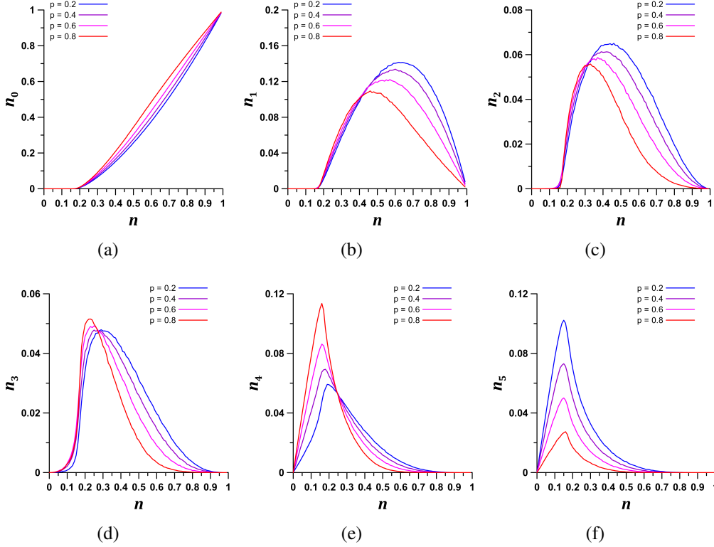
Figure 4 Steady-state velocity distributions of the NS+FI traffic cellular automata as functions of the particle density and stochastic delay. (a) n_0 , (b) n_1 , (c) n_2 , (d) n_3 , (e) n_4 , and (f) n_5 .
