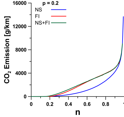
Figure 13 CO 2 emission per kilometer with the NS, FI, and NS+FI driving styles for the stochastic delay p = 0.2 .
