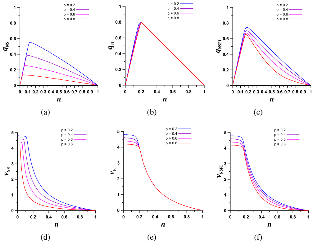
Figure 8 Fundamental diagrams for the traffic cellular automata under (virtually) steady-state conditions. (a) and (d) NS model, (b) and (e) FI model, (c) and (f) NS+FI model.
