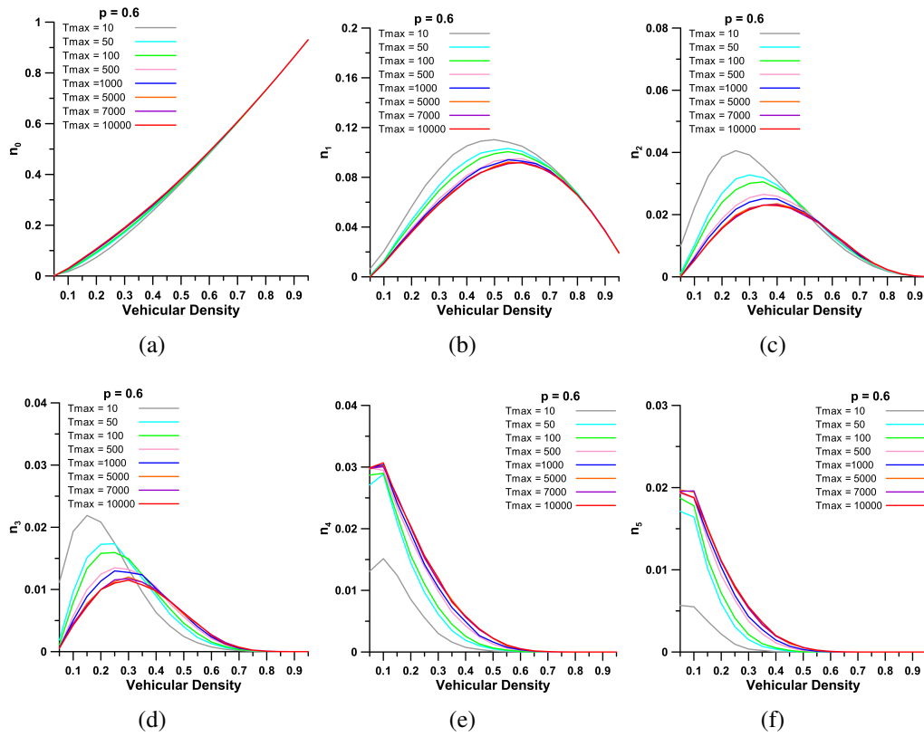
Figure 1 Verification of the steady-state condition. The plots show the partial densities n_0, n_1, \dots, n_5 of the NS model velocity distribution for the case v_{max} = 5 as functions of the particle density for p = 0.6 , and several simulation spans. For T_{max} > 5000 the system is virtually under a steady-state condition. (a) n_0 , (b) n_1 , (c) n_2 , (d) n_3 , (e) n_4 , and (f) n_5 .
