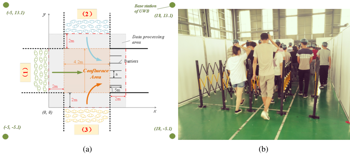
Figure 1 (a) The scene of evacuation experiment. (b) Photographs at the entrance of channelizing facilities.
