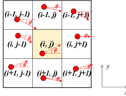
Figure 2 Calculation region of cell (i, j) , which contains the cell (i, j) and its Moore neighborhood cells. Red circles represent the persons in the calculation region at time t .
