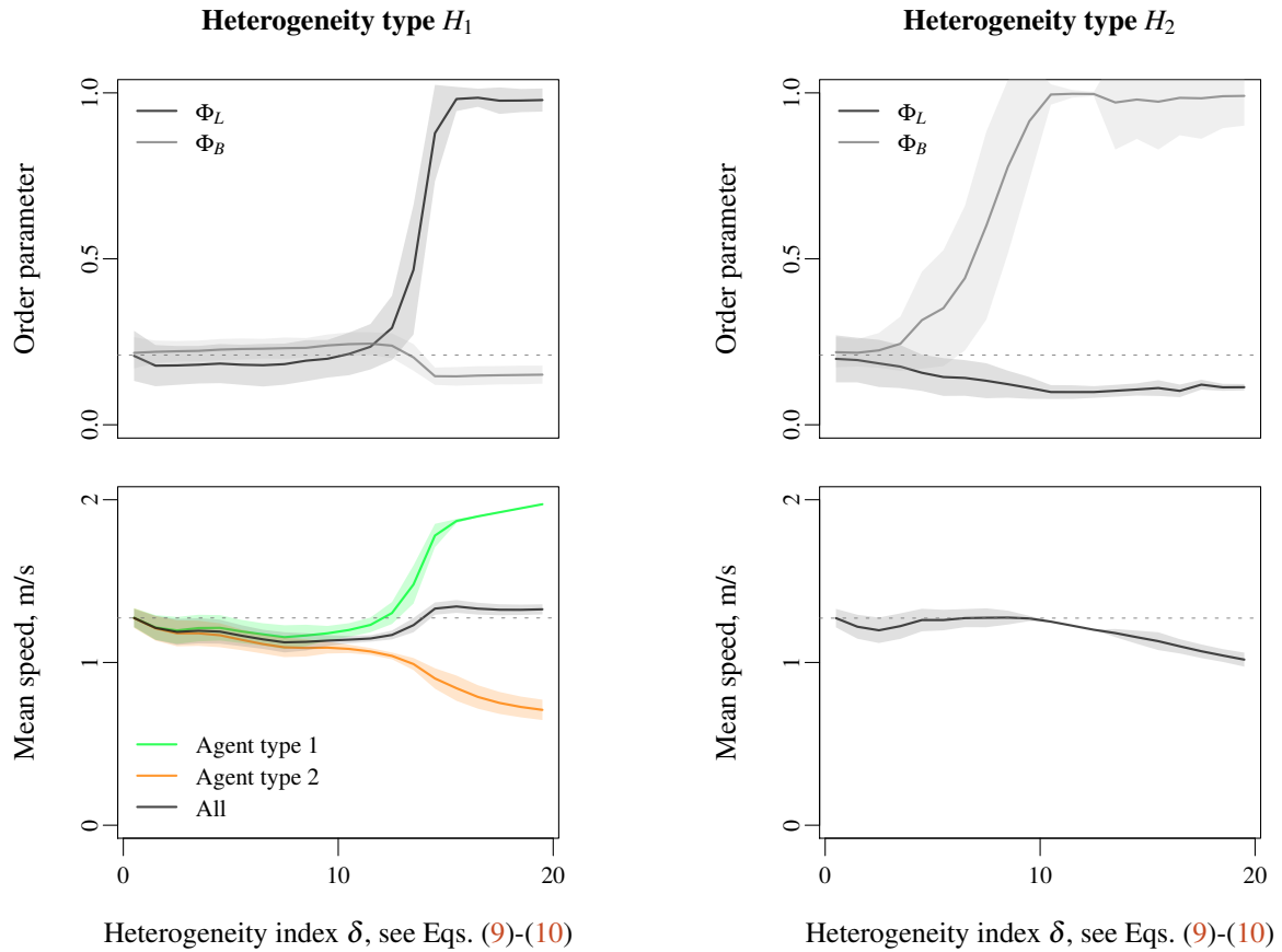
Figure 4 Order parameter for lane and band formation (top panels) and mean speed (bottom panels) according to heterogeneity of agent time gap and desired speed. Horizontal lanes emerge ( \Phi_L tends to 1 while \Phi_B tends to 0) with the model (5) for which the heterogeneity relies on agent characteristics (left panels), while vertical bands appear ( \Phi_B tends to 1 while \Phi_L tends to 0) with the model (6) for which the heterogeneity operates in the interaction (right panels).
