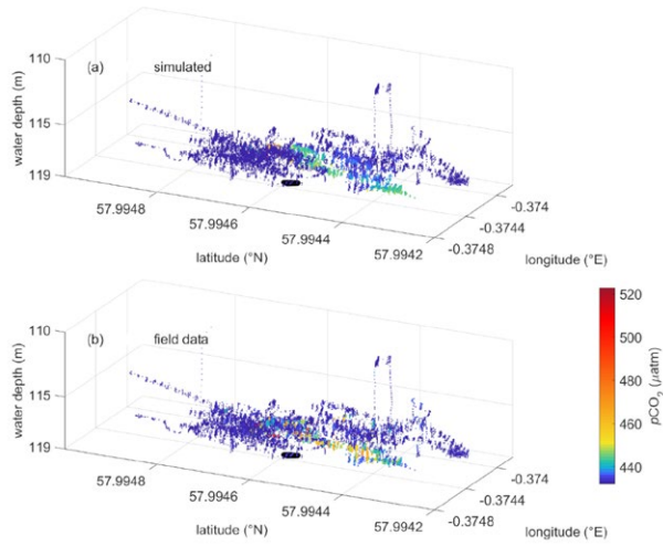
Fig. 3: Comparison of simulated (a) and measured (b) spatial distribution of p\text{CO}_2 in the water column during injection of 143 kg \text{CO}_2 per day into sediment at Goldeneye. The black shape indicates the bubble release site (Gros et al., 2021).
