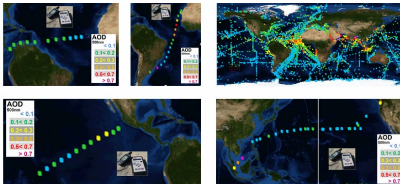
Fig. 1: daily AOD averages (also illustrating the vessel tracks) during MSM79-2 (top left), MSM82-2 (top center), SO267-2 (bottom left) and SO268-3 (bottom right) transit are shown in the context off all shipborne samples contributed to the MAN data-base over the last 18 years (top right).
