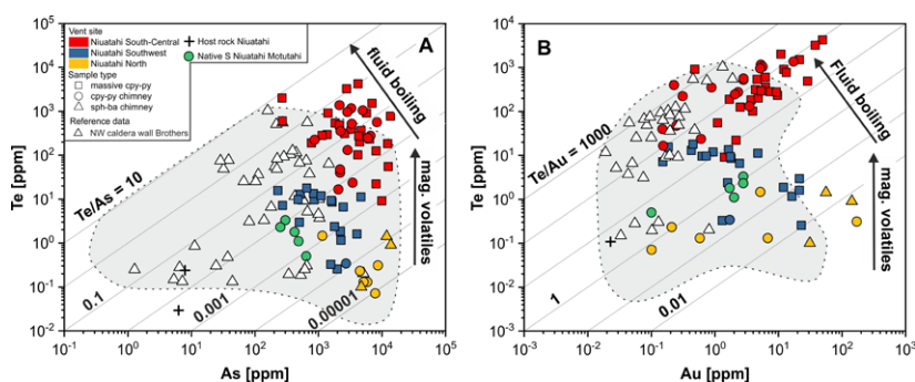
Fig. 2: In-situ LA-ICP-MS composition of hydrothermal pyrite compared to the composition of the magmatic host rock (this study), native S from Niutahi Motutahi (Kim et al. 2011) and pyrite from other subduction zone-related systems (Keith et al. 2016).
