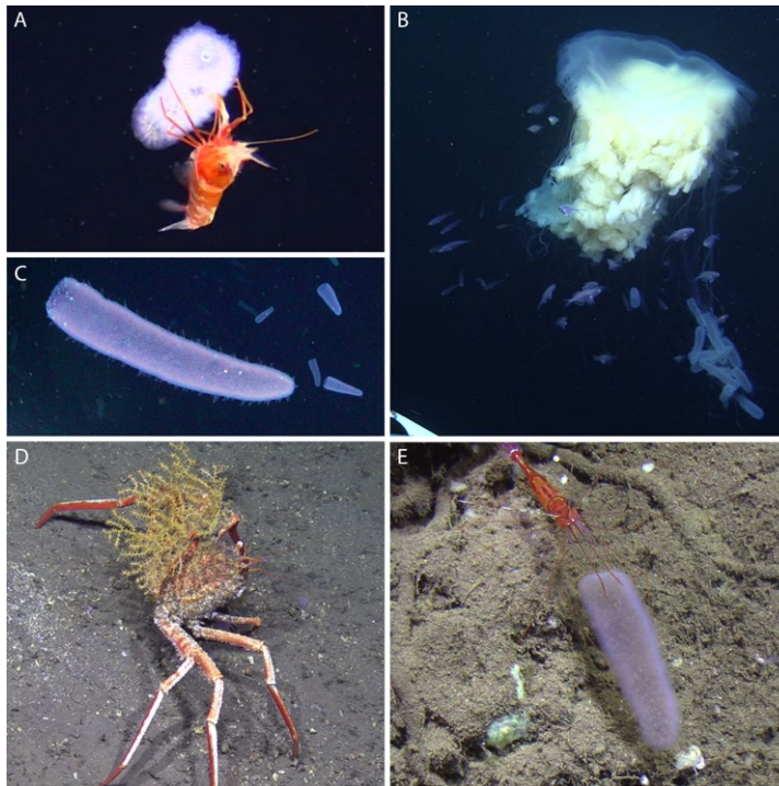
Fig. 4: Pelagic (A,B) and benthic (D,E) animals associated with P. atlanticum (C.) in the eastern tropical North Atlantic, observed in February 2018 and 2019. (A) Unidentified Opolophoridae sp. and (B) Drymonema gorgo feeding on pyrosomes. (C) Pyrosoma atlanticum (D) An unidentified decorator crab, (E) Pandalopsis sp. feeding on pyrosomes. (Stenvers et al 2021)
