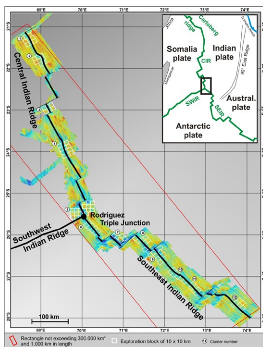
Fig. 2: The German exploration license area along the southernmost Central Indian Ridge and the northernmost Southeast Indian Ridge. Cruise SO271/1 (INDEX 2019) with TFS SONNE addressed the clusters #01, #04, #05, #06, #07, #10, and #12 along the southern Central and the northern Southeast Indian Ridges.
