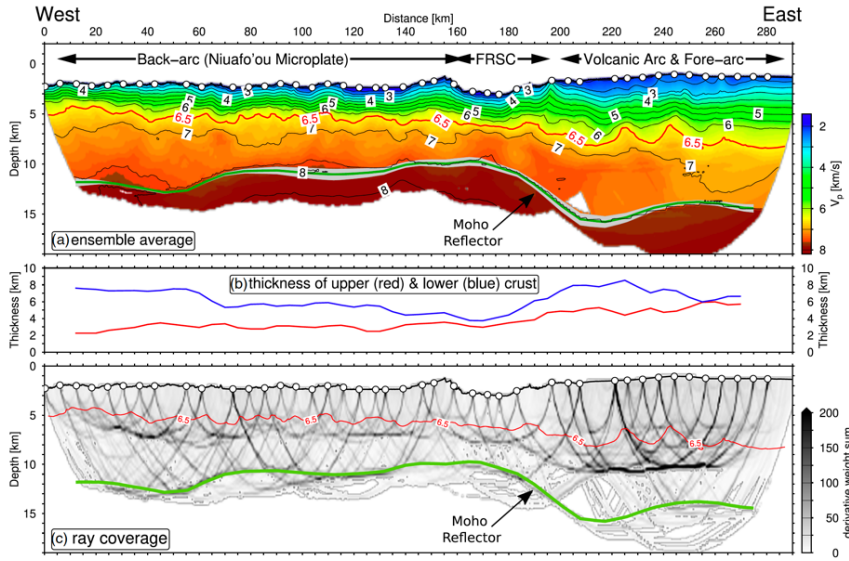
Fig. 2: a) Final P wave tomographic model for BGR-203 with the major tectonic regions indicated. b) Thickness of the upper crust and lower crust. c) Derivative weight sum for individual nodes of the model grid, representing the ray coverage. Red line represents the 6.5 km/s contour, which marks the boundary between upper and lower crust. Solid green line represents the Moho reflector. Image from Schmid et al. (2020).
