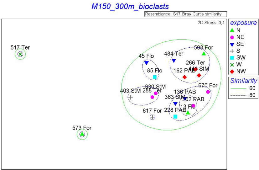
Fig. 2: nMDS plot of sediments from all 300m Stations of M150 Cruise concerning the entire bioclcasts component spectrum. Ter = Terceira, Flo = Flores, StM = St. Maria, For = Formigas, PAB = Princess Alice Bank.
