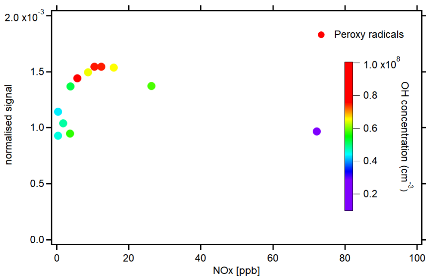
Figure 4.10: The normalised signal of peroxy radicals as a function of NOx. Colour code shows the OH concentration in units of molecules cm -3 .
