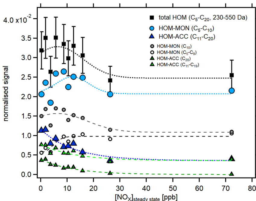
Figure 4.4: The normalised signals of total HOM, monomers, accretion products and HOM that resulted from fragmentation processes, in the mass range of 230 Da to 550 Da as a function of NOx. Black squares show total HOM, blue circles and triangles represent HOM monomers (HOM-MON) and accretion products (HOM-ACC). HOM-MON did not change much as NOx concentration increased while HOM-ACC decreased by \frac{2}{3} at the highest NOx level (72 ppb) compared to reference NOx level (0.3 ppb). Smaller grey and white circles show the signal of C 10 monomers and C 5-9 monomers, respectively. Smaller light green and dark green triangles represent C 20 accretion products and C 11-19 accretion products. From the gain of C 5-9 monomers and the relative gain of C 11-19 accretion products, the increasing importance of fragmentation is deduced. Dashed and dotted lines serve only to guide the eye and have no further meaning. All data presented here were corrected for turnover and particle surface as described in Chapter 2.4.1
