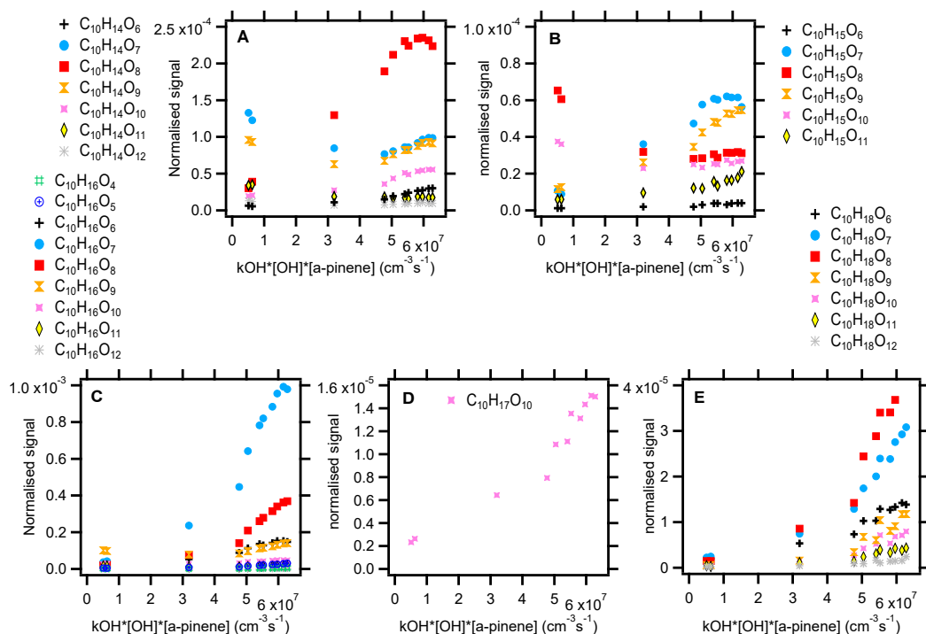
Figure 3.14: The normalised signal of the C_{10} family members versus turnover. Panel A shows C_{10}H_{14}O_z family members and panel B shows members of C_{10}H_{15}O_z peroxy radical family. Panel C shows C_{10}H_{16}O_z family members which was attributed to the mixture of alcohol, hydroperoxide and carbonyl from different peroxy radicals. Panel D shows C_{10}H_{17}O_z peroxy radical family members and panel E shows C_{10}H_{18}O_z family members which is the mixture of the alcohol and the hydroperoxide. Mind that the scale of the y-axes are not same.
