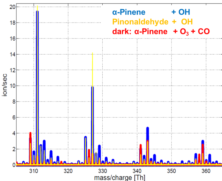
Figure 3.11: Overlapped mass spectrum of \alpha -pinene ozonolysis (red), \alpha -pinene OH oxidation (blue) and pinonaldehyde OH oxidation (yellow). The x-axis shows mass per charge ratio and the y-axis shows non-normalised signal. Pinonaldehyde mass spectrum was scaled to match the \alpha -pinene peak at 310 Th. Compound's mass/charge is shown with a cluster with NO_3^- ion. Data from Iida Pullinen.
