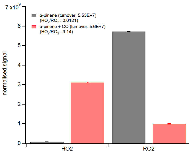
Figure 3.15: Bar graph of modeled HO 2 and RO 2 concentration of two experiments. The HO 2 /RO 2 ratio was 0.012 for the reference experiment and 3.1 for the CO experiment. (Model data were provided by Silvia Proff)
