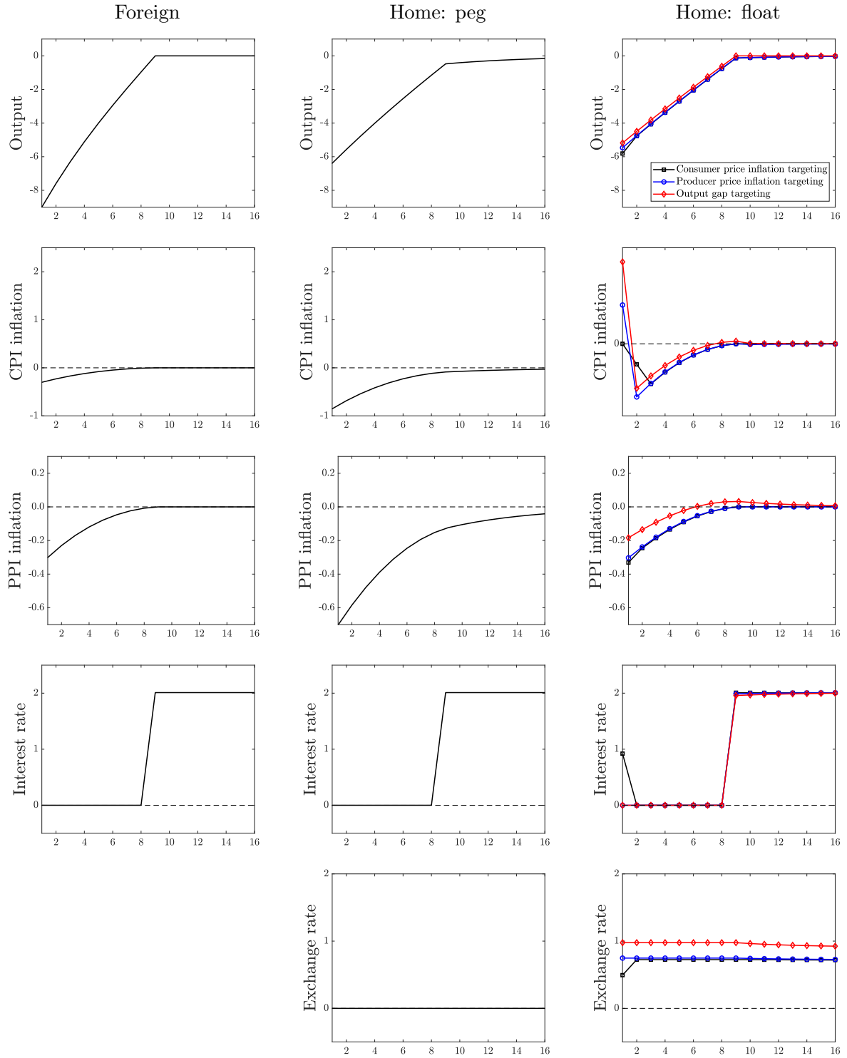
Figure I.10: ELB scenario
