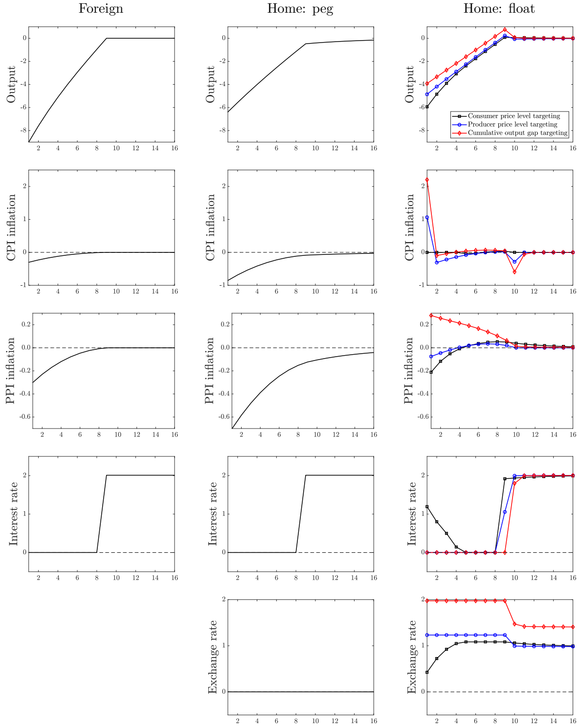
Figure 8: ELB scenario
