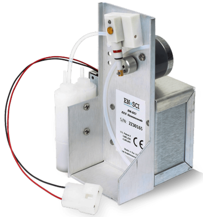
Figure 2.4: Left: Schematics of an ECC ozonesonde (adapted from JOSIE, Jülich) [Smit et al., 2007]. Right: Picture of an ECC ozonesonde (from Manufacturers webpage).
