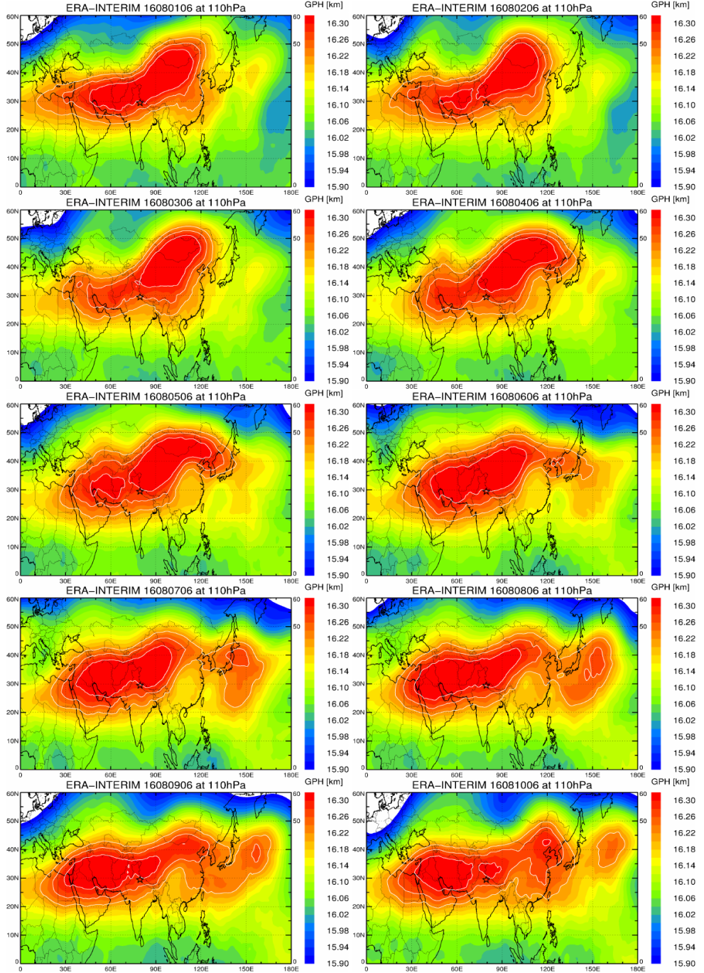
Figure 4.1: The development of GPH at 110 hPa for the first half of August month i.e., from 01-08-2016 till 10-08-2016 for the analysis of balloon soundings over Nainital. Data are from ERA-Interim reanalysis.
