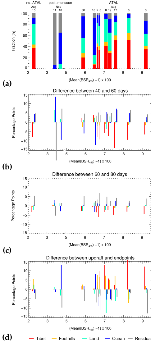
Figure 5.16: Contributions of Tibet, foothills, land, ocean and residual to the boundary layer (BL) sorted by increasing back-scatter ratio (\text{BSR}_{455}-1) \times 100 (see Tabs. 3.1 and 5.2) for 40-day backward trajectories (a). The contributions are normalised by the total number of trajectories within the boundary layer for each day. The days of the soundings in August and November are indicated above the top of the bars. For better representation, the range between 4.0 and 5.0 is removed from the x-axis. Low statistics flights (11, 21, 23 and 26 August) for which the trajectory number is lower than 50% of the maximum number of trajectories (# 704) calculated on 18 August 2016 are not shown as well as the 12 August, when the UTLS is filled by a 5 km thick cirrus cloud. The difference between 40 and 60-day (b) and between 60 and 80-day (c) backward trajectory calculations as well the difference between the location of the end points and the location of strong-updraft (d) for 40-day backward calculations is also shown. This figure has been taken from Hanumanthu et al. [2020].
