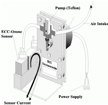
Figure 2.4: Left: Schematics of an ECC ozonesonde (adapted from JOSIE, Jülich) [Smit et al., 2007]. Right: Picture of an ECC ozonesonde (from Manufacturers webpage).
