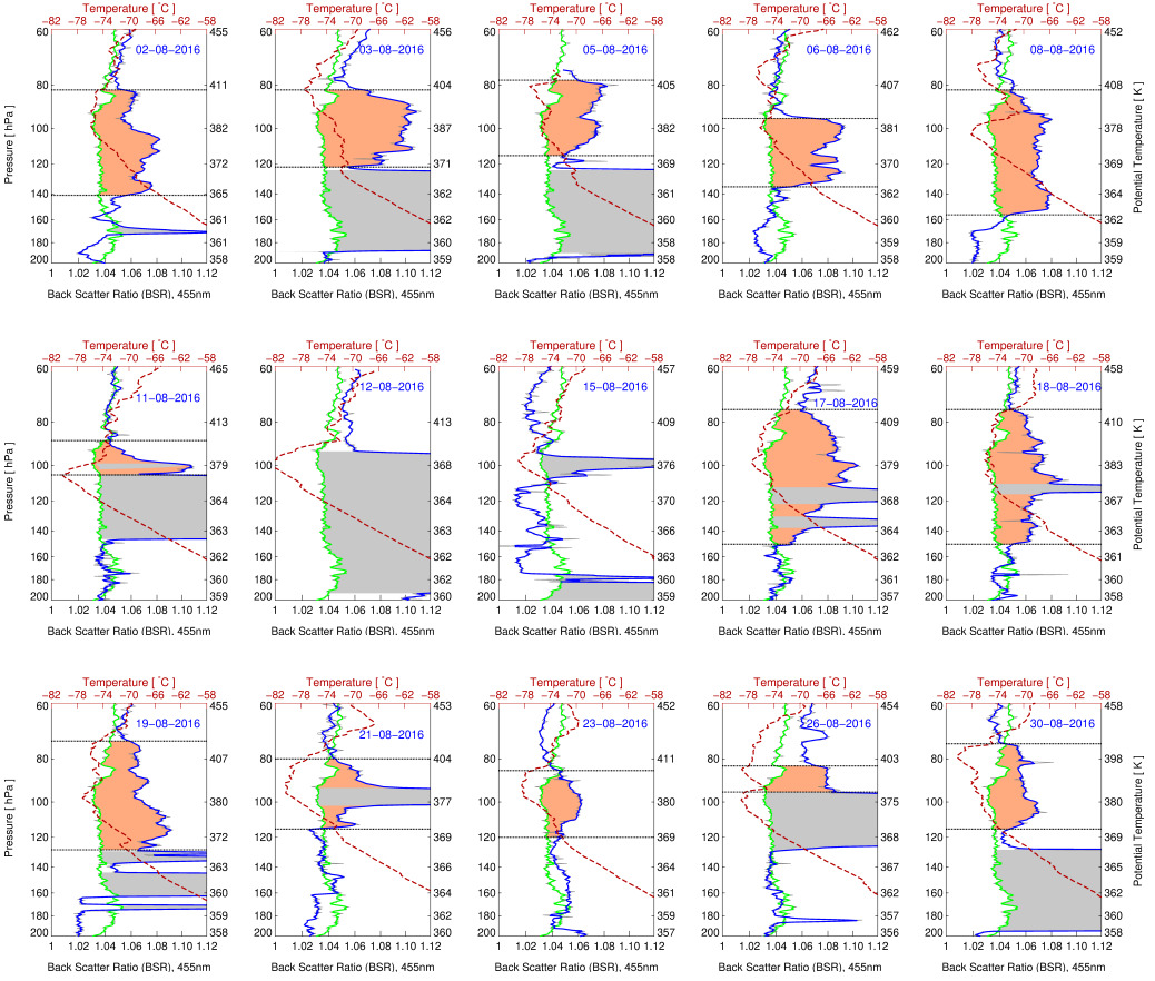
Figure 3.3: COBALD BSR 455 measurements in the UTLS region versus pressure 60–200 hPa for each flight in August 2016 (blue line). Corresponding potential temperature calculated using both measured pressure and temperature is also given for orientation (see right-hand y-axis). The averaged BSR 455 profile of the two November measurements is shown in green. The blue and the green lines show a slightly smoothed representation (three point smoothing) of the original 0.5 hPa binned data (light grey lines; see Sect. 3.2 for details). The measured temperature for each day in August 2016 is shown in red. The ATLAS is highlighted by the orange shading and cirrus clouds are indicated by the grey shading. The top and bottom boundaries of the ATLAS (see Tab. 3.1) are marked by horizontal dashed black lines, except for 12 and 15 August, as no ATLAS was detected on these days (Figure has been adapted from [Hanumanthu et al., 2020]).
