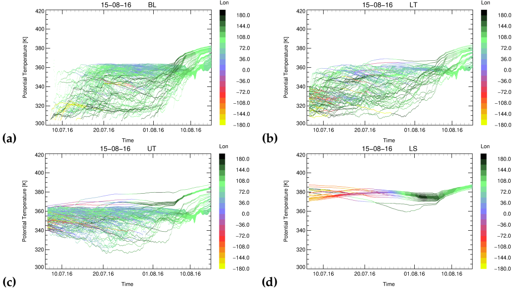
Figure 5.9: The same as Fig. 5.6, but for the no ATAL case on 15 August 2016 (Case2). The trajectories are calculated in a pressure range between 140 hPa and 92 hPa (365 K to 389 K). This figure has been taken from Hanumanthu et al. [2020].
