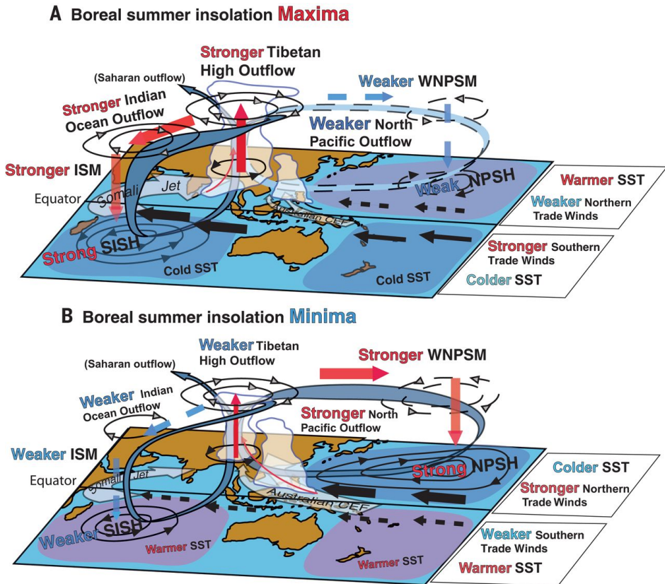
Figure 1.9: The Asian monsoon teleconnections has been demonstrated in the above figure. Inter-tropical seesaw: Orbitaly induced changes in solar insolation mimic the seasonal inter-hemispheric heating-cooling cycle in the tropics and subtropics. (A) During boreal summer insolation maxima, Tibetan high outflow to the southern Indian Ocean subtropical high (SISH) is increased in response to two factors: (i) colder SST in the South Indian ocean, which enhances the surface anticyclone there, and (ii) earlier seasonal transition of the upper-tropospheric subtropical zonal westerly jet [Schiemann et al., 2009; Zhu, 2012; Fu and Lin, 2011] to the north side of the TP, strengthening the Tibetan high. Both factors enhance Hadley circulation and result in strengthening trade winds and Somali jet in the Indian ocean, strengthening the Indian Summer Monsoon. At the same time, outflow to the North Pacific subtropical high (NPSH) is reduced in consequence to warmer north Pacific SST, producing weaker northern trade winds and smaller onshore pressure gradient in the North Pacific, weakening the Western North Pacific monsoon (WNPM). (B) During Boreal summer insolation minima, the opposite occurs. This figure has been adapted from Beck et al. [2018].
