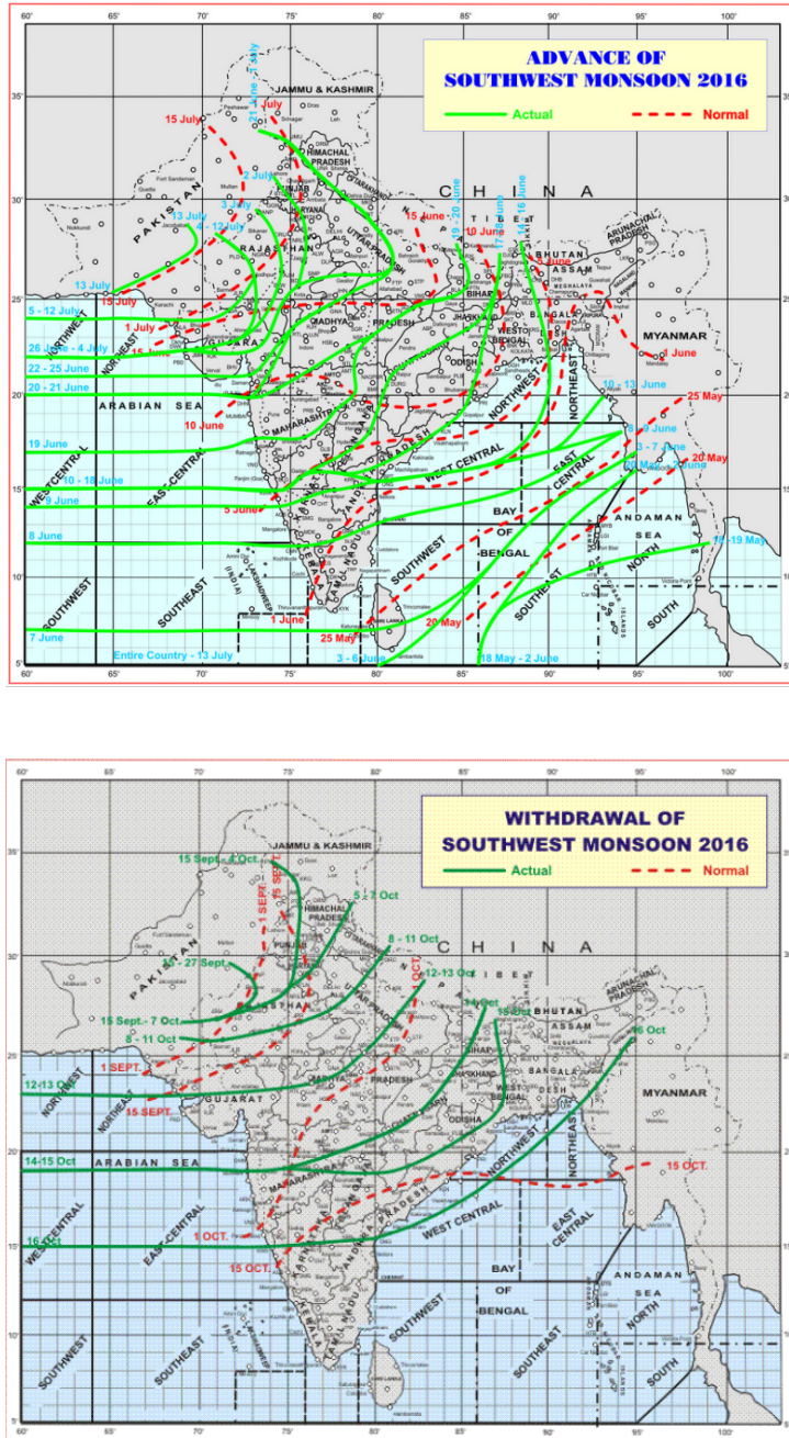
Figure 1.10: 2016 is the year when the measurements were performed. Top: shows (green) and advance of South Asian Summer Monsoon season in 2016 compared to the normal (Climatology) situation. It demonstrate monsoon actual season progression w.r.t climatology (i.e., red) of the following regions and also for the year 2016 (green). Bottom: shows withdrawal dates of monsoon year 2016 over the Indian region w.r.t climatology (i.e., normal, dark red) and also for the year 2016 (i.e., actual, dark green). Figures are adapted from the seasonal reports issued every year by the Indian Meteorological Department (IMD).
