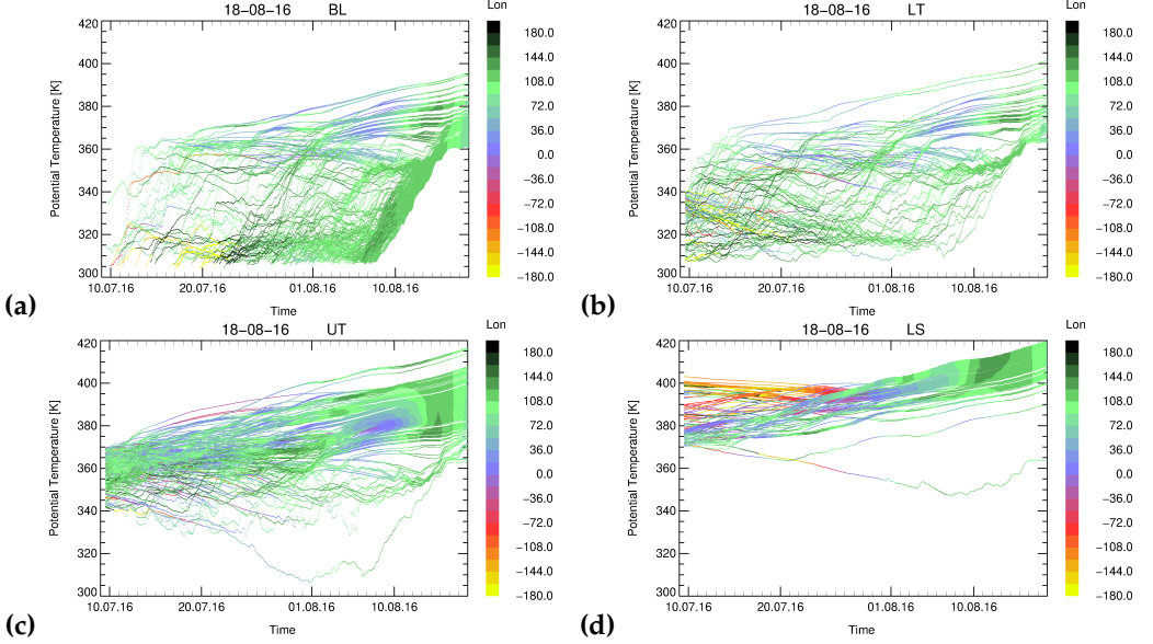
Figure 5.12: The same as Fig. 5.6 and Fig. 5.9, but for Case 3 the typhoon influenced ATAL on 18 August 2016. The trajectories are calculated in a potential temperature range between 150 hPa to 75 hPa (362 K to 422 K). This figure has been taken from Hanumanthu et al. [2020].
