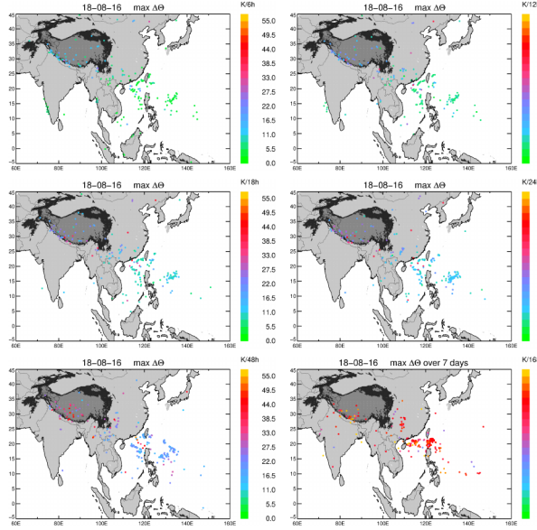
Figure A.11: the change in trajectories contributions w.r.t averaging time intervals, strongest updraft regions are calculated from 40-day backward trajectories (see Tab. 5.1), the difference between backward trajectory calculations depending on the time periods considered which are 6, 12, 18, 24 and 48 hrs and also 7days on 18th of August.
