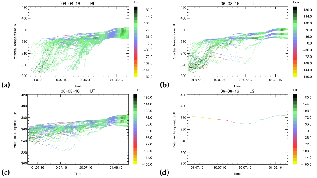
Figure 5.6: 40-day backward trajectories initialized on 6 August 2016 at the location of the ATAL measurement (see Tab. 3.1). The trajectories are sorted by air mass origin in the boundary layer (BL), in the lower troposphere (LT), in the upper troposphere (UT) and in the lower stratosphere (LS). The fractions of the different atmospheric height layers (BL, LT, UT, LS) to the composition of the ATAL are shown in Tab. 5.1. The colour indicates the location of the trajectory in longitude. This figure is taken from Hanumanthu et al. [2020].
