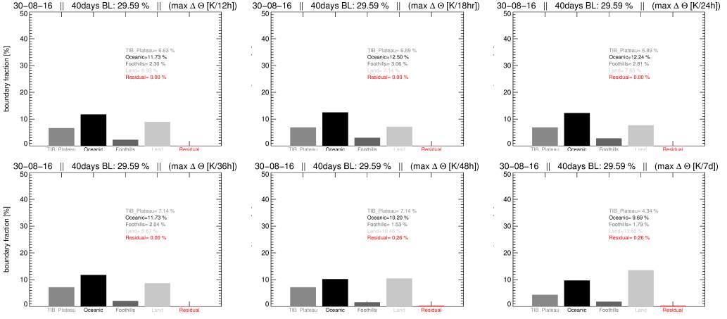
Figure A.28: Strong Updraft criterion followed trajectory sources of 40 day backward run on 30th August.
