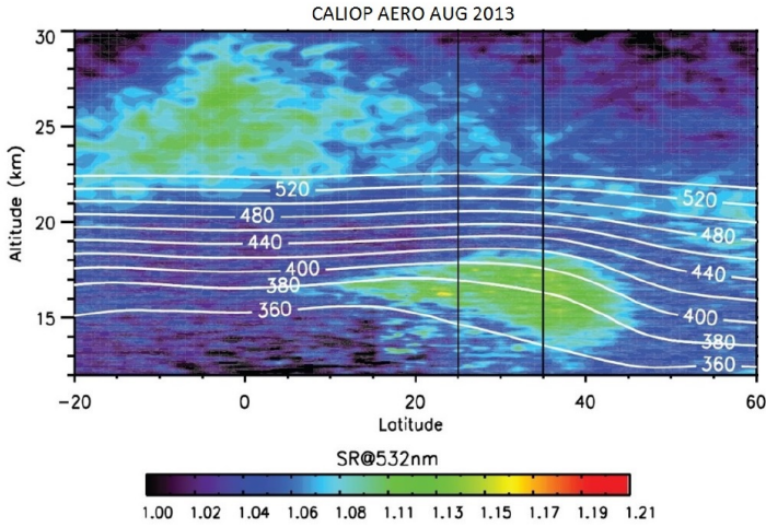
Figure 1.15: Mean CALIOP scattering ratio cross-section averaged between 60^\circ\text{E} and 120^\circ\text{E} in August 2013. Potential temperature isentropes from GOES-5 model are shown with the white lines. Note that clouds observed by CALIOP are filtered when the volume depolarization exceeds 5%, a third method independent from the balloon measurements. This figure demonstrates the ATAL extension meridionally between 15^\circ - 45^\circ\text{N} . Figure has been adapted from Vernier et al. [2015].
