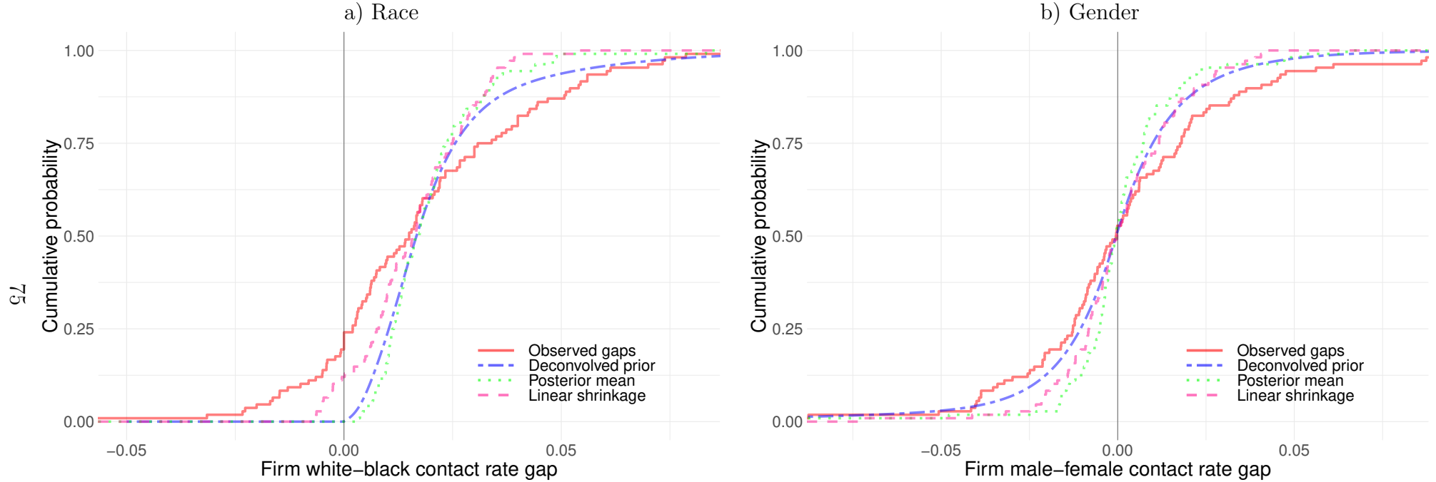
Figure A9: Distribution of observed, deconvolved, and posterior estimates
