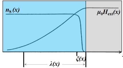
Figure 2.5: Superconductor (blue) to insulator (grey) interface with spatially varying Cooper pair density n_S(x) and the superconducting parameters \xi_{GL}(x) and \lambda_L(x) in an applied magnetic field \mu_0 H_{\text{ext}}(x) .
