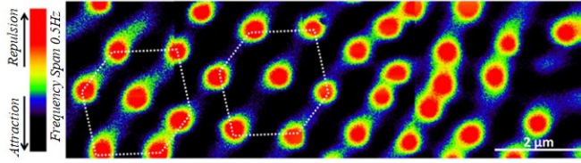
Figure 2.20: Low-temperature MFM measurement of the vortex formation in a Nb/Py heterostructure below T_c and acquired in a field of 19 Oe of the MFM-tip, i.e. perpendicular to the sample surface, taken from [101].
