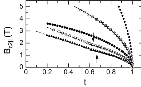
Figure 2.11: Parallel critical field B_{c2||}(t) measured for Nb thin films, taken from [53]. Arrows indicate the temperature t^* below which surface superconductivity comes into play due to a decrease of \xi_{GL} with decreasing temperature, details can be taken from the main text. Solid and dashed lines show the square-root and linear behavior above and below t^* , respectively.
