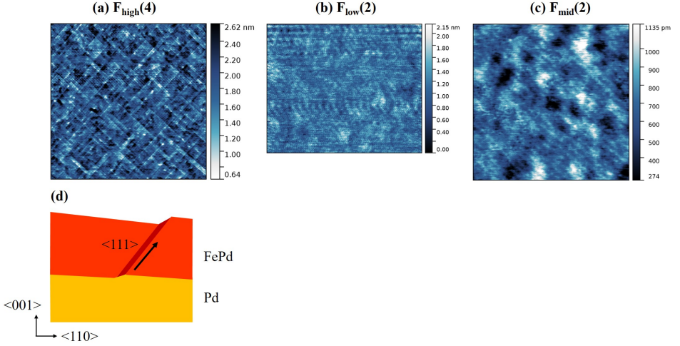
Figure 5.12: (a) 3x3μm AFM measurement of sample F_{\text{high}}(4) , (b) F_{\text{low}}(2) (with 2.5x3μm) and F_{\text{mid}}(2) (3x3μm). (d) Plane defects along (111) in a thin film FePd layer of strong PMA can cause surface terraces visible in sample F_{\text{high}} in (a), Figure inspired from [17].
