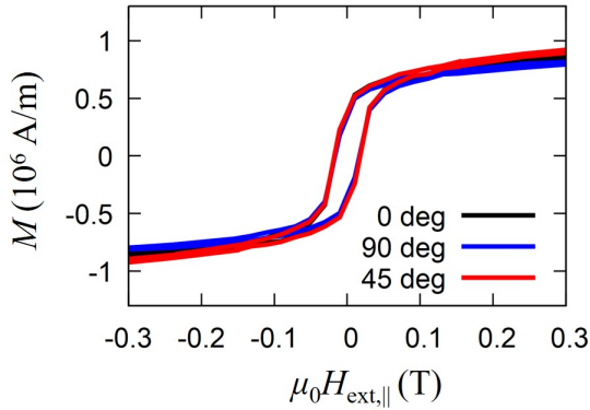
Figure 9.14: Hysteresis loops at 300 K in an in-plane applied field of sample SF low (1) at various angles between the \langle 100 \rangle crystalline axis and the magnetic field. Here, 0^\circ denotes a field applied along \langle 100 \rangle .
