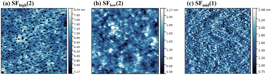
Figure 9.9: 3 \times 3 \mu\text{m} AFM images of samples \text{SF}_{\text{high}}\text{-}\text{SF}_{\text{low}} at room temperature.
