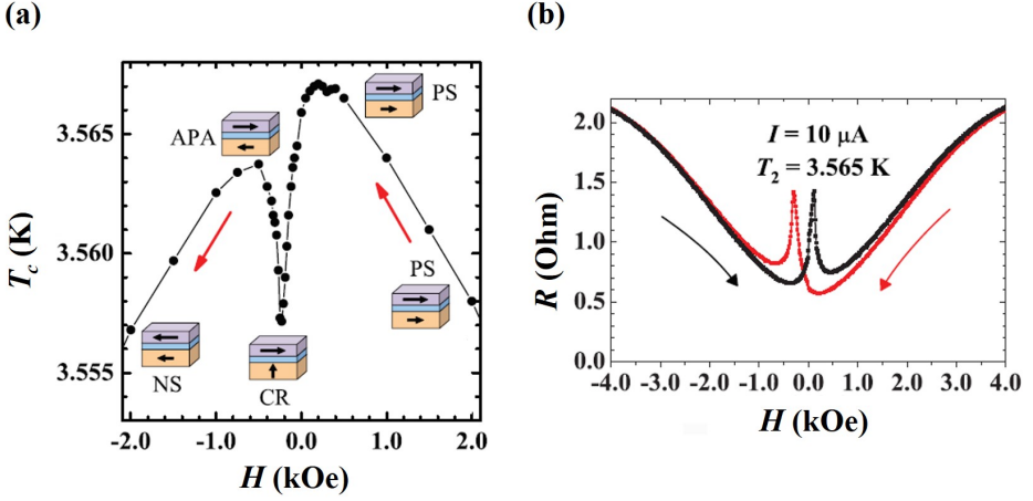
Figure 2.24: (a) Dependence of the critical temperature T_c on the magnetic field for different relative magnetization orientations of the F1 and F2 layers, marked in dark and light red. The thin blue layer between F1 and F2 denotes a normal conducting interlayer to independently switch the magnetization inside the two F layers. (b) Resistance measurements with respect to an external field H at constant temperature for the sample shown in (a). Figure taken from [116].
