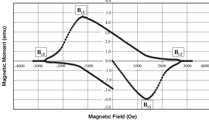
Figure 2.10: Magnetic hysteresis of bulk Nb adapted from [67].
