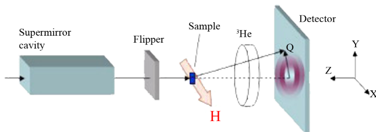
Figure 4.13: Instrument setup of vSANS, taken from [167].
