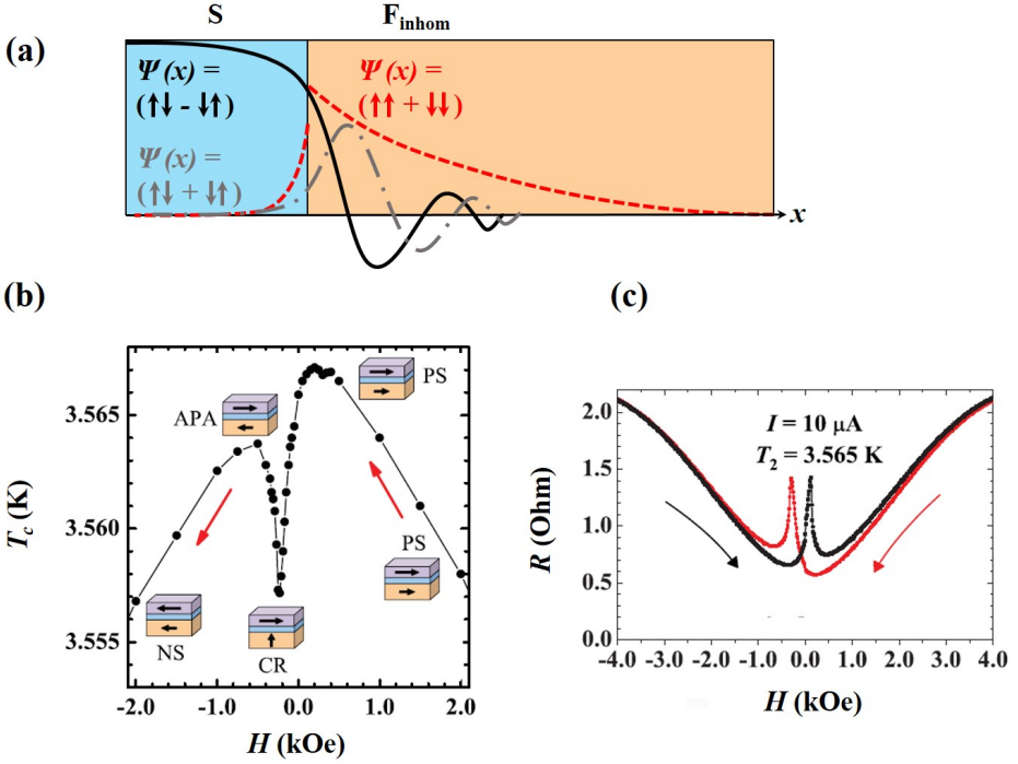
Figure 6.12: (a) Schematic sketch of the penetration of Cooper pair components from S into an inhomogeneous F layer. Black lines denote spin-singlet components, grey lines denote spin-triplet components with S_z = 0 and red lines denote spin-triplet components with S_z = \pm 1 . (b) Critical temperature T_c and (c) resistance R with respect to an external magnetic field H , taken from Zdravkov et al. [116].
