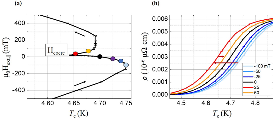
Figure 9.15: (a) Dependence of T_c on the applied field \mu_0 H_{\text{ext},||} of \text{SF}_{\text{low}}(1) . All data points in (a) are extracted from \rho(T) measurements such as those displayed in (b). Red arrows indicate a transition of T_c first to lower values and subsequently to increasing values for increasing magnetic fields.
