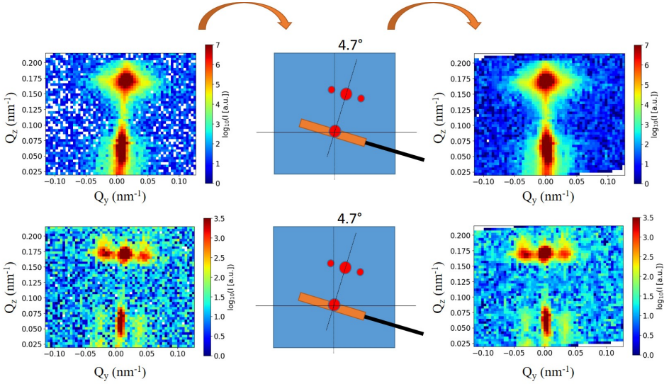
Figure 9.16: Q_y - Q_z -maps of the I^- and I^+ channels of polarized GISANS at T_B = (10.10 \pm 0.02) K on \text{SF}_{\text{high}}(2) (left) before rotation, and (right) after a rotation of 4.7^\circ due to a slightly tilted GISANS holder as sketched in the middle.
