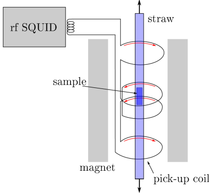
Figure 4.10: Schematic instrument setup of the rf-SQUID and the sample environment: the sample is mounted in a straw and placed between pick-up coils to transfer the induced voltage to the rf-SQUID. Taken from [128].
