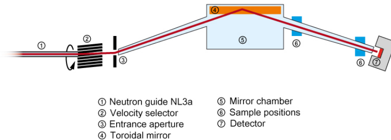
Figure 4.12: Instrument setup of KWS-3, taken from [164].
