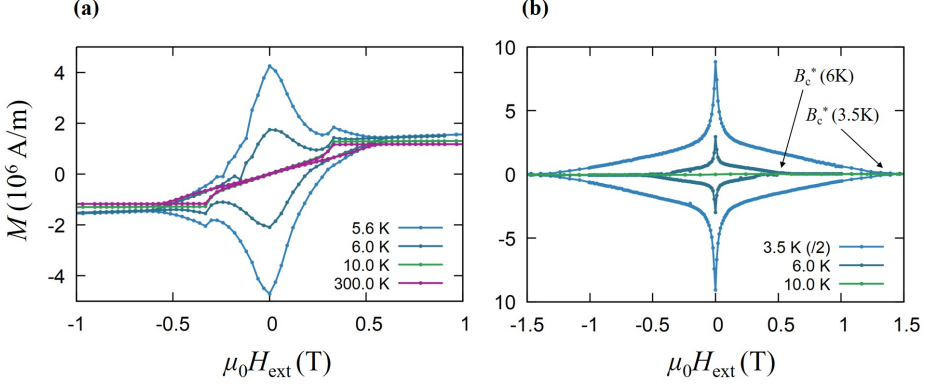
Figure 6.1: (a) M(H_{\text{ext},\perp}) of \text{SF}_{\text{high}}(2) measured at various temperatures indicated by the legend. (b) Hysteresis loops of \text{S}(5) with corresponding Nb thickness to \text{SF}_{\text{high}}(2) ( d_{\text{Nb}}=39 nm, see tables 9.1-9.6).
