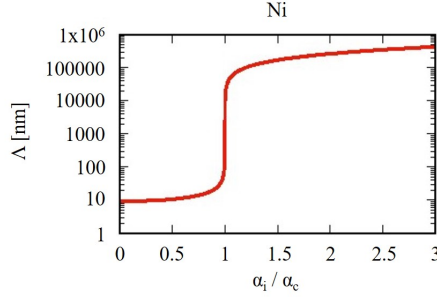
Figure 3.7: Penetration depth of the neutron beam \Lambda into Nickel as function of the incident angle \alpha_i at a neutron wavelength of 6 Å.
