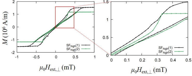
Figure 9.13: Magnetization with respect to an out-of-plane applied field \mu_0 H_{\text{ext},\perp} of SF high (1) and SF high (2).
