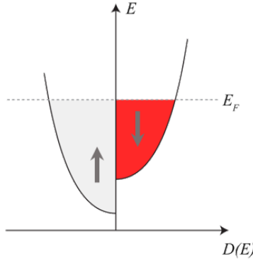
Figure 2.1: Density of states D(E) for a metallic ferromagnet with majority spin up and minority spin down bands filled up to the Fermi energy E_F .
