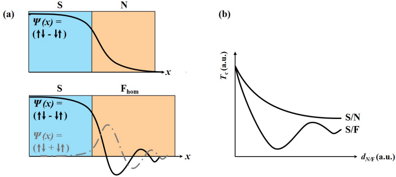
Figure 2.16: Comparison of S/N and S/F hom proximity effects with a homogeneous magnetization inside F hom . (a) \psi(x) of the spin-singlet components decays monotonically over x inside N. Inside S/F hom , the shift of energy bands for up and down spin orientation leads to an oscillation in \psi(x) and a phase shift for the spin-singlet (black line) and spin-triplet (grey line) components with S_z = 0 . (b) Dependence of T_c on the thickness of the proximity coupled layer. In S/N, T_c decreases monotonically with increasing d_N , whereas in S/F hom , T_c oscillates with increasing d_F . Figure (b) is inspired from [85].
