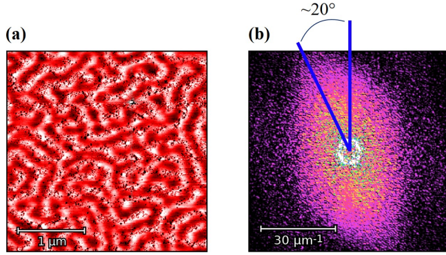
Figure 9.19: (a) 3x3μm MFM image of SF_{\text{high}}(2) at room temperature under zero field and (b) 2D-FFT analysis of (a) performed using the software Gwyddion [194]. The dark blue line denotes a preferential direction of magnetic domains visible by a distortion from a circular shape.
