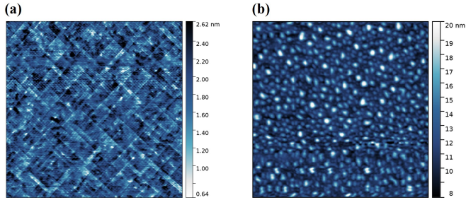
Figure 5.13: 3x3μm AFM measurements of sample F_{\text{high}}(4) in the as-grown state with a flat surface (a) and after three weeks of sample aging with islands of \sim 20 nm height (b).
