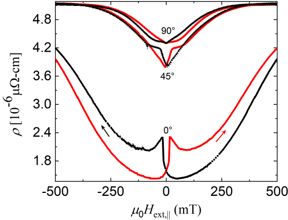
Figure 6.14: \rho(H_{\text{ext},||}) at various external magnetic field angles with respect to the sample surface: 0^\circ denotes a magnetic field applied parallel to the \langle 100 \rangle axis and 90^\circ a magnetic field applied along the \langle 001 \rangle axis (i.e. perpendicular to the sample surface). All measurements are obtained at T = 4.5 K.
