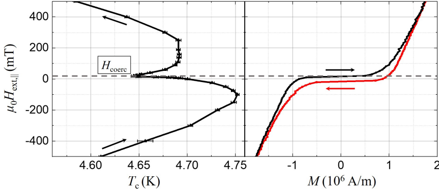
Figure 6.13: H_{\text{ext},||}(T_c) of \text{SF}_{\text{low}} (left), all data points are measured after saturation of the sample in a negative magnetic field. The corresponding hysteresis loop (right) is measured in both field sweep directions at T = 3.5 K, adapted from [181].
