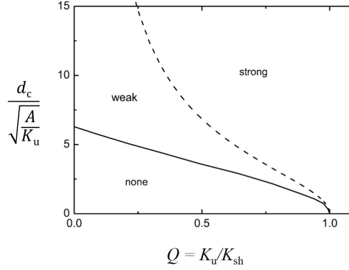
Figure 5.2: Critical thickness d_c with respect to Q = \frac{K_u}{K_{sh}} for uniaxial thin films, Figure adapted from Viro et al. [172]. The area above the dashed line denotes thicknesses and Q values leading to strong PMA, whereas between the dashed and solid lines a weak PMA is evolved. Below the solid line, no PMA occurs in the thin film.
