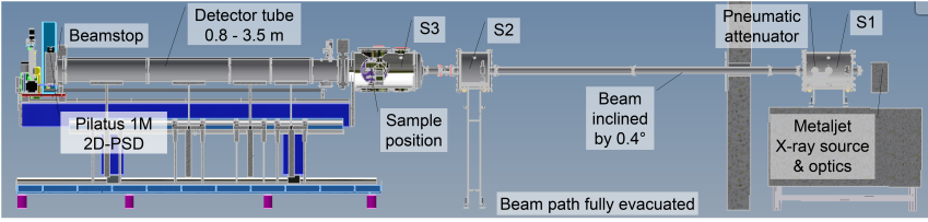
Figure 4.11: Instrument setup of GALAXI, taken from [141].
