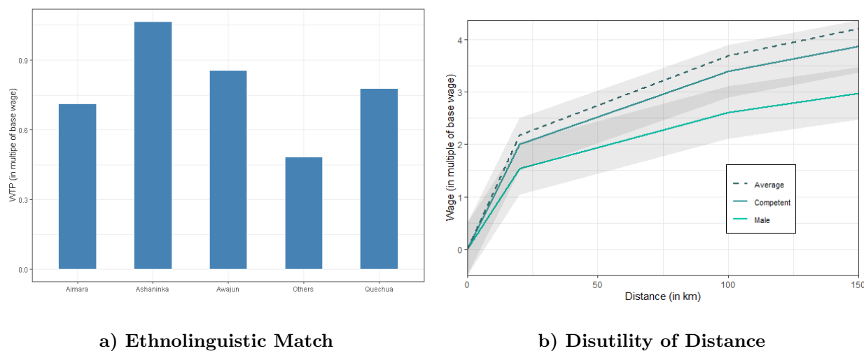
Figure C.1: Match Effects
