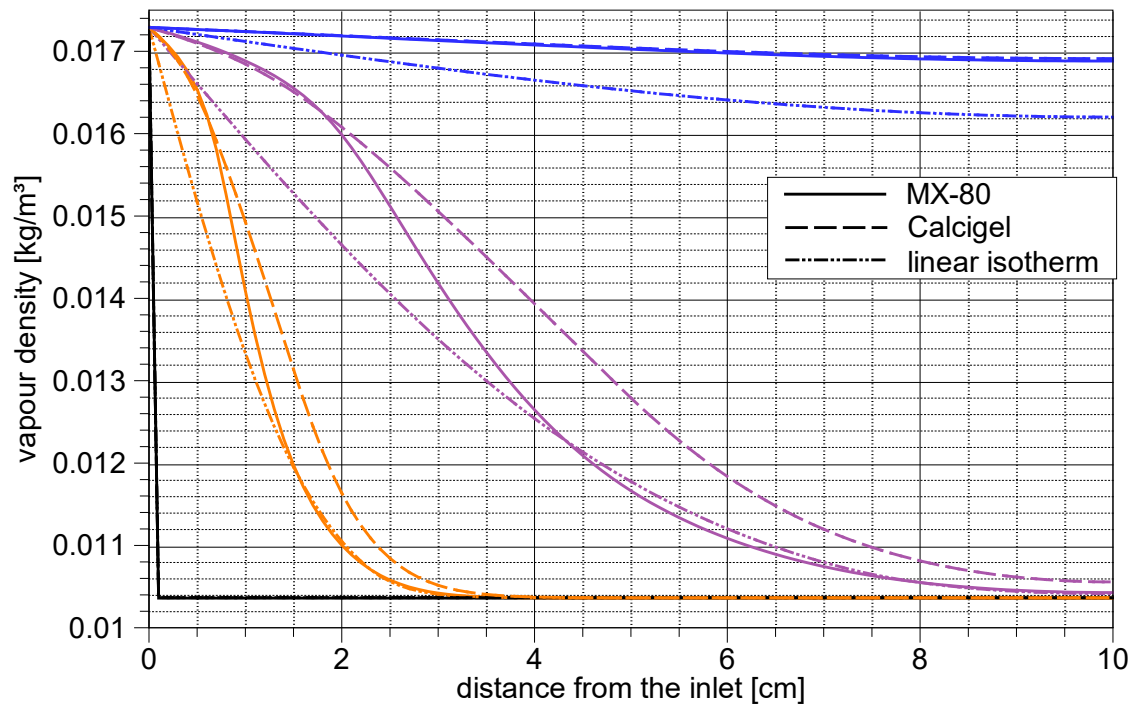
Fig. 8.4 Simulated vapour density distributions based on four adsorption isotherms; results at 0 (black), 1 (orange), 10 (violet) and 100 (blue) days
