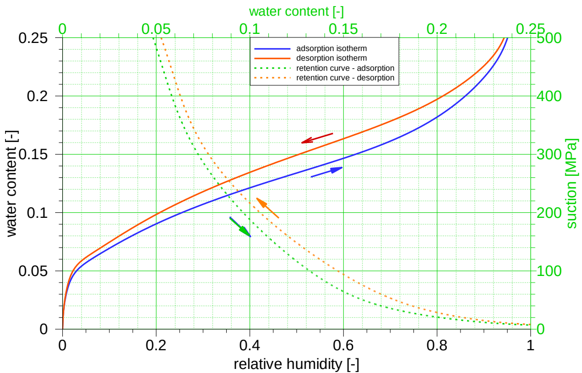
Fig.3.6 Hysteresis of the isotherms for Calcigel at 25 °C and analytical formulations
