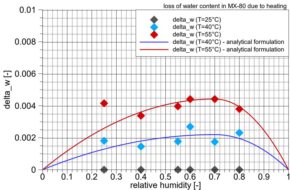
Fig. 5.22 Fit of an analytical formulation to the loss of water content of MX-80
