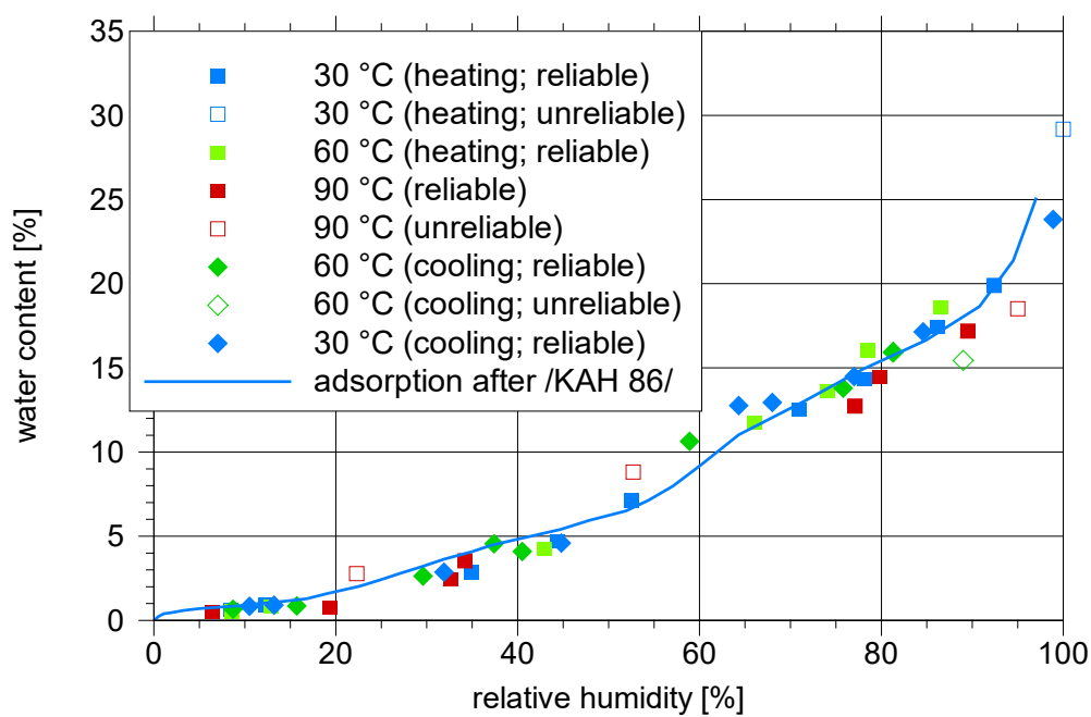
Fig. 5.13 Comparison to data from /KAH 86/
