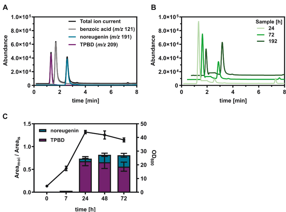
Figure 9: Detection of the noreugenin synthesis intermediate 1-(2,4,6-trihydroxyphenyl)butane-1,3-dione (TPBD) in extracted cultivation samples. (A) Exemplary chromatogramm of an extracted cultivation sample both as total ion current and the individual m/z ratios. (B) Total ion current chromatograms of extracted samples resembling the spontaneous cyclization of TPBD towards noreugenin over the cultivation time. For better visualization, the benzoic acid signal was removed from the chromatogram. (C) Growth curve and product abundance for the strain C. glutamicum M-CoA pMKEx2- pcs AaCg -short. Unavailability of an authentic TPBD standard prevented quantification of this particular molecule. To evaluate product formation over time, the normalized signal areas of the molecules of interest (Area mol ) TPBD and noreugenin were added up. Signal area of the internal standard (Area is ) benzoic acid was used for normalization. The calculated ratios are depicted on the primary Y-axis. At the given sampling time points, OD 600 of the cultures was also determined (filled circles, shown on secondary Y-axis). The obtained data represent mean values with standard deviations from biological triplicates.
