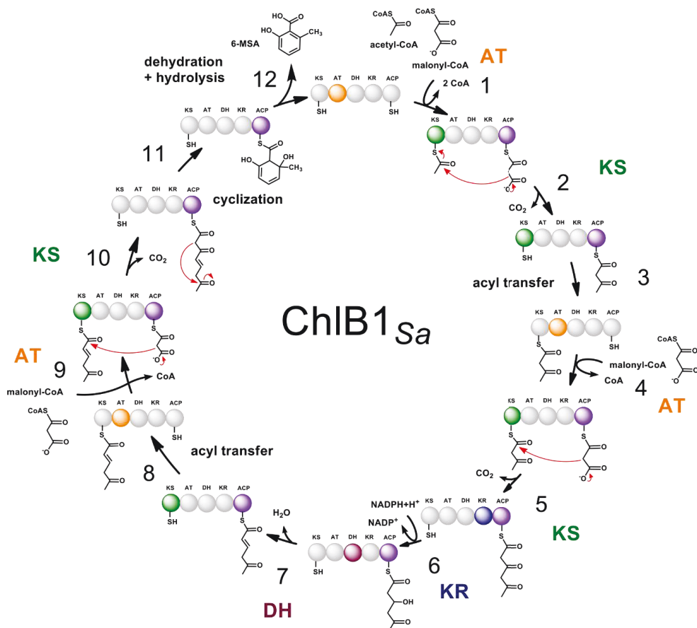
Fig. 1 6-Methylsalicylic acid formation by the type I PKS ChIB1 Sa . The depicted steps follow a previously established reaction sequence. 6-Methylsalicylic acid is produced from acetyl-CoA and three molecules of malonyl-CoA. Acetyl-CoA as starter unit is consumed in step 1, whereas three malonyl-CoA molecules are consumed in steps 1, 4, and
