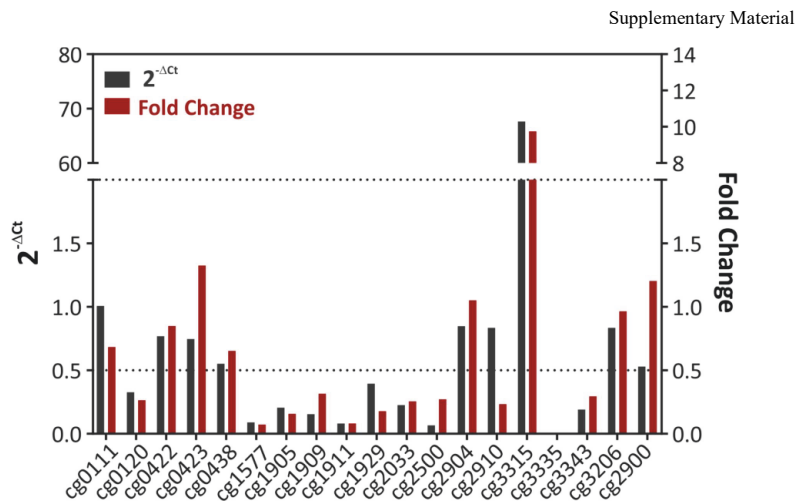
Figure S4: Verification of DNA-microarray data using qRT-PCR. Microarray data were verified with qRT-PCRs (oligonucleotides are listed in Table S3 D). The dark-grey bars represent the relative transcriptional change based on the qRT-PCR data and the red bars show the average fold-change obtained from DNA microarray experiments. The values below 0.5 are classified as “downregulated”, the values above 2 are classified as “upregulated”. In the case of cg3335, the bars are not visible because of very low values (qRT-PCR: 0.018, DNA-microarray: 0.007).
