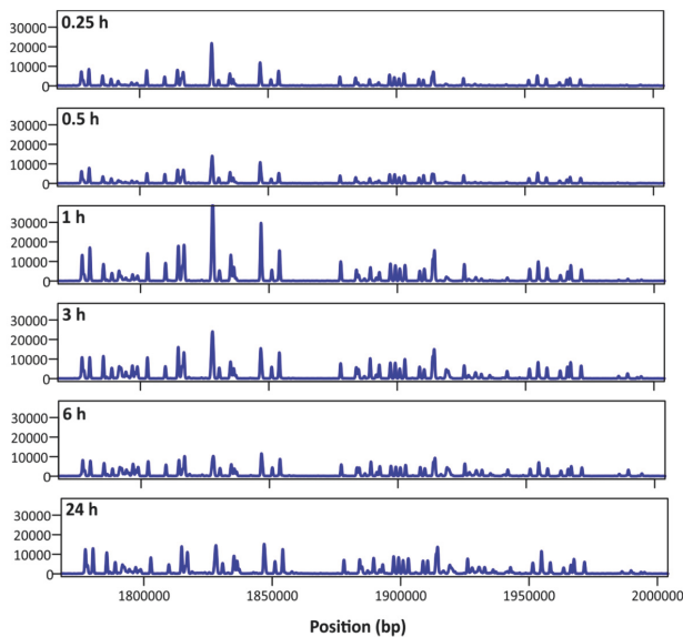
Figure S3: Enlargement of the CgpS binding inside the CGP3 region. This plot is a zoomed-in version of the time series represented in Figure 4. This zoom only shows the CGP3/CGP4 area of the chromosome. For the data generation, C. glutamicum ATCC 13032::cgpS-strep cells were grown as described previously in CGXII medium containing 2 % (w/v) glucose and 600 nM mitomycin C (all but t = 0 h). Subsequently, cells were harvested at different timepoints (0 h, 0.25 h, 0.5 h, 1 h, 3 h, 6 h, 24 h) and CgpS-bound DNA was purified and sequenced. The presented data was normalized with regard to the average intrinsic coverage for inter-experiment comparison as well as to an genomic input controls for each time point, in order to remove an impact of the prophage copy number as well as of the higher amount of DNA towards the ori region on the binding peaks size after mitomycin C addition (compare Figure S1).
