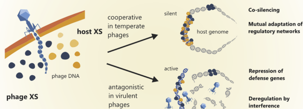
Fig. 3. Model for the functions of phage-encoded silencers depending on the phage lifestyle. Examples like the Lsr2-like silencer CgpS demonstrated that XS proteins may play an important role in maintaining the lysogenic state. Depending on the XS repertoire or the particular host strain, (pro-)phage-encoded XS proteins may also cooperate with the host-encoded protein(s) to form heteromeric complexes. The function of phage-encoded silencers has not been studied experimentally and therefore remains subject to speculation. Nevertheless, it can be postulated that virulent phages might employ XS-like proteins as a weapon to interfere with host defense systems or to repress other host defense mechanisms.
