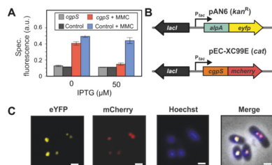
Figure 2. CgpS functions as a silencer of CGP3 prophage activity. (A) Silencing of CGP3 induction. The prophage reporter strain C. glutamicum ATCC 13032::P h3 -eYFP containing the cgpS overexpression plasmid pAN6-cgpS-Strep was cultivated in CGXII minimal medium in the presence or absence of IPTG (50 μM) and MMC (600 μM). The prophage reporter strain carrying the empty plasmid pAN6 served as a control. eYFP fluorescence was measured after 20 h of microplate cultivation. (B and C) CgpS is located in the nucleoid and displays colocalization with the phage adaptor protein AlpA (34). For co-localization studies, a C-terminal CgpS-mCherry fusion and a C-terminal fusion of the phage adaptor protein AlpA to eYFP (pEC-XC99E) were analyzed. Both gene fusions were under control of the inducible tac promoter. DNA was stained with Hoechst Dye 33342. Fluorescence images were taken after 2.5 h of cultivation in CGXII with 150 μM IPTG. Scale bar, 2 μm.
