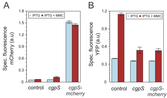
Figure S2: Silencing of CGP3 prophage induction. A and B. Phage reporter cells (WT::P lys-eyfp ) were transformed with pAN6, pAN6- cgpS and pAN6- cgpS-mcherry and were cultivated in CGXII with 50 \mu M IPTG and in the presence or absence of 0.6 \mu M MMC. The mCherry (A) and eYFP (B) fluorescence as well as backscattered light were measured in the BioLector® microcultivation system and were used to calculate the specific fluorescence. The specific fluorescence after 20 h of cultivation is shown. The data represent average values from three biological replicates including the standard deviation.
