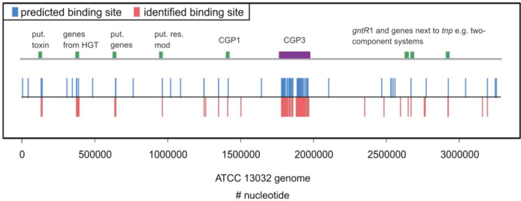
Figure S5: Comparison of predicted and experimentally identified CgpS binding sites. The DNA binding motif derived from ChAP-Seq results (Fig. 3C) was checked for further hits in the genome of ATCC 13032 using FIMO (14). Here, 90 positions exhibiting highest probability (p-Values: 2.7 \cdot 10^{-10} – 2.3 \cdot 10^{-6} ) (in blue) were compared with the 90 experimentally identified binding sites acquired by ChAP-Seq binding studies (in red). Potential CgpS site within the CGP3 region (purple boxes) and outside (green boxes) are highlighted. Correlation between experimentally identified and predicted CgpS binding sites ~75 %.
