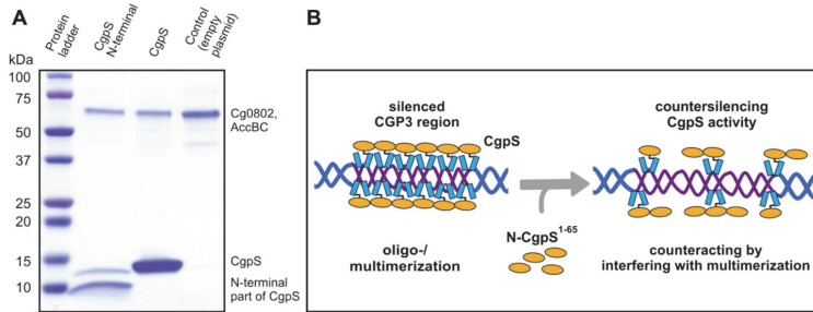
Figure 4. Principle of CgpS countersilencing. (A) Protein pull-down assays were conducted with C. glutamicum cells containing the plasmids pAN6-cgpS-Strep and pAN6-N-cgpS-Strep, which were used for the overexpression of Strep-tagged cgpS and its truncated variant. The pull-down of full-length CgpS by the truncated variant (aa 1–65) confirmed the N-terminal part of CgpS as oligo-/multimerization domain of CgpS proteins. (B) Model of CgpS silencing and countersilencing. The expression of genes depends on the accessibility of their particular promoter regions to the RNA polymerase. AT-rich regions such as CGP3 are bound by CgpS, likely resulting in an oligomerization of the CgpS protein (18,76,77), thereby interfering with the binding of RNA polymerase. The production of an N-terminal truncated CgpS variant interferes with the silencing ability of the native protein by binding to its N-terminal oligomerization domain while lacking the site for DNA binding.
