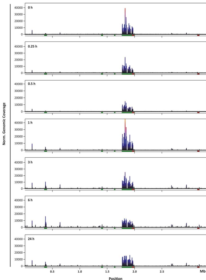
Figure 2: Normalized time series of CgpS binding in C. glutamicum under SOS-dependent prophage induction using ChAP-seq analysis. For these ChAP-seq analyses C. glutamicum ATCC 13032::cgpS-strep cells were grown in CGXII medium containing 2 % (w/v) glucose. The CGP3 prophage was induced by the addition of 600 nM mitomycin C. Samples were taken before (0 h) as well as 0.25 h, 0.5 h, 1 h, 3 h, 6 h and 24 h after induction with MMC. CgpS-bound DNA was purified and sequenced. The presented data were normalized with regard to the average coverage to enable comparisons between the different experiments (exemplarily shown in Figure S1). The coloring of the graphs represents the genomic coverage at a certain point and is split into 20 % sections in the following order (from lowest to highest values): black, blue, purple, red, orange. The green lines represent regions of low GC content and prophage regions (LGC1, CGP1-4), the dark red line represents a high GC region and the brown inclusion inside the big green CGP3 region marks the CGP4 area included in CGP3.
