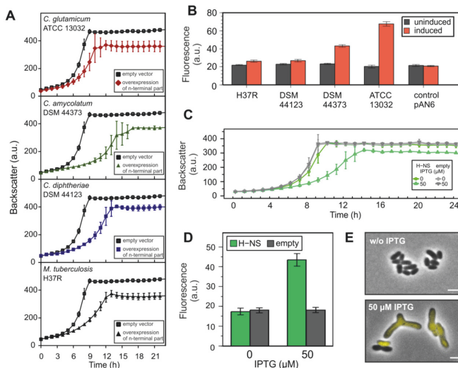
Figure 6. Impact of H-NS and Lsr2/Lsr2-like truncated variants on CgpS prophage induction. (A and B) Impact of truncated CgpS orthologs on the growth and CgpS prophage activity using the reporter strain ATCC 13032::P trc -cypn. Shown is the cultivation in microtiter plates in CGXII minimal media with 25 μg·ml -1 kanamycin and 150 μM IPTG. As a control the reporter strain containing the empty plasmid was used. In (B), the fluorescence output after 20 h is shown in comparison to the uninduced samples. (C and D) Growth experiments were performed with WT::PhyS-cypn cells carrying hns on the prophage reporter after 20 h is shown in (D). (E) After 24 h, fluorescence images were taken of cells (of C and D) placed on agar pads. Scale bar is 2 μm. Data represent average values and standard deviations of three biological replicates.
