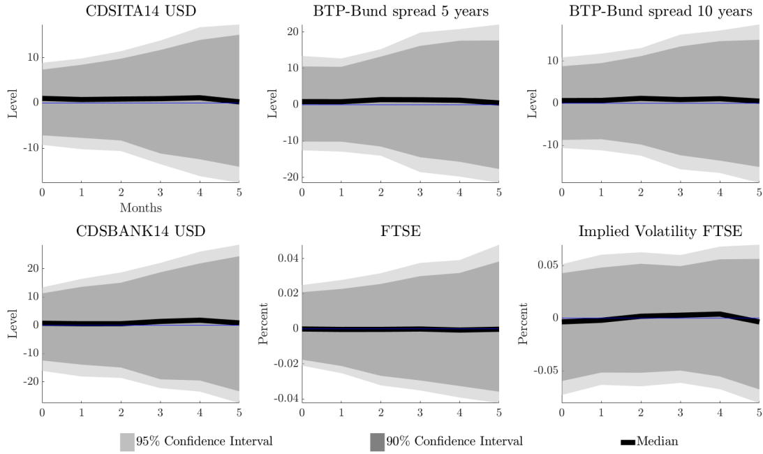
Figure 30: Financial variables: impulse responses at a monthly frequency; placebo
