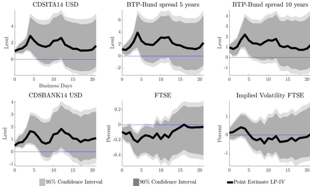
Figure 17: Financial variables: impulse responses at a daily frequency, excluding common EU dates
