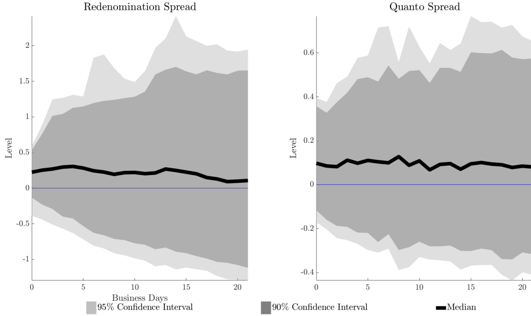
Figure 31: Redenomination spread and quanto spread: impulse responses and variance decomposition at a daily frequency; placebo
