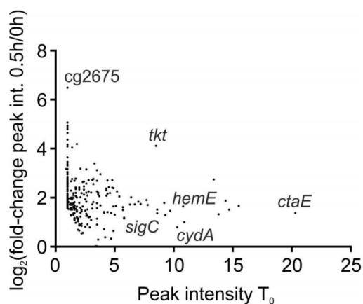
Figure S7: Dynamic range of HrrA association upon addition of external heme. ChAP-Seq analysis revealed that targets that are moderately bound before stimulus addition show a generally higher fold-change in HrrA association than targets sequences that showed already a high coverage at T_0 . The \log_2 of the fold change of the normalized peak intensities was calculated ( T_{0.5} versus T_0 ) and plotted against the peak intensity at time point T_0 (before stimulus addition). For details on cultivation and ChAP-Sequencing, see material and methods and Figure 1.
