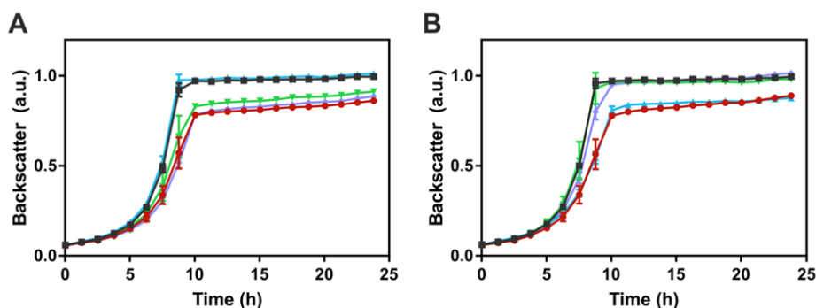
Fig. 5. Complementation of the growth defect of the C. glutamicum \Delta surf1 mutant with expression plasmids for genes encoding the Surf1 homologs of Corynebacterium diphtheriae (pAN6_CDC7B1688, blue triangles), Mycobacterium smegmatis (pAN6_MSMEG4311, green triangles), and Mycobacterium tuberculosis (pAN6_Rv2235, purple diamonds). The strains were cultivated in CGXII medium with 2% (w/v) glucose either in the absence of (A) or in the presence of 100 \mu M IPTG (B) at 30°C and 1200 rpm using a BioLector microcultivation system (m2p-labs, Aachen). As reference, C. glutamicum wt (black squares) and \Delta surf1 mutant (red circles), both carrying the pAN6 plasmid vector, were used. Growth was followed as backscatter at 620 nm and the maximal value obtained for the wt was set as 1. Mean values and standard deviation from three biological replicates are shown. a.u., arbitrary units.
