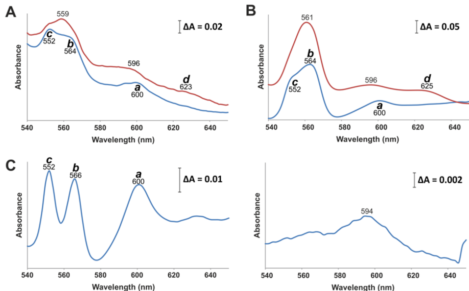
Fig. 3. Cytochrome spectra of the C. glutamicum wt and its \Delta surf1 mutant. (A) Dithionite-reduced spectra of intact cells. (B) Dithionite-reduced-minus-ferricyanide-oxidized difference spectra of membranes isolated from the C. glutamicum \Delta surf1 mutant (red) and the wt (blue). (C) Dithionite-reduced-minus-ferricyanide-oxidized difference spectra of the proteins purified by StrepTactin-affinity chromatography of CtaD St from strain \Delta ctaD/pJC1-ctaD_{St} (left) and from strain \Delta ctaD\Delta surf1/pJC1-ctaD_{St} (right). The absorption maxima of cytochrome c , cytochrome b , cytochrome a , and cytochrome d are depicted. Altered cytochrome peak maxima are indicated in the graphs. Cells were grown aerobically in BHI medium with 2% (w/v) glucose. All measurements were performed in 100 mM Tris/HCl (pH 7.5).
