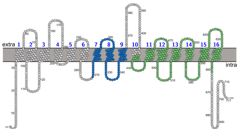
Figure 2. Topology model of the CtiP protein (Cg2699) created with the PROTTER software (72). The regions labeled in blue and green show sequence similarity to the CopD family (PFAM PF05425) and Caa3-CtaG family (PFAM PF09678), respectively.
