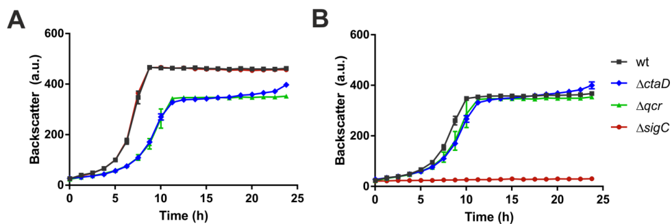
Figure S6.5.7. Growth properties of C. glutamicum deletion strains compared to the wt.
