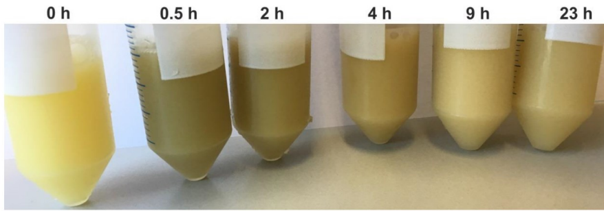
Figure S5: Visual inspection of C. glutamicum cells before and after addition of heme. Iron-starved C. glutamicum wild type cells were cultivated in CGXII medium (2 % (w/v) glucose, without \text{FeSO}_4 ) and cells were harvested at different time points before and after the addition of 4 \mu\text{M} heme. Cell pellets were subsequently resuspended in Tris-buffer (100 mM Tris-HCl, 1 mM EDTA, pH 8.0) and adjusted to an \text{OD}_{600} of 3.5.
