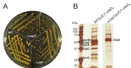
Figure 5. Properties of the \Delta\text{copC} mutant. A, C. glutamicum WT, the \Delta\text{copC} mutant, and the \Delta\text{ctiP} mutant were grown on a BHI agar plate for 2 days. B, solubilized membranes of the indicated strains were subjected to Strep-tactin affinity chromatography, and the eluates (10 \mu\text{g} ) were analyzed by SDS-PAGE and silver staining. The labeled proteins were identified by MS using protein bands from a Coomassie-stained gel performed in parallel.
