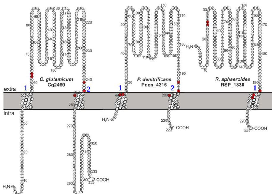
Fig. 1. Topology models of Surf1 proteins from C. glutamicum (Cg2460), P. denitrificans (Pden_4316) and R. sphaeroides (RSP_1830). Predictions of protein architectures were done using the PROTTER software [32]. Red shaded amino acid residues were shown to be involved in heme a binding in P. denitrificans Surf1 [18].
