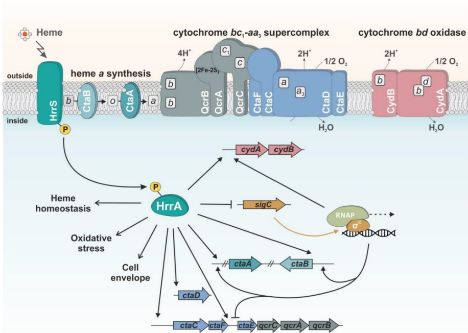
Figure 5: Model of heme-responsive control of components of the respiratory chain by HrrSA. The results of this study reveal HrrSA as a global regulator of heme homeostasis coordinating the expression of genes involved in heme biosynthesis, oxidative stress responses and cell envelope remodeling. An important part of the HrrA regulon is comprised by genes encoding the components of the branched respiratory chain of C. glutamicum . While HrrA acts as an activator of all components ( ctaE-qcrCAB , ctaA , ctaB , cydAB ), it represses transcription of the sigC gene encoding an important sigma factor required for cydAB expression. This regulatory network architecture consequently confers prioritization to the synthesis of the more efficient proton pump, the cytochrome bc 1 -aa 3 supercomplex. Bordered boxes, b, c, a, d: heme b, heme c, heme a, heme d.
