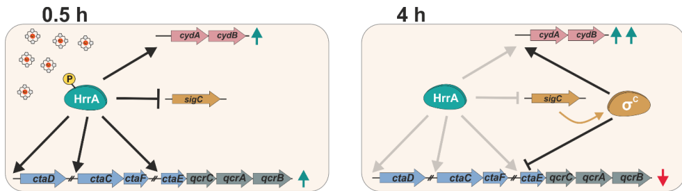
Figure 7: Working model of HrrSA-mediated respiratory chain gene regulation in response to heme under iron-limiting growth conditions. During the early growth phase (0.5 h after addition of 4 \mu M hemin) with an abundance of heme HrrA activates all genes encoding subunits of the cytochrome bc 1 -aa 3 branch ( ctaD , ctaCF , ctaE-qcrCAB ) and the cytochrome bd branch ( cydAB ) while repressing sigC expression. Decreasing heme concentrations (4 h after hemin addition) lead to derepression of sigC resulting in a further upregulation of the cyd genes and simultaneous repression of the ctaE-qcrCAB operon (modified from (Keppel et al. , 2019)).
