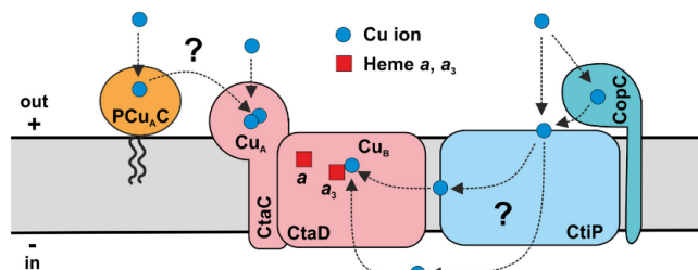
Figure 6. Model of the roles of CtiP (Cg2699), CopC (Cg1884), and PCu A C (Cg1883) in the biogenesis of cytochrome aa 3 oxidase in C. glutamicum . The CtiP protein is assumed to have a dual function in copper transport and copper transfer to the Cu B center of CtaD (subunit I). The absence of CtiP triggers the copper-deprivation response under copper excess. The CopC protein is a membrane-bound copper chaperone with a Cu(II)-binding motif that might donate copper to CtiP under copper deprivation. PCu A C is a secreted lipoprotein with a Cu(II)-binding motif that might be involved in the formation of the Cu A center. In contrast to the strains lacking CtiP or CopC, the mutant lacking PCu A C showed no growth defects under the conditions tested. Blue circles, copper ions; red squares, heme groups.
