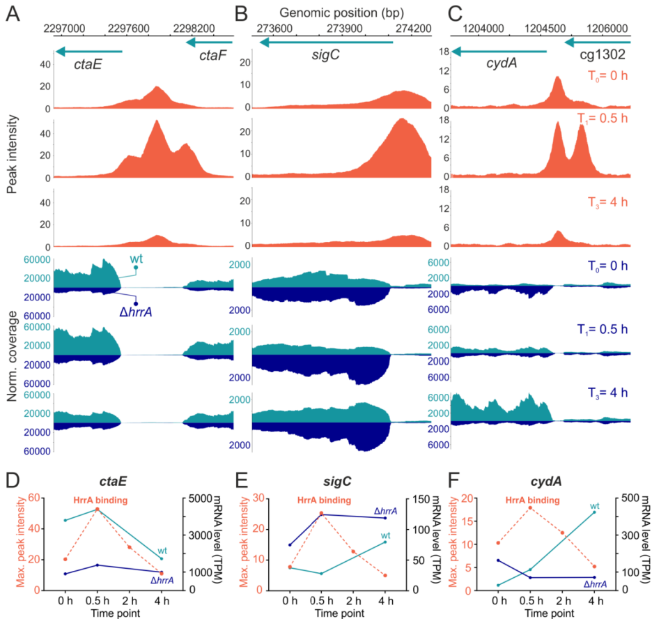
Figure 4: HrrA prioritizes the expression of genes encoding components of the bc 1 -aa 3 supercomplex. Depicted are HrrA binding peaks as identified by ChAP-Seq analysis (Figure 1 and 2) in comparison to the normalized coverage of RNA-Seq results (wild type and the \Delta hrrA mutant) for the genomic loci of ctaE (A, D), sigC (B, E) and cydA (C, F). D-F: HrrA binding (max. peak intensities measured by ChAP-Seq experiments) and the mRNA levels (in transcripts per million, TPM) of the respective genes in the \Delta hrrA strain as well as in wild type C. glutamicum cells 0, 0.5 and 4 h after the addition of hemin.
