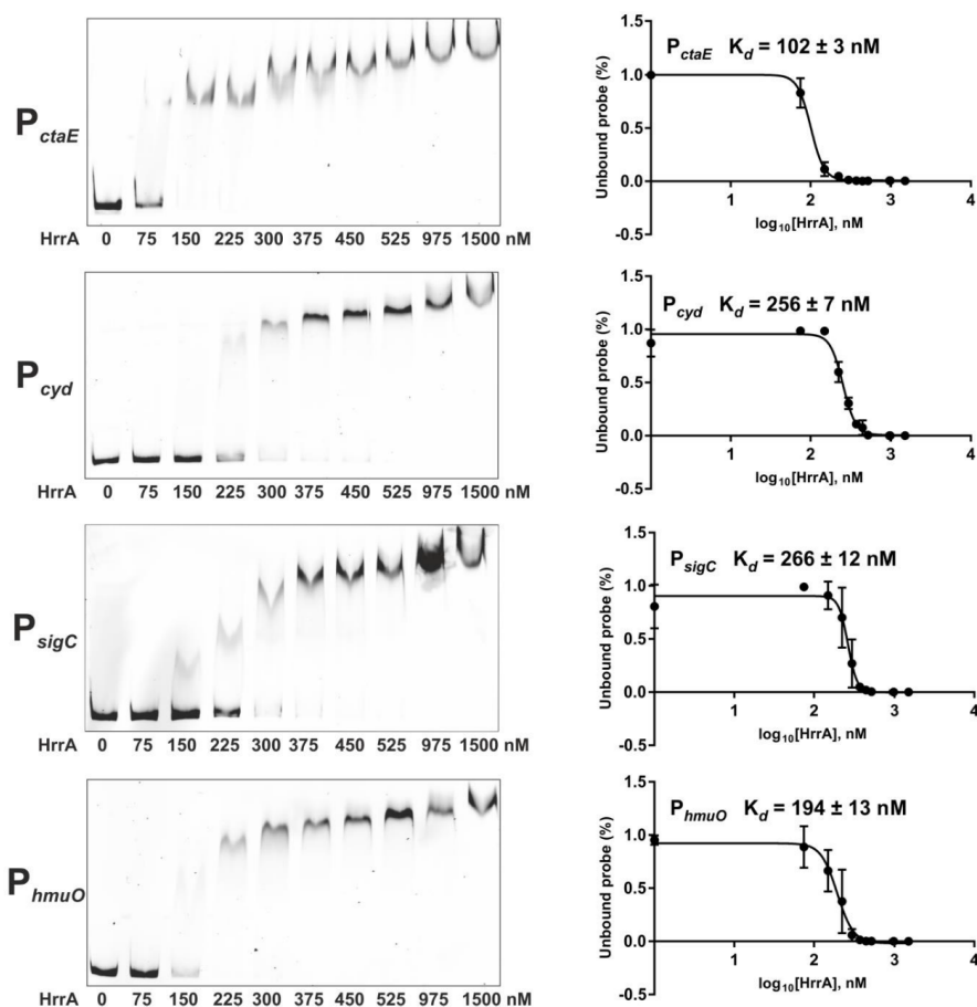
Figure S8: Binding affinity of HrrA to selected target promoters. Depicted are representative images of quantitative EMSAs used for analysis of protein-DNA interaction and the calculation of HrrA affinities to the different promoters. For the analyses, 15 nM DNA fragments covering 250 bp up- and downstream of the maximal ChAP-Seq peak height were used with an increasing monomeric protein concentration. Determination of unbound DNA in EMSA studies allowed the calculation of HrrA binding affinities to different target promoters. Quantification of unbound DNA band intensities was performed using AIDA v.4.15 (Raytest GmbH, Germany) and K_d values were calculated using GraphPad Prism 7.
