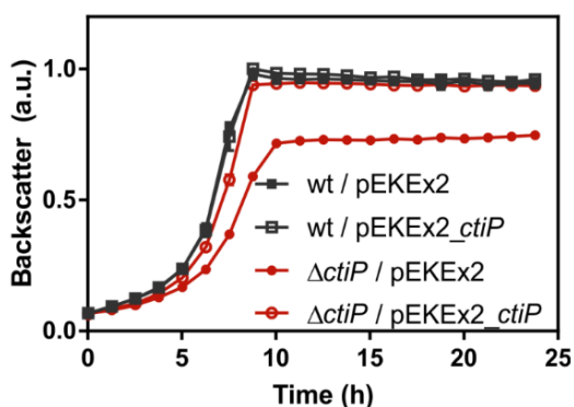
Figure S2. Complementation of the growth defect of the \Delta ctiP mutant by plasmid-based expression of ctiP using plasmid pEKEEx2_ ctiP carrying ctiP under control of the P_{tac} promoter. The strains were cultivated in CGXII medium with 4% (w/v) glucose supplemented with 25 \mu g ml -1 kanamycin in a Biolector microcultivation system. Growth was followed online as backscatter at 620 nm. All backscatter values were normalized by setting the maximal backscatter value of the WT/pEKEEx2 culture as 1. Mean values and standard deviations of three biological replicates are shown.
