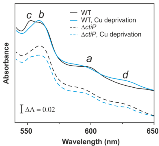
Figure S1. Dithionite-reduced spectra of C. glutamicum WT cells and \Delta cgt2699 mutant cells cultivated either in standard CGXII medium or in copper-deprived CGXII medium. Cytochromes c , b , a and d are indicated at the wavelengths 552 nm, 562 nm, 600 nm and 630 nm, respectively.
