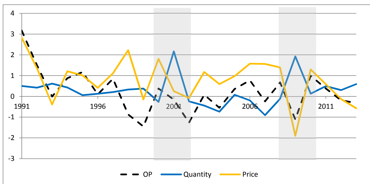
Figure 7: Components of OP term (percentage points)
