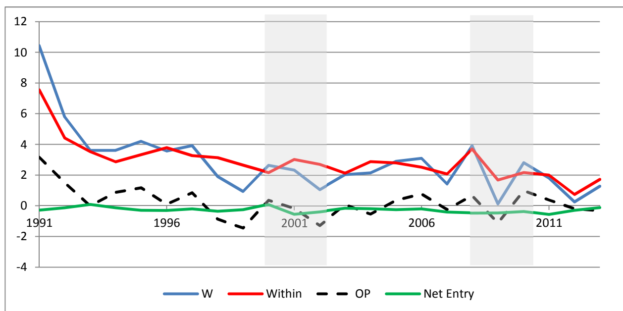
Figure 6: dynamic OP decomposition (percentage points)
