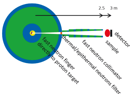
Fig. 4.2. Schematic view of the neutron source NOVA ERA with the instrument for in-beam fast neutron imaging
