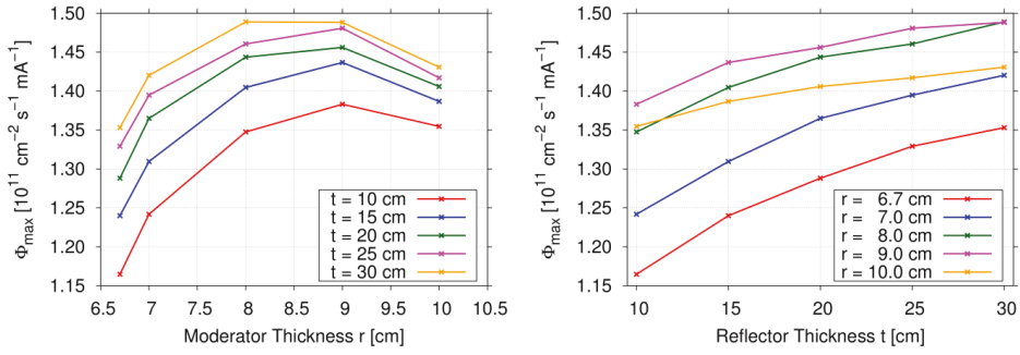
Fig. 3.10. Dependence of the maximum thermal neutron flux on the polyethylene moderator thickness for different thicknesses of the lead reflector (left). Dependence of the maximum thermal neutron flux on the lead reflector thickness for different thicknesses of the polyethylene moderator (right)
