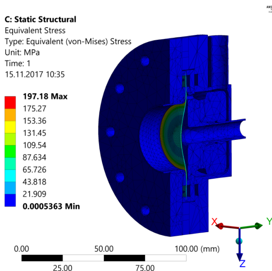
Fig. 3.8. Mechanical deformation and von-Mises-stress for the beryllium target. The colours show the equivalent stress in MPa, while the deformation is visually exaggerated by a factor of 50. The true deformation has a maximum value of 0.14 mm in the centre of the target disc. Local stress maxima are found in the centre of the disc, with values around 140 MPa. At the boundary between the supported and the unsupported area of the beryllium disc the stress is 197 MPa.
