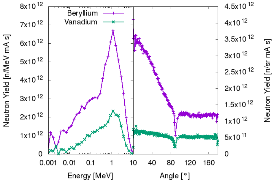
Fig. 3.4. Primary neutrons' energy spectra obtained for the interaction of 10 MeV protons with beryllium and vanadium (left) and corresponding angular distributions for a proton beam of 30 mm diameter (right)
