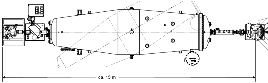
Fig. 3.2. Dimensions of a 5 MV tandem accelerator with ion source, chopper, and switching magnet as offered by High Voltage Engineering B.V. [18]
