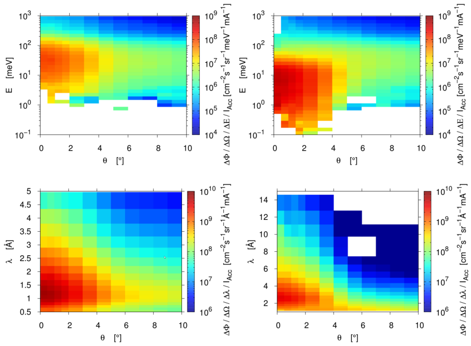
Fig. 3.15. Brilliance delivered by the thermal neutron channel T2 (left) and the cold neutron channel C2 (right) at surface of the lead reflector (see Fig. 3.12 for corresponding beam-line configuration). Note the different wavelength scale for the two cases. The beryllium target is used for the production of fast neutrons.
