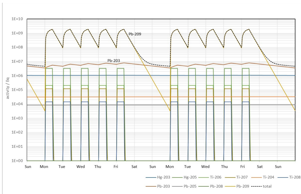
Fig. A6.10. Activity of the radionuclides formed by neutron activation in the lead reflector ( m = 1,000 kg) at week 39 and 40 out of 40 weeks of irradiation with 10 h of irradiation per working day and 5 working days per week (in total 2,000 h of irradiation)
