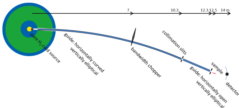
Fig. 4.4. Schematic view of the neutron source NOVA ERA with the instrument for neutron reflectometry
