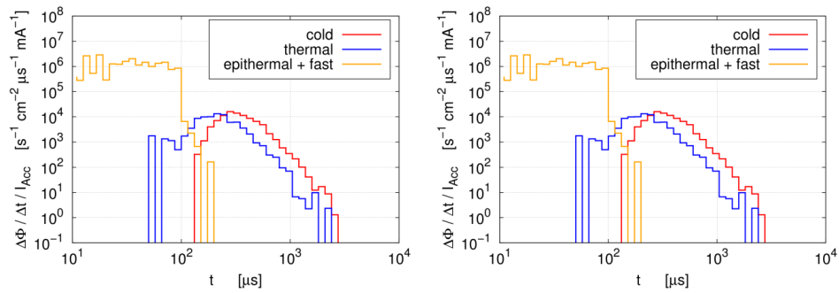
Fig. A3.4. The time structure of fast, thermal and cold neutron pulses delivered by the fast neutron channel F1 (left) and the cold neutrons channel C4 with liquid parahydrogen as cold moderator (right) (see Fig. 3.12 for corresponding beam-line configuration). The beryllium target is used for production of fast neutrons. The length of the proton pulse is \mu\text{s} .
