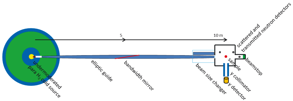
Fig. 4.1. Schematic view of the neutron source NOVA ERA with the instrument for prompt and delayed gamma neutron activation analysis with neutron time-of-flight (TOF-P&DGNA)
