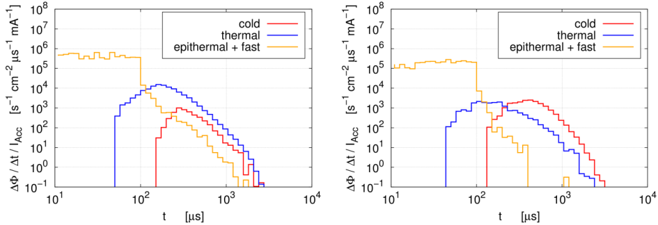
Fig. A3.2. The time structure of fast, thermal and cold neutron pulses delivered by the thermal neutron channel T2 (left) and the cold neutrons channel C2 with liquid parahydrogen as cold moderator (right) (see Fig. 3.12 for corresponding beam-line configuration). The beryllium target is used for production of fast neutrons. The length of the proton pulse is 100 \mu s.
