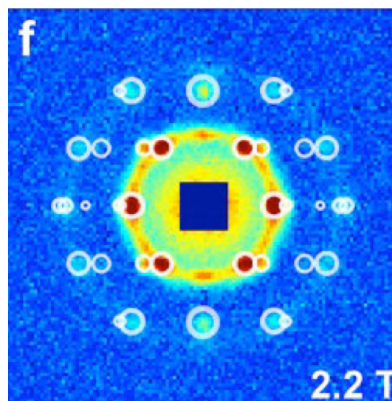
Fig. 2.2. SANS patterns of an iron oxide particle solution [9]
