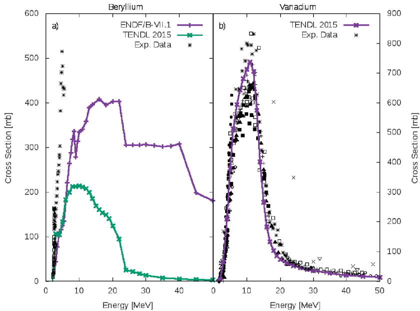
Fig. 3.3. Proton energy dependence of the microscopic cross section for the reactions a) {}^9\text{Be}(p,n){}^9\text{B} and b) {}^{51}\text{V}(p,n){}^{51}\text{Cr} . The theoretical data are taken from the ENDF/B-VII.1F [19] and TENDL 2015 [20] databases. The symbols represent experimental data.
