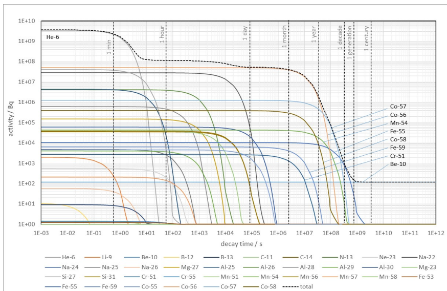
Fig. A6.1. Decay of the radionuclides formed by proton and neutron activation in the beryllium target ( m = 6.5 g) during 2,000 h of operation without interruption
