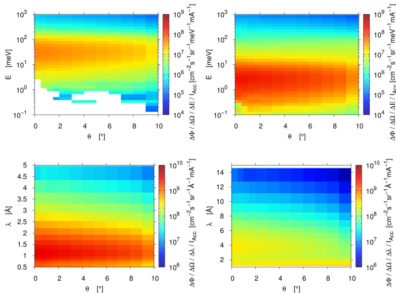
Fig. A4.3. Brilliance delivered by the thermal neutron channel T3 (left) and the cold neutron channel C3 with solid methane as cold moderator (right) (see Fig. 3.12 for corresponding beam-line configuration). The beryllium target is used for the production of fast neutrons.
