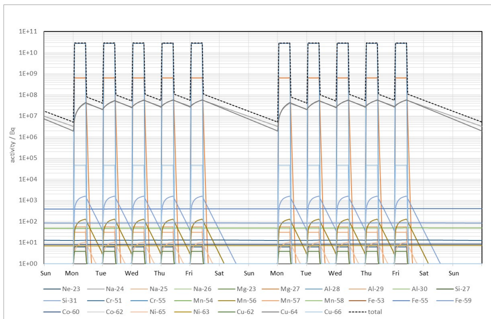
Fig. A6.6. Activity of the radionuclides formed by neutron activation in the aluminum mounting ( m = 1,100 g) at week 39 and 40 out of 40 weeks of irradiation with 10 h of irradiation per working day and 5 working days per week (in total 2000 h of irradiation)
