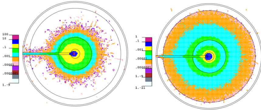
Fig. 3.20. Neutron (left) and gamma (right) dose rate distributions calculated by using MCNP6 for a shielding made of 30 cm borated polyethylene surrounded with 10 cm lead. The unit of the colour legend is 10 mSv/h/source-particle.
