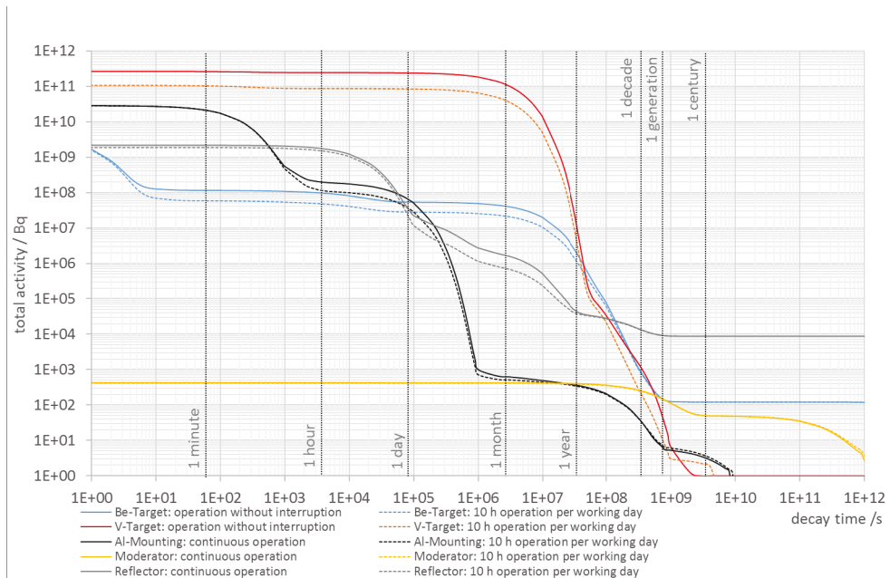
Fig. 7.1. Decay of the total activity induced by irradiation of the beryllium target, the vanadium target and the aluminium mounting for two operation scenarios of the neutron source. Elemental composition of the materials and neutron activation fluxes are given in Table 7.1.
