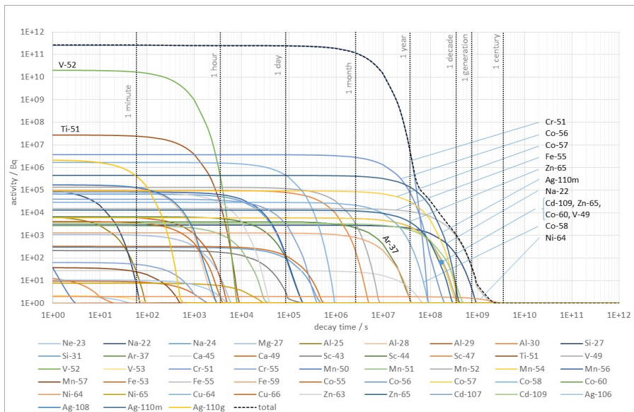
Fig. A6.3. Decay of the radionuclides formed by proton and neutron activation in the vanadium target ( m = 61.4 g) during 2,000 h of operation without interruption
