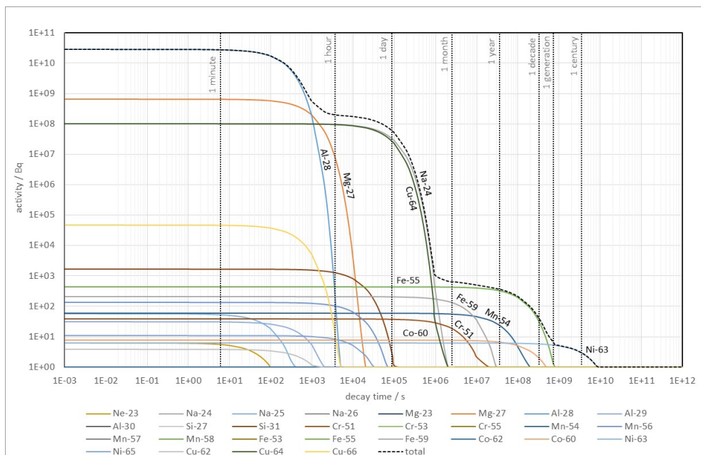
Fig. A6.5. Decay of the radionuclides formed by neutron activation in the aluminum mounting ( m = 1,100 g) during 2,000 h of operation without interruption
