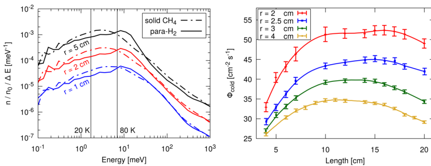
Fig. 3.16. Spectra of neutrons leaving a cylindrical parahydrogen or solid methane cold moderator at 20 K for three different radii (left). The lengths of the cylinders are 4, 5, and 6 cm for parahydrogen and 2, 2.5, and 5 cm for solid methane. The maximum shifts not only with the material, but also with the spin state, since the main low energy scattering mechanism is an induced spin flip. Emitted brilliance at the moderator surface (right). While the total neutron flux is decreasing with the radius (see left diagram), the brilliance is enhanced up to a factor of 2.
