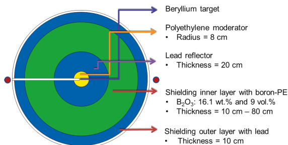
Fig. 3.19. Simplified model of the neutron source for calculation of neutron and gamma dose rates using MCNP 6. A horizontal cut through the target is shown. The proportions of the moderator reflector assembly and the components of the biological shielding are not respected for better visualization. The red surfaces represent the point detectors.
