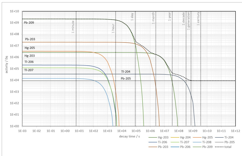
Fig. A6.9. Decay of the radionuclides formed by neutron activation in the lead reflector ( m = 1,000 kg) during 2,000 h of operation without interruption
