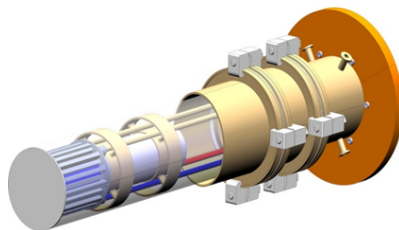
Fig. 3.18. Cold moderator vessel with cryogenic supply and monitoring (left). Technical drawing of the moderator vessel (left). The total length of the vessel is 600 mm.
