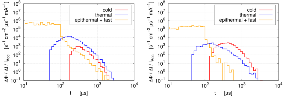
Fig. A3.1. The time structure of fast, thermal and cold neutron pulses delivered by the thermal neutron channel T1 (left) and the cold neutrons channel C1 with solid methane as cold moderator (right) (see Fig. 3.12 for corresponding beam-line configuration). The beryllium target is used for production of fast neutrons. The length of the proton pulse is 100 \mu s.
