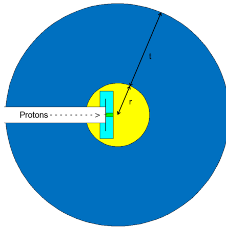
Fig. 3.9. MCNP model of the moderator-reflector assembly including the proton beam-line and the beryllium target. The radius of the polyethylen moderator is r . The thickness of the lead reflector is t . Components displayed are the target (black), the target mounting (cyan), the target coolant (green), the polyethylene moderator (yellow) and the lead reflector (blue). A horizontal cut through the target is shown.
