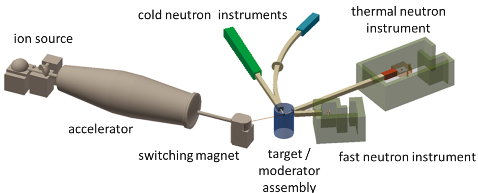
Fig. 1.1. Artistic view of NOVA ERA with four beam-lines and instruments
