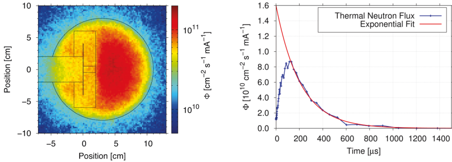
Fig. 3.11. Distribution of the thermal neutron flux inside polyethylene moderator and lead reflector at the middle plane of the beryllium target irradiated with 10 MeV protons (left). Time structure of the thermal neutron flux inside a finite volume at the location of highest neutron flux obtained for a proton pulse of 100 \mu\text{s} (right). The energy range for the thermal neutrons is 13 to 127 meV.
