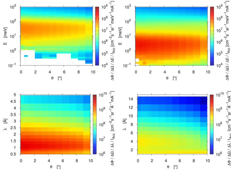
Fig. A4.1. Brilliance delivered by the thermal neutron channel T1 (left) and the cold neutron channel C1 with solid methane as cold moderator (right) at surface of lead reflector (see Fig. 3.12 for corresponding beam-line configuration). The beryllium target is used for the production of fast neutrons.
