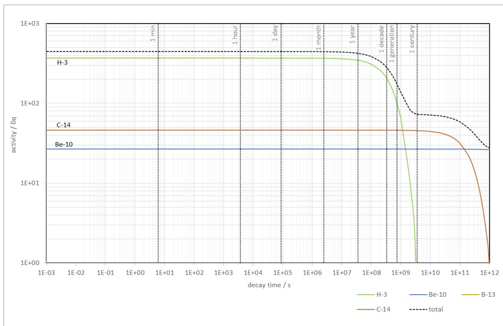
Fig. A6.7. Decay of the radionuclides formed by neutron activation in the polyethylene moderator ( m = 1,300 g) during 2,000 h of operation without interruption
