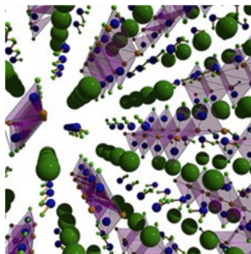
Fig. 2.1. Crystal structure solution of \text{KMg}(\text{ND})(\text{ND}_2) : An ordered mixed amide/imide compound [8]
