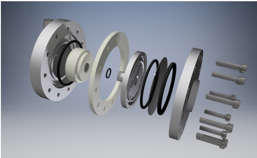
Fig. 3.6. Explosion view showing the components of the target assembly
