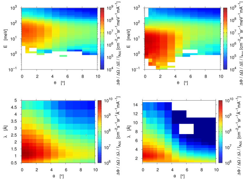
Fig. A4.2. Brilliance delivered by the thermal neutron channel T2 (left) and the cold neutron channel C2 with liquid parahydrogen as cold moderator (right) (see Fig. 3.12 for corresponding beam-line configuration). The beryllium target is used for the production of fast neutrons.
