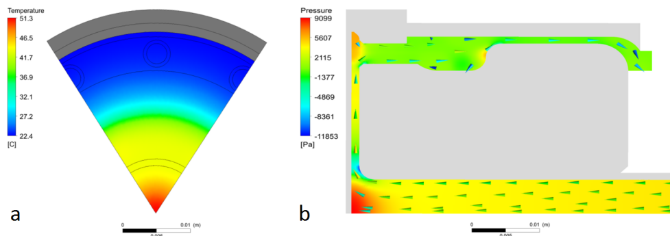
Fig. 3.7. a) Temperature at the beryllium surface on the vacuum side. b) Kinetic pressure component of the water. The arrows indicate the velocity vector of the coolant. For the CFD simulations, a water inlet temperature of 22°C was assumed with an inlet velocity of 3 m/s.
