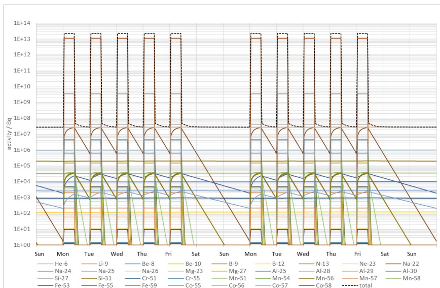
Fig. A6.2. Activity of the radionuclides formed by proton and neutron activation in the beryllium target ( m = 6.5 g) at week 39 and 40 out of 40 weeks of irradiation with 10 h of irradiation per working day and 5 working days per week (in total 2,000 h of irradiation)
