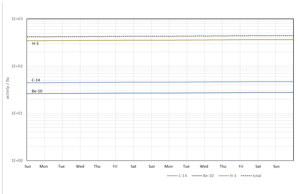
Fig. A6.8. Activity of the radionuclides formed by neutron activation in the polyethylene moderator ( m = 1,300 g) at week 39 and 40 out of 40 weeks of irradiation with 10 h of irradiation per working day and 5 working days per week (in total 2,000 h of irradiation)
