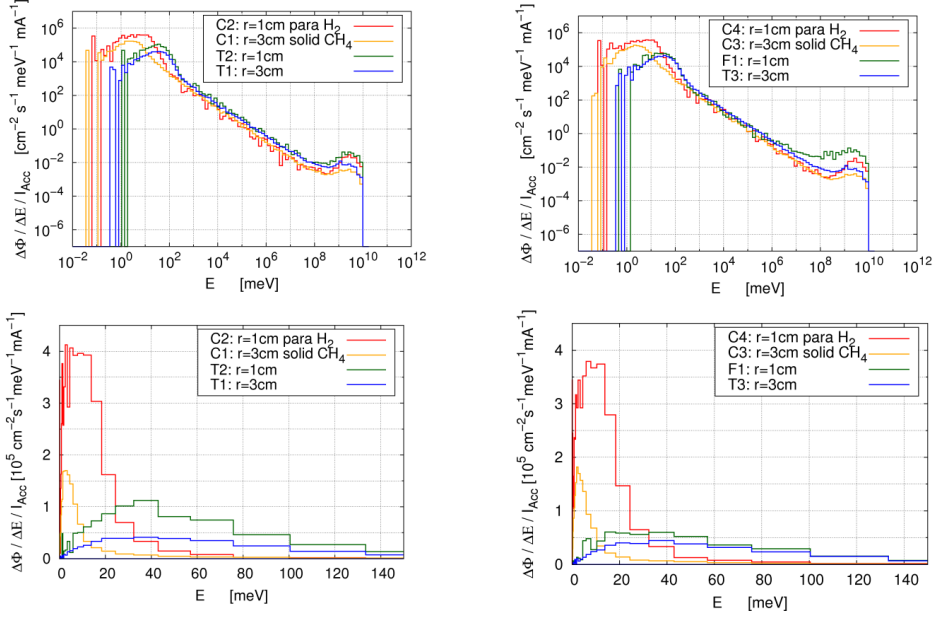
Fig. 3.13. Neutron energy spectra obtained for the neutron channels of the two beam-line configurations shown in figure 3.12. The beryllium target is used for production of fast neutrons.
