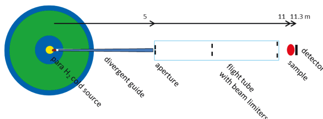
Fig. 4.3. Schematic view of the neutron source NOVA ERA with the instrument for in-beam cold and thermal neutron imaging with time-of-flight resolution of the neutron wavelengths
