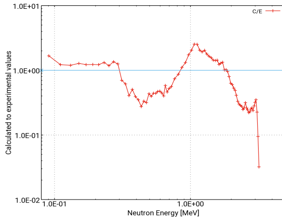
Fig. A1.2. Ratio of calculated to experimental neutron spectrum for the ^9\text{Be}(p,n) reaction with 5 MeV protons. The bin widths are 20 keV up to neutron energy of 700 keV and are 50 keV otherwise. The energy at the centre of the bins is provided.
