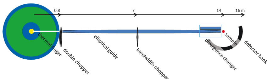
Fig. 4.6. Schematic view of the neutron source NOVA ERA with the instrument for neutron powder diffraction
