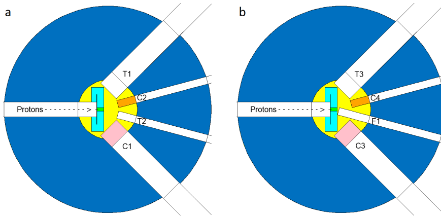
Fig. 3.12. MCNP model of the neutron source. a) Configuration with two channels for thermal neutrons (channels T1 and T2) and two channels for cold neutrons using either solid methane (channel C1) or parahydrogen (channel C2) as cold moderator. b) Configuration with one channel for thermal neutrons (T3), one channel for fast neutrons (F1) and two channels for cold neutrons (channel C3 with solid methane and channel C4 with parahydrogen). Components displayed are the target (black), the target mounting (cyan), the target coolant (green), the polyethylene moderator (yellow), the lead reflector (blue), solid methane (pink) and parahydrogen (orange). A horizontal cut through the target is shown.
