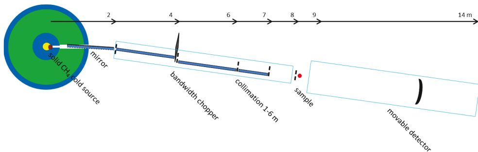
Fig. 4.5. Schematic view of the neutron source NOVA ERA with the instrument for small angle neutron scattering
