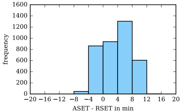
Figure 6.4: ASET-RSET difference map distribution.
