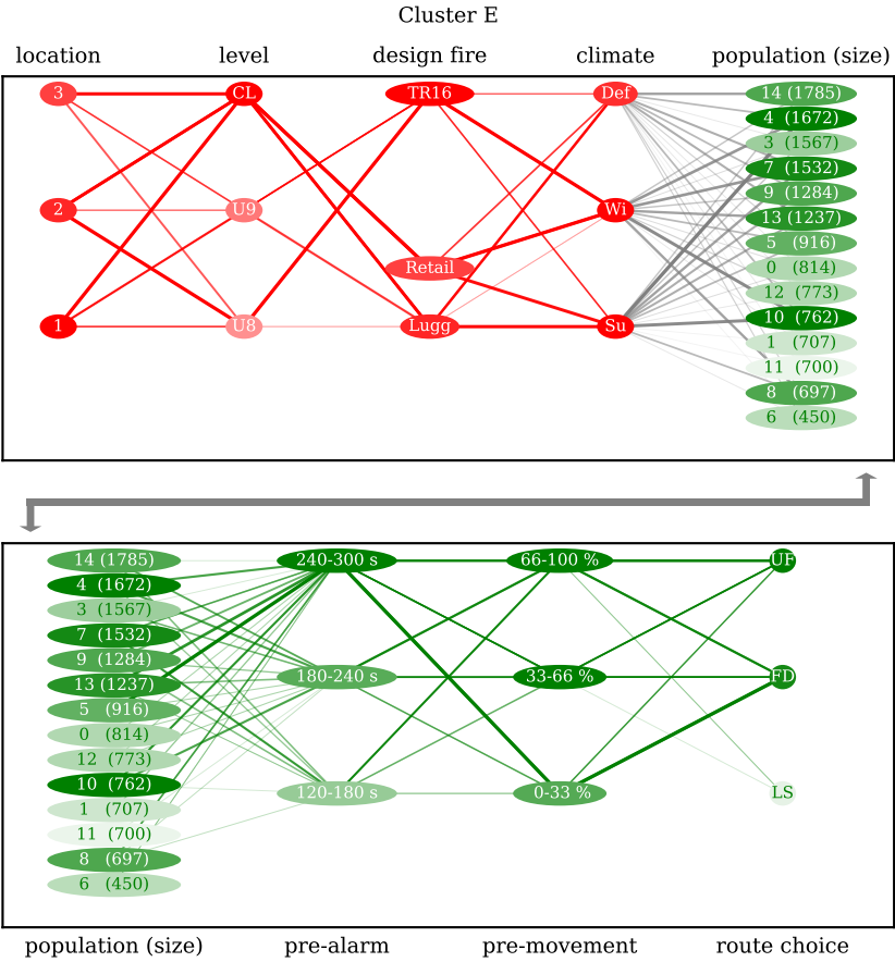
Figure C.8: Parallel coordinate plot illustrating the parametric relations of cluster E.
