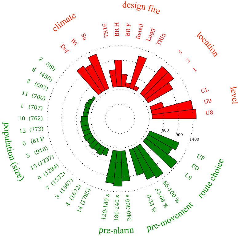
Figure 6.12: Radar plot illustrating the parametric origin of cluster B.
