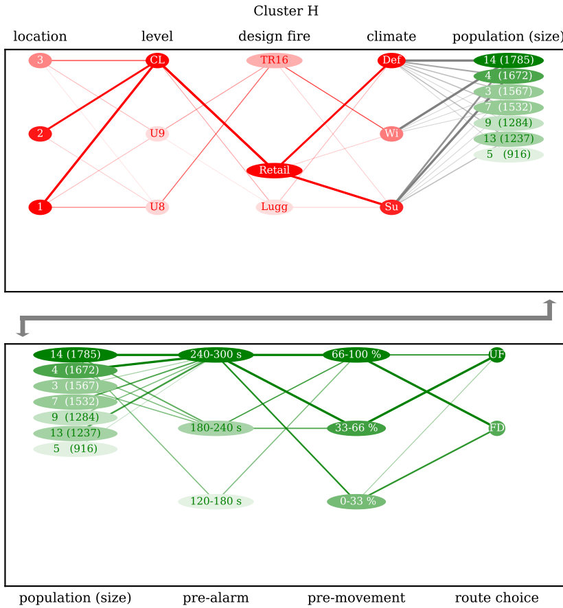
Figure C.14: Parallel coordinate plot illustrating the parametric relations of cluster H.
