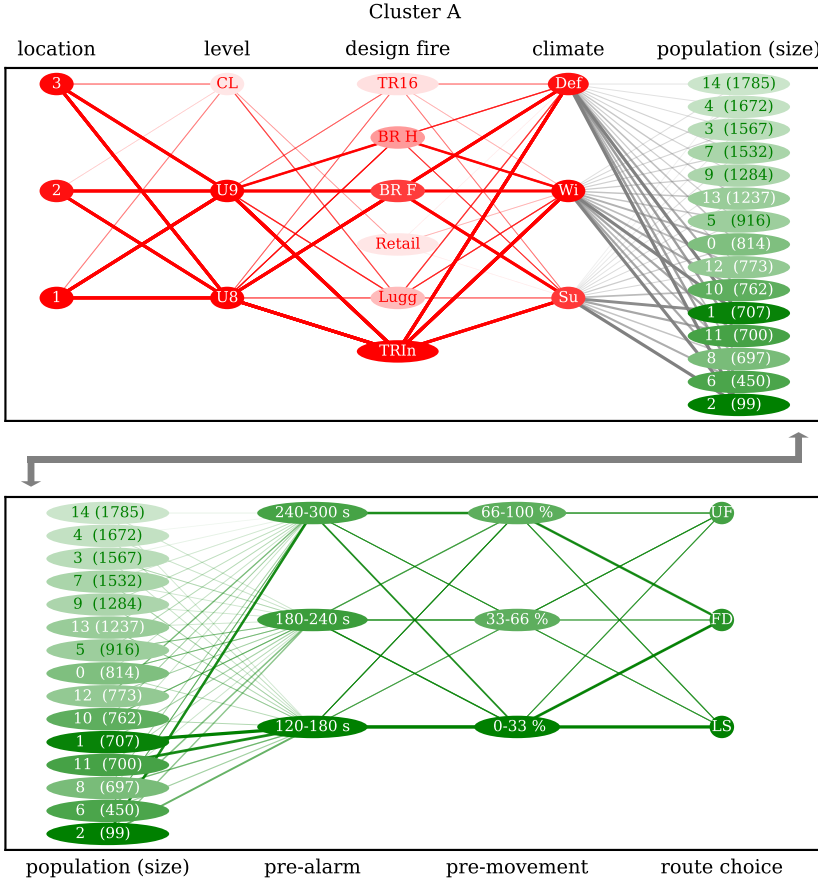
Figure 6.11: Parallel coordinate plot illustrating the parametric relations of cluster A.
