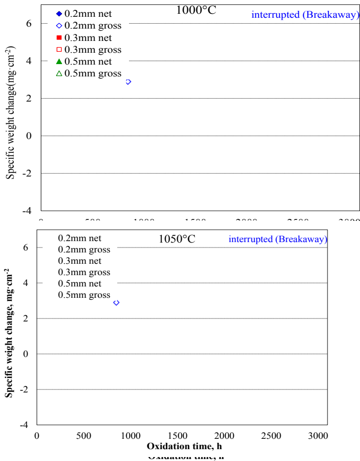
Figure 5.1. Typical example of net and gross weight change of alloy 230 (with specified specimen thicknesses) during oxidation in laboratory air at 1000 and 1050°C. The open and closed symbols indicate the total and specimen mass changes, respectively.
