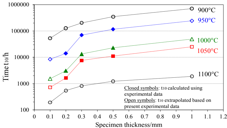
Figure 6.18: Calculated times t_{10} as function of specimen thickness for alloy 230 with extrapolations (open symbols) to other temperatures and specimen thicknesses based on experimental results of specimens oxidized at studied temperatures. See text for details used in the calculation.
