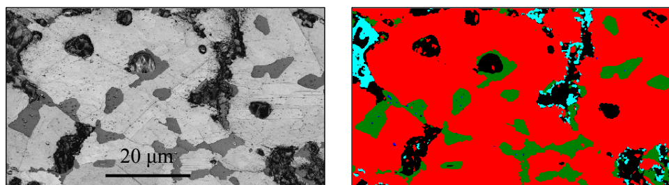
Figure 8.12: EBSD phase mapping in the center of the 0.2 mm alloy X specimen after oxidation of 3000 h at 1000°C (compare Figure 8.6 d ).
