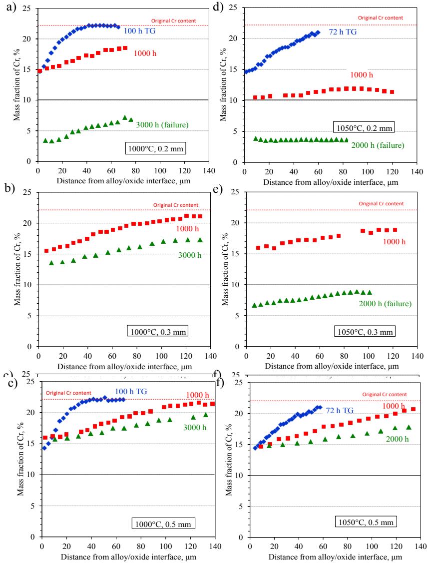
Figure 8.16: Concentration profiles of Cr in \gamma -Ni matrix (measured by EDX) of alloy X specimens of different thicknesses after different times of air oxidation at a-c) 1000°C and d-f) 1050°C.
