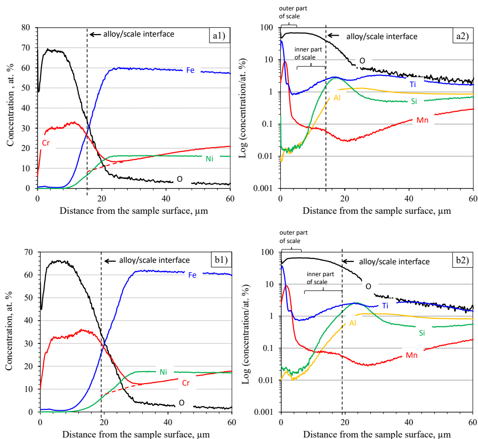
Figure 10.16: GDOES profiles of the a) 0.2 mm and b) 0.5 mm specimens of Nicrofer 2020 after 72 h isothermal TG test in synthetic air at 1050°C.
