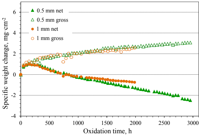
Figure 6.19: Comparison of net and gross weight changes of 0.5 and 1 mm specimens of alloy 230 during oxidation at 1050°C.
