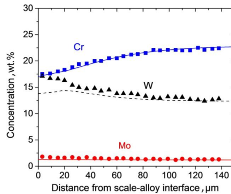
Figure 5.16: Cr, W and Mo concentration profiles in the \gamma\text{-Ni} matrix measured by EDX (symbols) in the 0.3 mm thick specimen of alloy 230 compared with DICTRA calculations (lines) after 1000 h oxidation at 1000°C in laboratory air. Measured oxidation kinetics used as input for the calculation was taken from the gravimetric data in Figure 5.1 .
