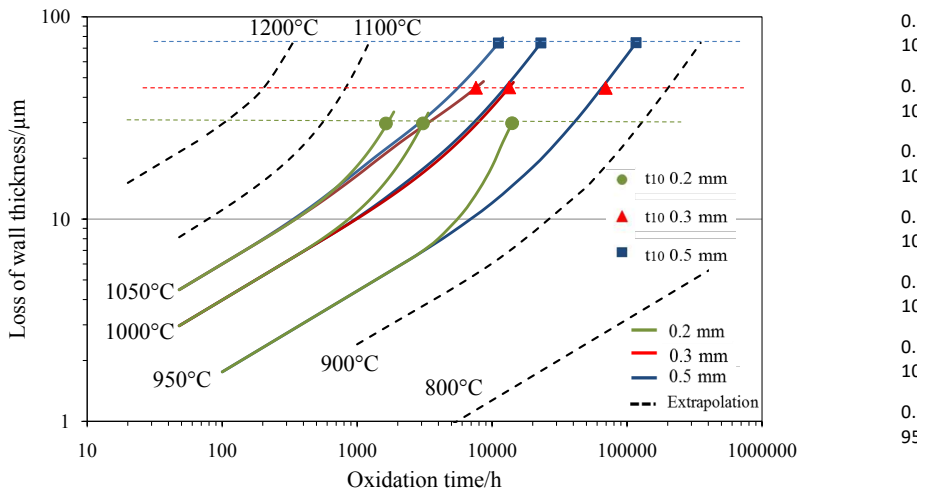
Figure 6.16: Lifetime diagram of alloy 230 showing data from Figure 6.15 (solid lines) and extrapolations to other temperatures (dashed lines), using procedures described in text.
