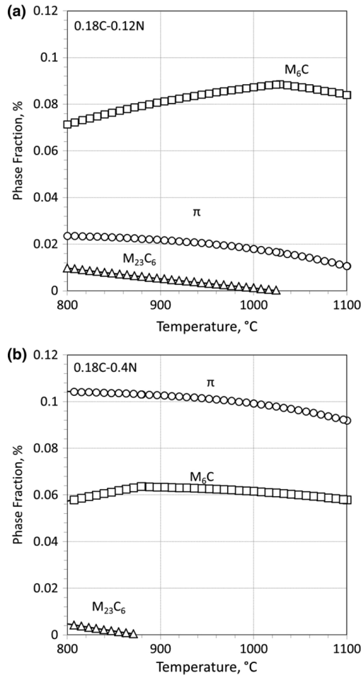
Figure 5.18: Calculated phase fractions in alloy 230 as function of temperature for various C and N contents. For details, see text.
