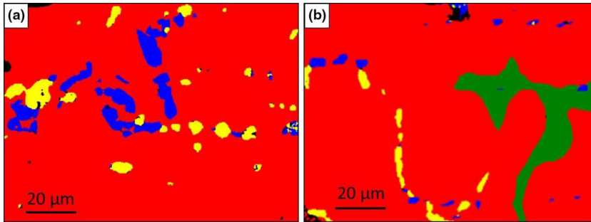
Figure 5.7: EBSD phase maps for Alloy 230 in two different places (a, b) in the center of 0.3 mm specimen of alloy 230 after 3000 h oxidation at 1000°C in laboratory air. In the EBSD phase map red color corresponds to \gamma -Ni matrix, yellow to M_{23}C_6 , blue to M_6C and green to \pi - Ni_2W_3N . The location used for the measurement in Fig. a) corresponds to the left side of Figure 5.5 ; the location used for the measurement in Fig. b) corresponds to the right side of Figure 5.5 .
