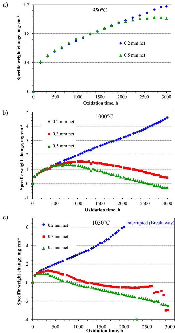
Figure 6.2: Area specific net weight change curves of alloy 230 specimens with different thicknesses during oxidation for 3000 h at a) 950°C (10 h cycle), b) 1000°C (48 h cycle), and c) 1050°C (48 h cycle).
