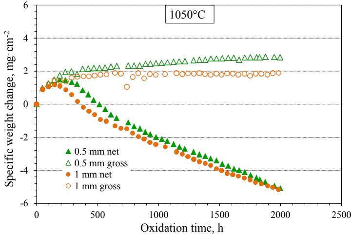
Figure 8.2: Comparison of weight change data of 1 mm and 0.5 mm specimens of alloy X during oxidation at 1050°C in air.
