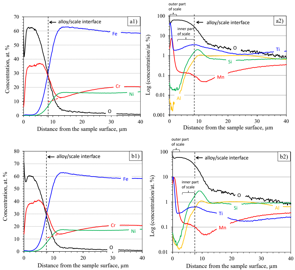
Figure 10.15: GDOES profiles of the a) 0.2 mm and b) 0.5 mm specimens of Nicrofer 2020 after 72 h isothermal TG test in synthetic air at 900°C.
