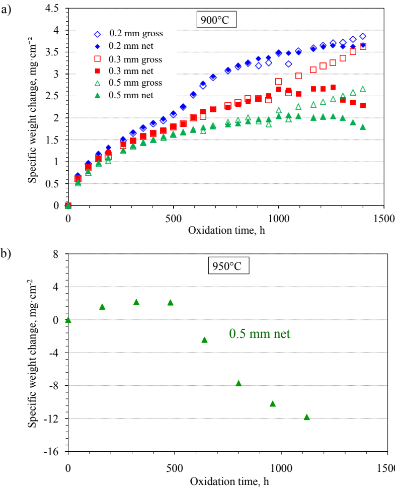
Figure 10.1: Oxidation kinetics of Nicrofer 2020 specimens with different thicknesses at a) 900, b) 950, and c) 1000°C.
