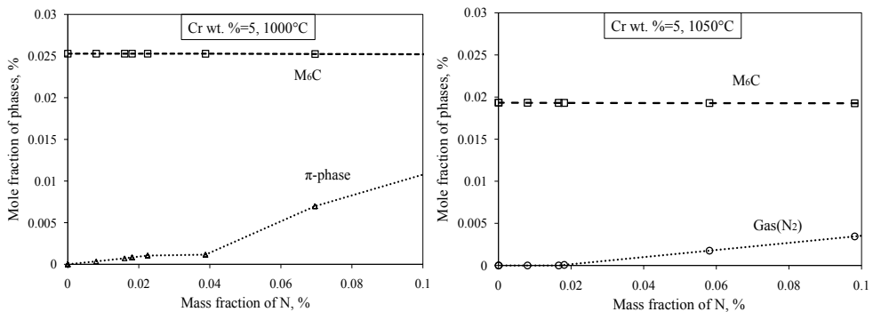
Figure 8.18: Mole fractions of stable phases (in addition to \gamma\text{-Ni} ) at 1000°C and 1050°C in alloy X, however with a Cr concentration of 5 wt. % calculated in Thermo-Calc using the TTNI7 database.
