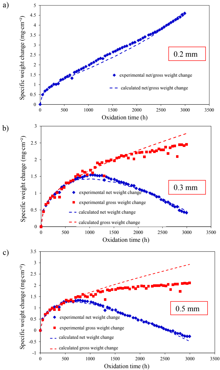
Figure 6.14: Comparison between experimental (symbols) and calculated (dashed lines) area specific net and gross weight change curves of alloy 230 for specimens of a) 0.2 mm b) 0.3 mm and c) 0.5 mm thickness here showing the results of the 1000°C experiments as examples.
