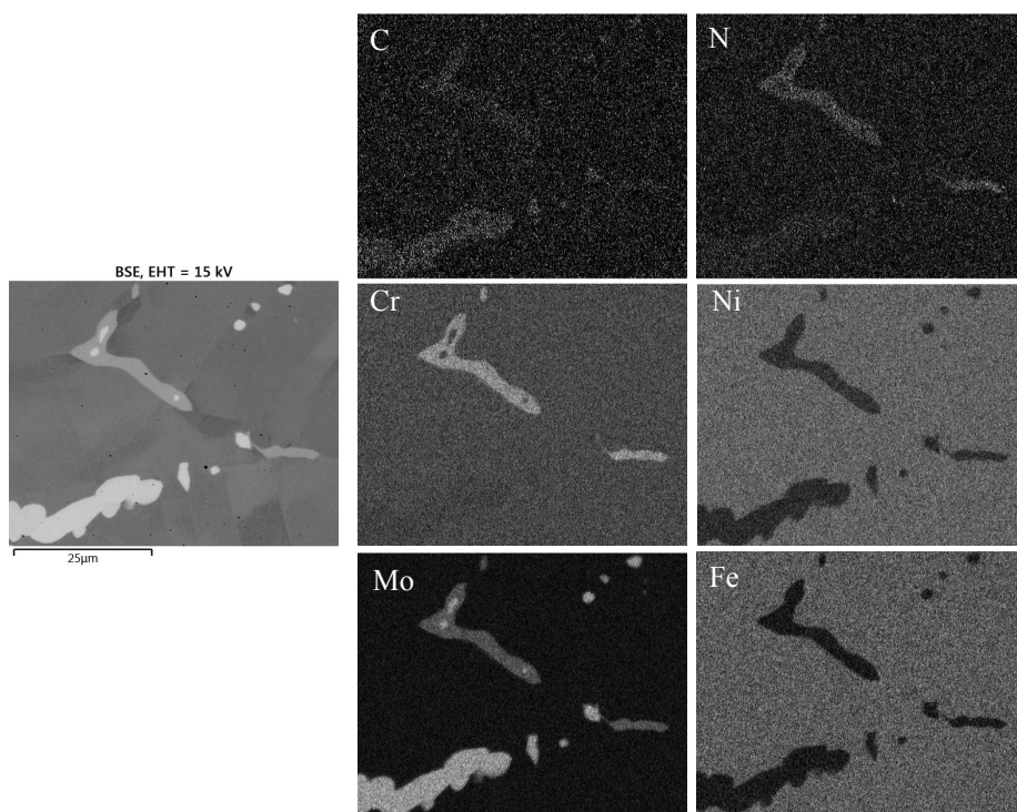
Figure 8.8: BSE image (left) and EDX element mappings in the center of the 0.3 mm specimen of alloy X after 3000 h oxidation at 1000°C (compare Figure 8.6 e ).
