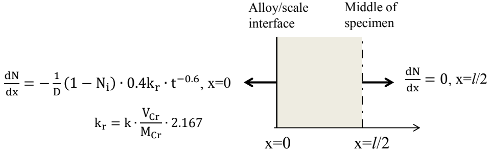
Figure 7.2: Schematic illustration of boundary conditions for Cr flux, i.e. (D \frac{dN}{dx}) used in steady-state FDM. ( l is the thickness of the specimen)
