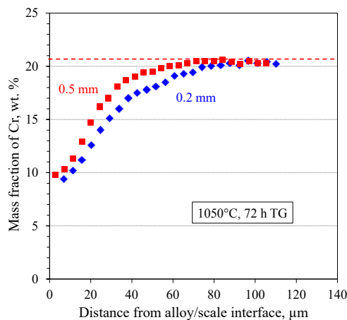
Figure 10.14: Subscale concentration profiles of Cr in Nicrofer 2020 specimens of different thicknesses isothermally oxidized at 1050°C for 72 h in TG test.
