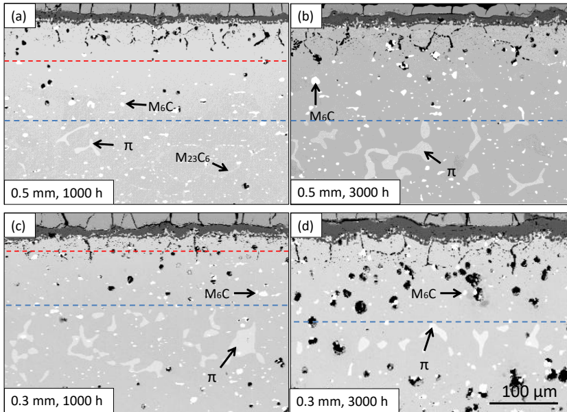
Figure 5.11: BSE images of a, b) 0.5 mm, c, d) 0.3 mm after reaction for a, c) 1000 h and b, d) 3000 h in laboratory air at 1050°C (blue and red dashed lines indicate the width of the zones depleted in M_6C and Cr-rich precipitates, respectively).
