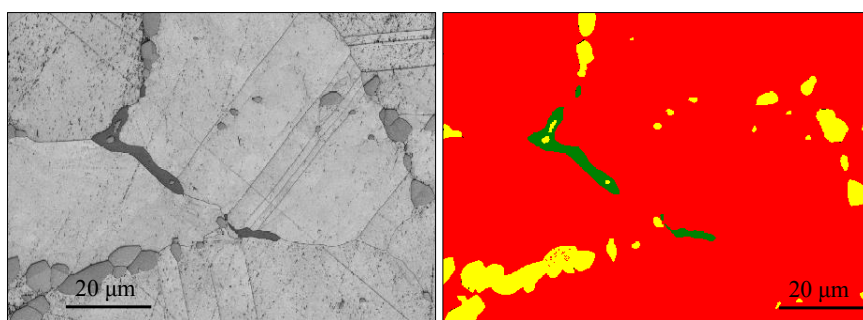
Figure 8.8: BSE image (left) and EDX element mappings in the center of the 0.3 mm specimen of alloy X after 3000 h oxidation at 1000°C (compare Figure 8.6 e ).
