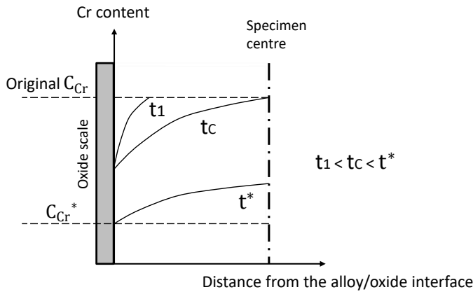
Figure 6.1: Schematic graph showing concentration profiles of scale forming element after different oxidation times in case of steady state scale growth illustrating difference in definition of times to critical subscale depletion ( t_c and t^* ).
