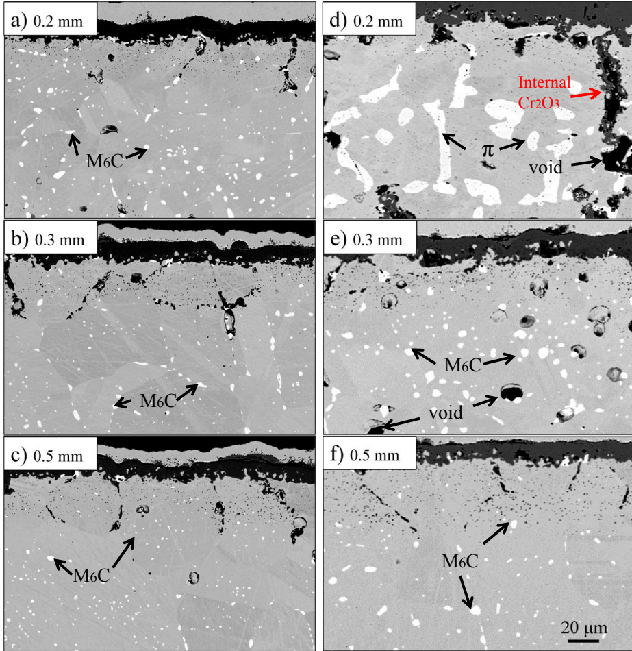
Figure 8.6: BSE cross section images showing the specimen thickness dependent microstructure of alloy X specimens after a-c) 1000 h and d-f) 3000 h oxidation at 1000°C.
