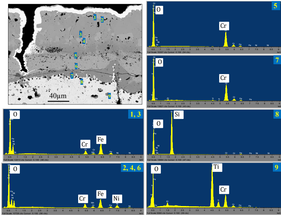
Figure 10.8: BSE image showing cross section of 0.5 mm thick specimen of Nicrofer 2020 after oxidation at 1000°C for 1560 h with spectrums of EDX point analyses, corresponding to the specimen shown in Figure 10.6 f .
