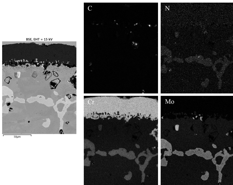
Figure 8.11: BSE image (left) and EDX element mappings in the center of the 0.2 mm alloy X specimen after 3000 h oxidation at 1000°C (compare Figure 8.7 d ).
