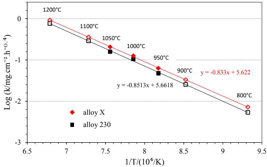
Figure 8.21: Comparison of rate constant of oxidation k (assuming power law kinetics, i.e. Eq. (3.19) with n=0.4 ) during steady state oxidation for alloy X and alloy 230. Closed symbols are derived from experimental data; open symbols are extrapolated values.
