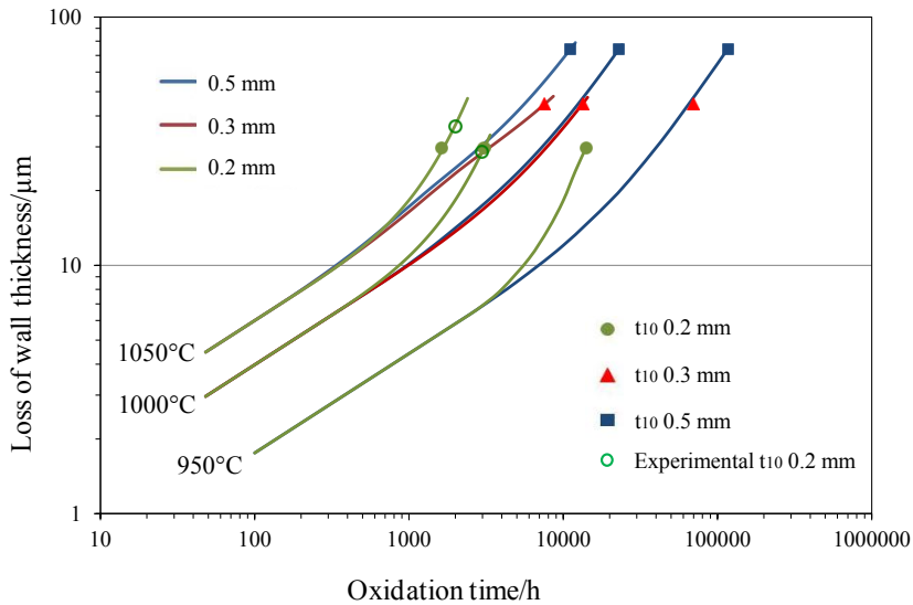
Figure 6.15: Lifetime diagram of alloy 230 showing calculated total loss of wall thickness as function of time at different temperatures. Calculations are based on assumption that wall thickness loss occurs on both specimen sides in the same manner. Inserted are solid symbols indicating times t_{10} for specimens of different thickness (0.2, 0.3 and 0.5 mm). Open symbols indicate experimentally observed times close to t_{10} .
