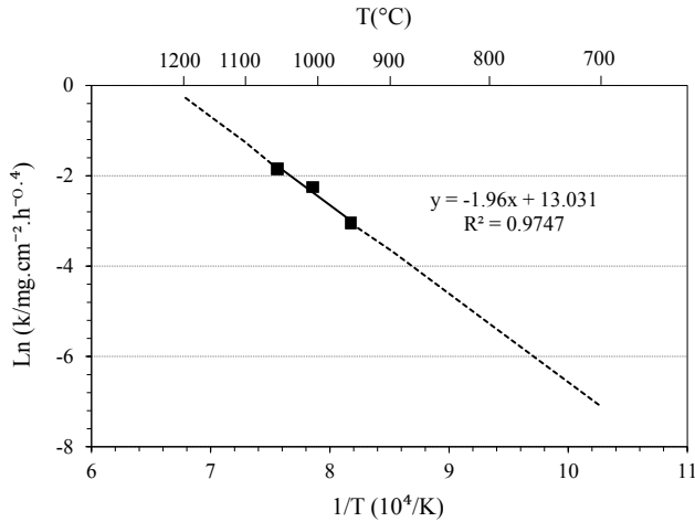
Figure 6.12: Rate constant k (Eq. (6.2)) during steady state oxide growth for alloy 230. Symbols indicate measured data, dashed line indicates extrapolation assuming an Arrhenius relationship (Eq. (6.3)).
