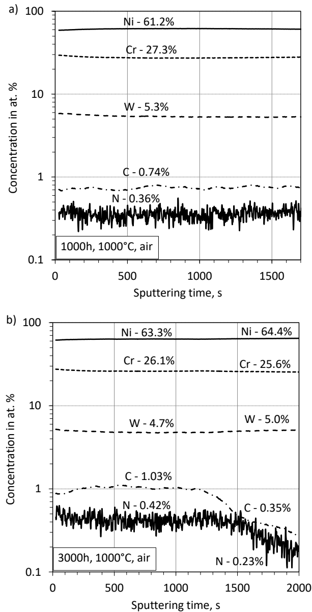
Figure 5.15: Element concentrations as function of sputter time for 0.5 mm alloy 230 specimen after 1000 and 3000 h exposure at 1000°C. Before the GDOES measurement, the specimens were ground to half thickness. Thus, the left part of the diagram (sputter time equals 0 s) corresponds to the center of the specimen. Averaged concentrations of the various elements in the respective regions are inserted in the graphs.
