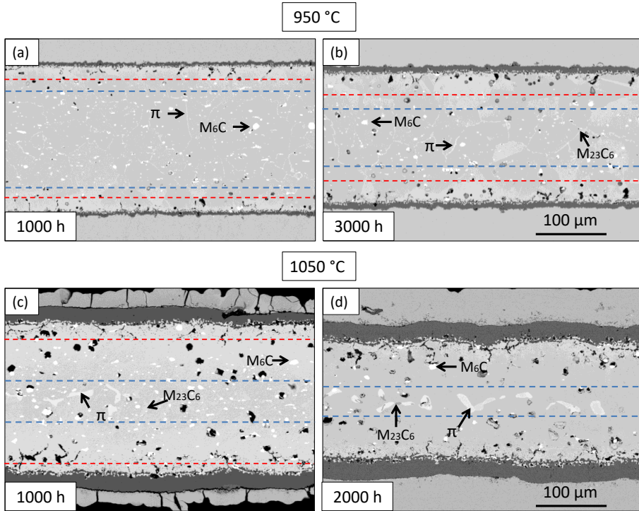
Figure 5.9: BSE images of 0.2 mm thick alloy 230 specimens after reaction for a) 1000 h and b) 3000 h at 950°C h and c) 1000 h and d) 2000 h at 1050°C in laboratory air (Blue and red dashed lines indicate the width of the zones free of M_6C and Cr-rich precipitates respectively)
