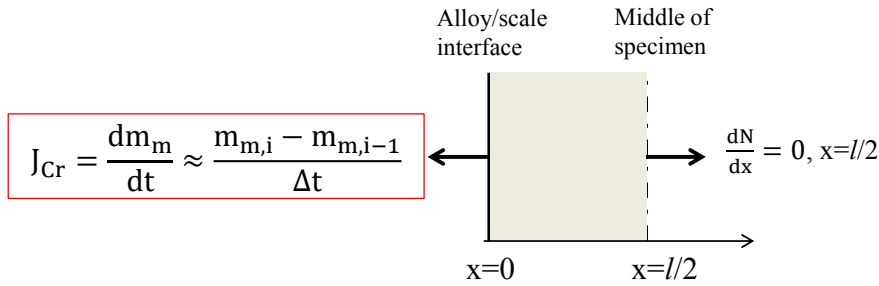
Figure 7.5: Schematic illustration of boundary conditions for Cr flux used in FDM for non-steady-state oxidation conditions. ( l : thickness of specimen)
