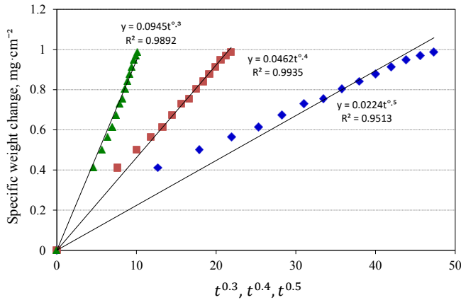
Figure 6.10: Fitting of the specific net weight change data of 0.5 mm alloy 230 specimen oxidized at 950°C to t^n .
