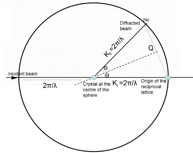
Figure 2.7: Ewald construction
