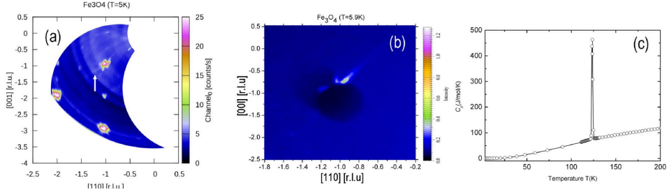
Figure 4.15: (a) Neutron Diffuse neutron scattering in( hhl ) plane at 5 K (b) Diffuse scattering by high energy X-rays in ( hhl ) plane at 6 K. (c) Specific heat, C_p of the crystal measured at zero magnetic field ( T_V=123\text{ K} ).
