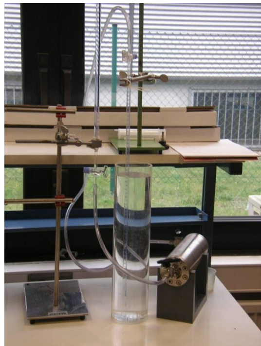
Fig. 3.23 System for measurement of sand/bentonite permeability to gas (left) and water (right)
