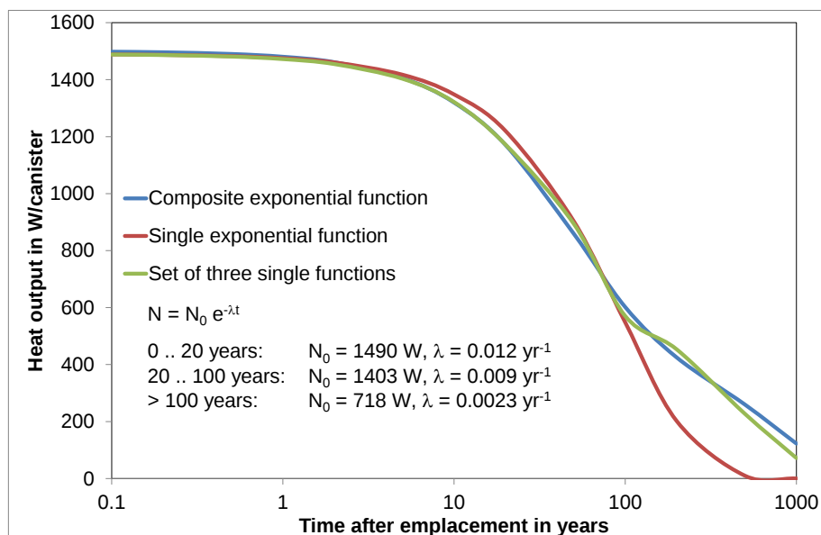
Fig. 5.14 Approximations of canister heat decay curve: The set of three single functions was used for the GRS simulation
