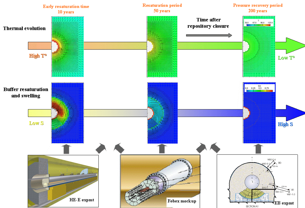
Fig. 1.1 Concept of the validation experiments in the project PEBS
