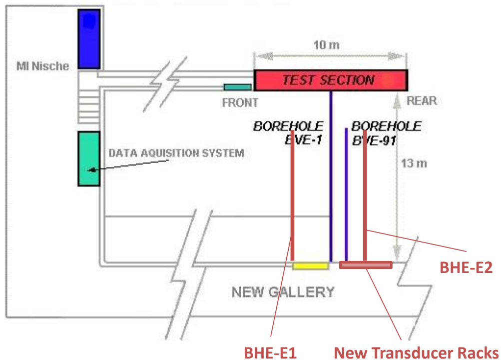
Fig. 4.9 Plan view showing the locations of the old VE boreholes BVE-1 and BVE-91 and of the additional packer boreholes BHE-E1 and BHE-E2
