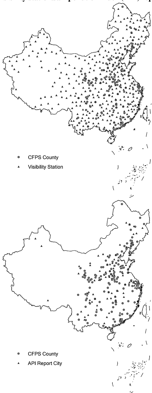
Figure 2.1—Distribution of China Family Panel Studies (CFPS) counties and visibility stations/air pollution index (API) report cities
