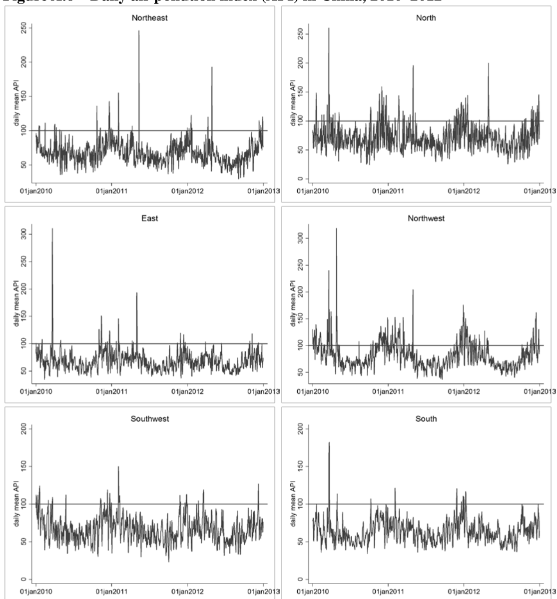
Figure A.6—Daily air pollution index (API) in China, 2010–2012
