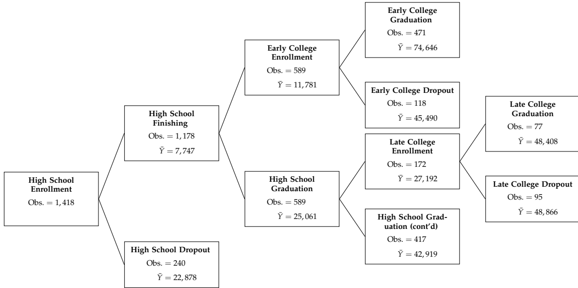
Figure 1: Decision Tree
