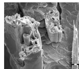
SEM micrograph: fracture surface of kenaf fibre reinforced PLA
