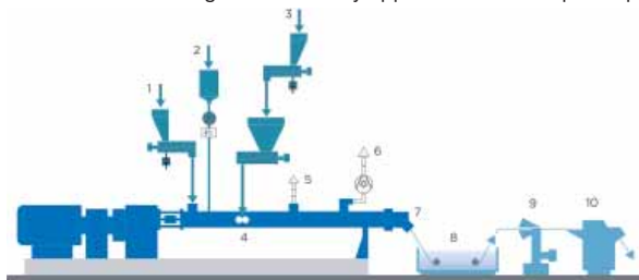
Typical plant structure for the production of biodegradable products
