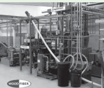
Compounding plant for the production of WPC Wood Plastic Composites.
